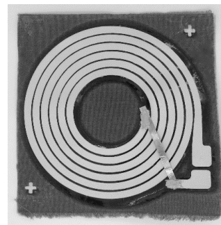
Figure 2: Printed coil, outer diameter 138 mm
