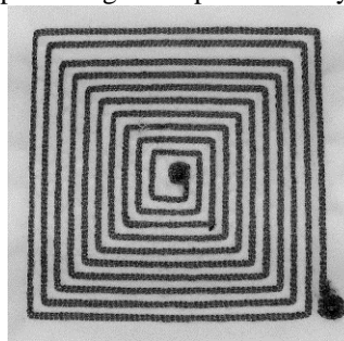
Figure 4: Square-single sided sewn coils, Light Stitches conductive thread, outer diameter 87 mm.
