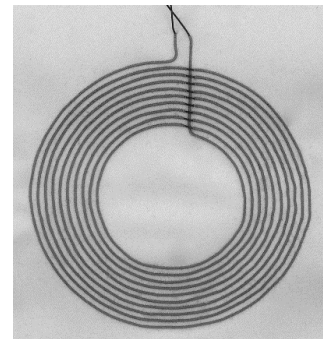
Figure 5: Circular sewn on coils, PTFE stranded wire, outer diameter 90 mm.
