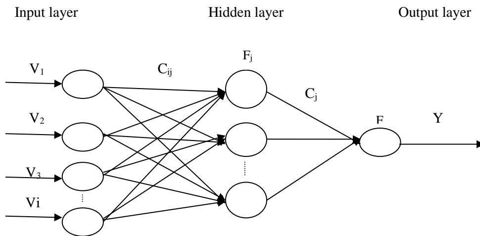
Figure 2: MLP Feed-Forward NN Architecture (one hidden layer)
