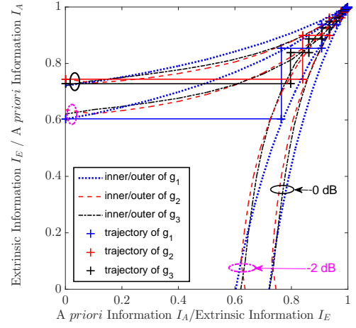
Fig. 6. EXIT chart for the GPs of g_1(D) = 1 + D^2 + D^5 (blue), g_2(D) = 1 + D + D^2 + D^4 + D^5 (red) and g_3(D) = 1 + D + D^3 + D^4 + D^{13} (black) over Nakagami channels, when m_l = 3.0 at SNR = -2 dB and SNR = 0 dB.
