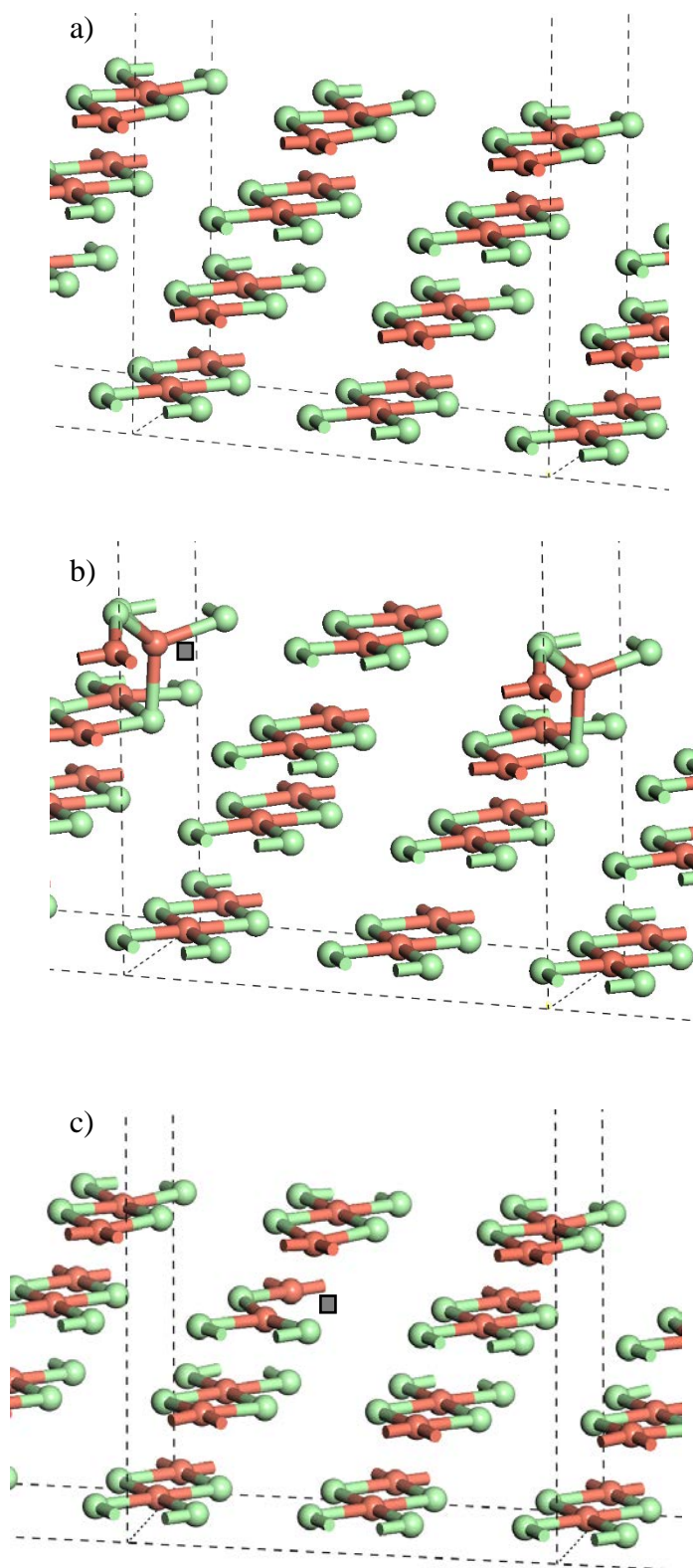
Figure 7. a ) Slab model of stoichiometric CuCl 2 (010) surface. b ) Structure with Cl - vacancy in surface layer of slab and c ) structure with Cl - vacancy in second layer of slab. Note that the position of the anion vacancy is indicated by a grey square in b ) and c ). All structures optimised with PBE+U using U=7 and Grimme D2 dispersion included. Atoms coloured Cu: pink, Cl : green.
