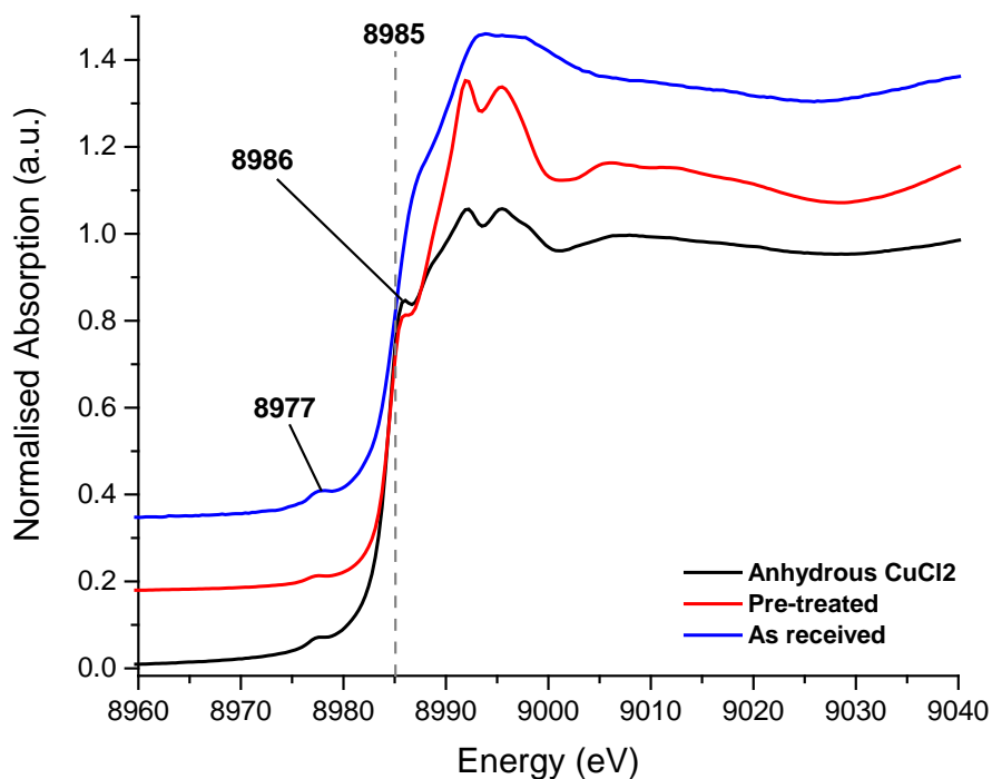
Figure 3 XANES Spectra - Fresh catalyst as received, chlorine pre-treated and the anhydrous \text{CuCl}_2 (prepared in situ )
