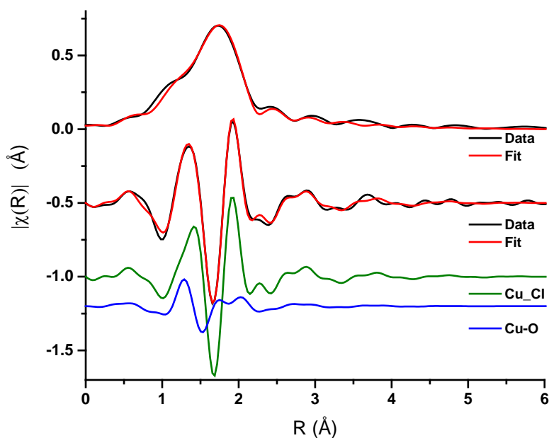
Figure 6. EXAFS spectra - Magnitude component of the k^2 weighted Fourier Transform of the data and fit for the 1 min CO exposure spectrum, and the imaginary component of the paths used in the fit.
