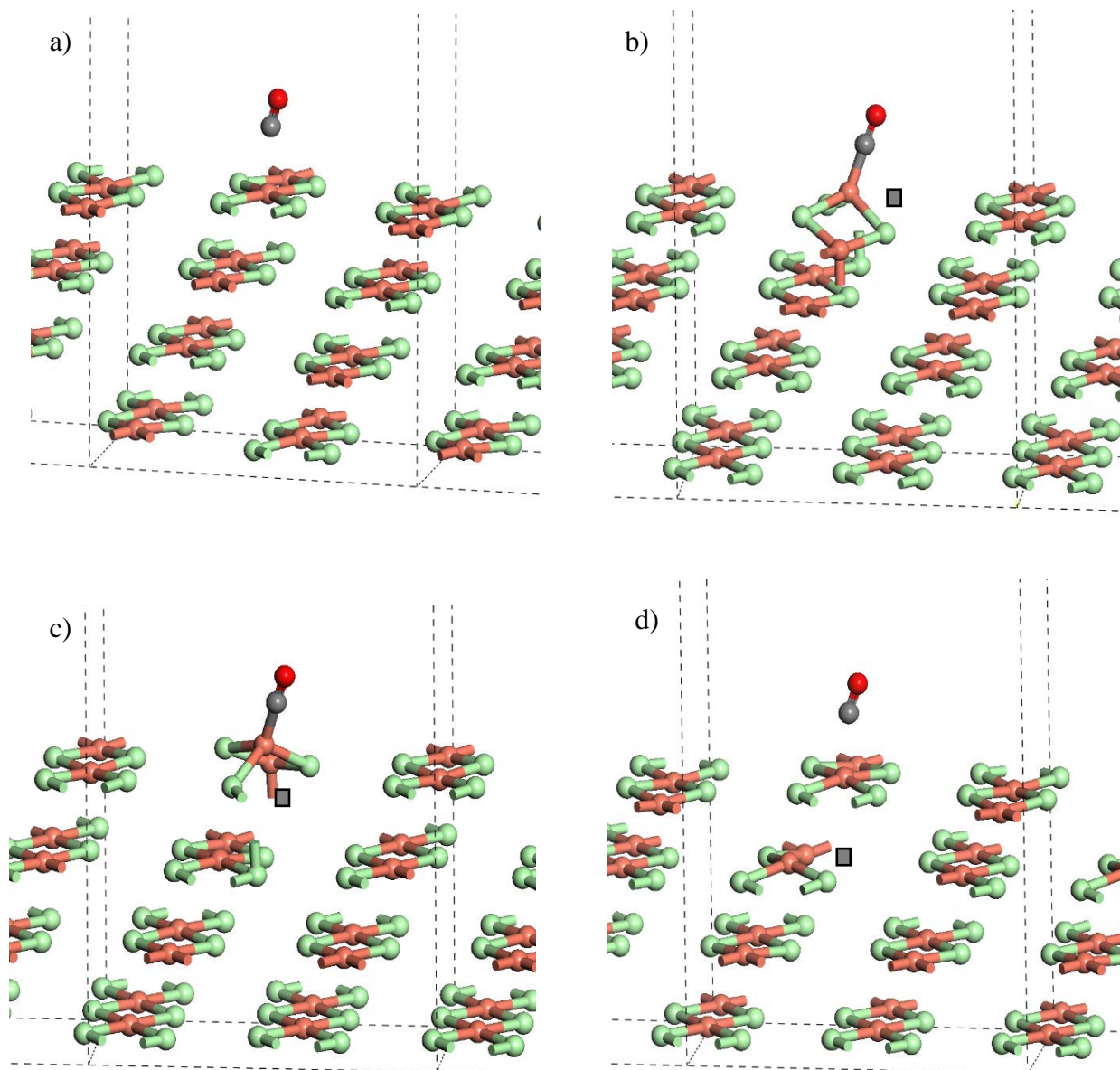
Figure 8. Calculated CO adsorption geometries on a ) Slab model of stoichiometric CuCl 2 (010) surface. b ) Structure with Cl - vacancy in surface layer of slab CO at Cu(3-fold) site, c ) Cl - vacancy in the surface layer with CO at Cu(4-fold) site and d ) structure with Cl - vacancy in second layer of slab. Note that the position of the anion vacancy is indicated by a grey square in b ) - d ) origin for cells in b ) and c ) has been shifted to place CO at the centre of the cell. All structures optimised with PBE+U using U=7 and Grimme D2 dispersion included. Atoms coloured Cu: pink, Cl: green, C: grey, O: red.
