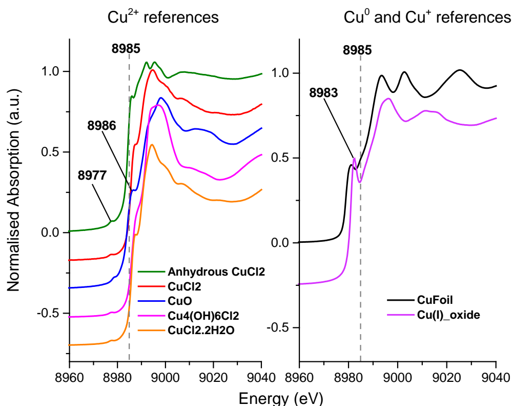
Figure 2 Ex situ XANES spectra - Left: Cu 2+ reference compounds, Right: Cu + reference compounds, spectra are vertically offset for clarity.
