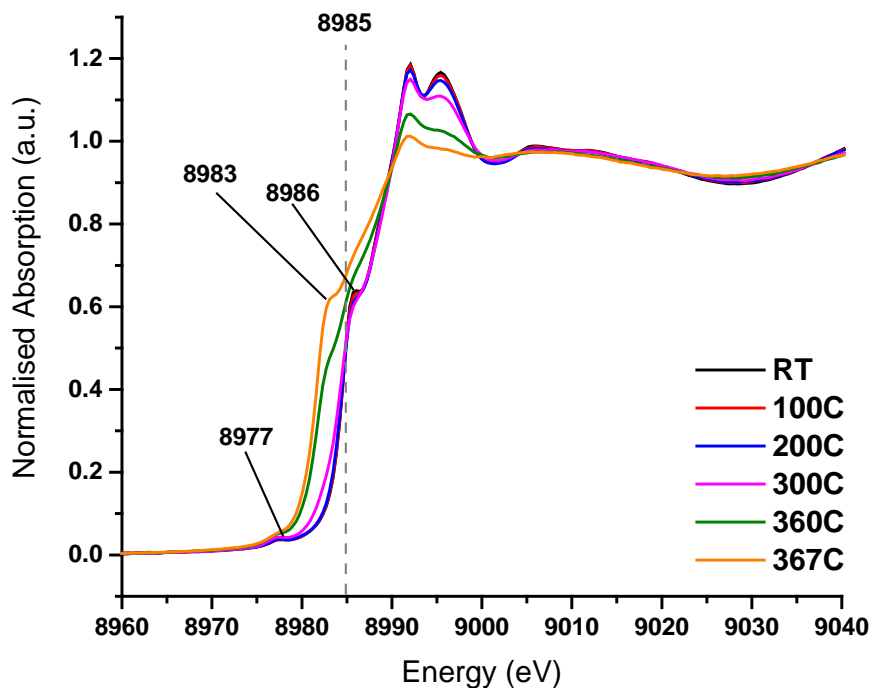
Figure 4. In situ XANES spectra - Temperature ramp of chlorine pre-treated catalyst showing loss of anhydrous-like \text{Cu}^{2+} to \text{Cu}^+ species.
