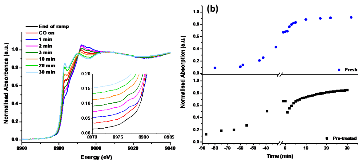
Figure 5. In situ XANES spectra - (a) From the end of the temperature ramp (367°C, under helium) then on exposure to CO. The insert shows the pre-edge region around 8977 eV in more detail. (b) The time dependence of the pre-edge feature at 8983 eV, characteristic of Cu + species during the ramp and on exposure to CO, (blue dots: fresh catalyst, black squares: Cl 2 pre-treated catalyst). Negative time points represent the temperature ramp; time t = 0 indicates the time that the catalyst was exposed to CO (temperature = 367°C).
