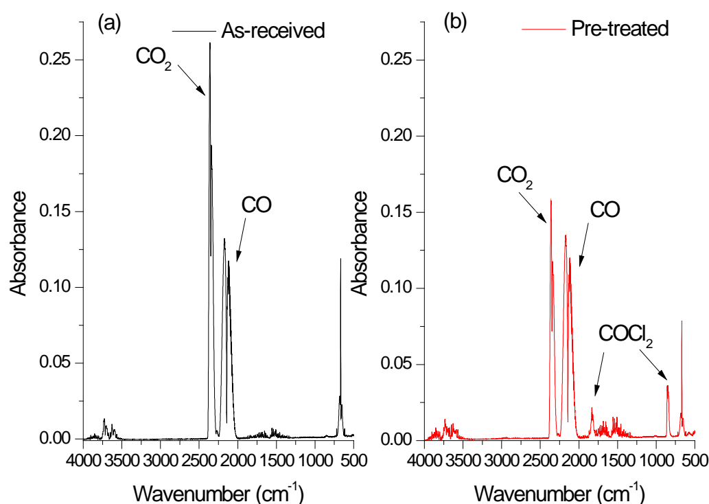
Figure 1. In-line FT-IR spectra of outlet gas mixture of CO reacting with the catalyst at 370 °C showing the effect of pre-treating the catalyst with Cl_2(g) . (a) as-received catalyst; (b) chlorine pre-treated catalyst.
