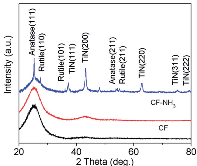
Fig. 2 XRD patterns of carbon fibres (CF), carbon fibres heated in ammonia at 800 °C (CF-NH 3 ) and carbon fibres coated with TiN (CF-TiN-1).
