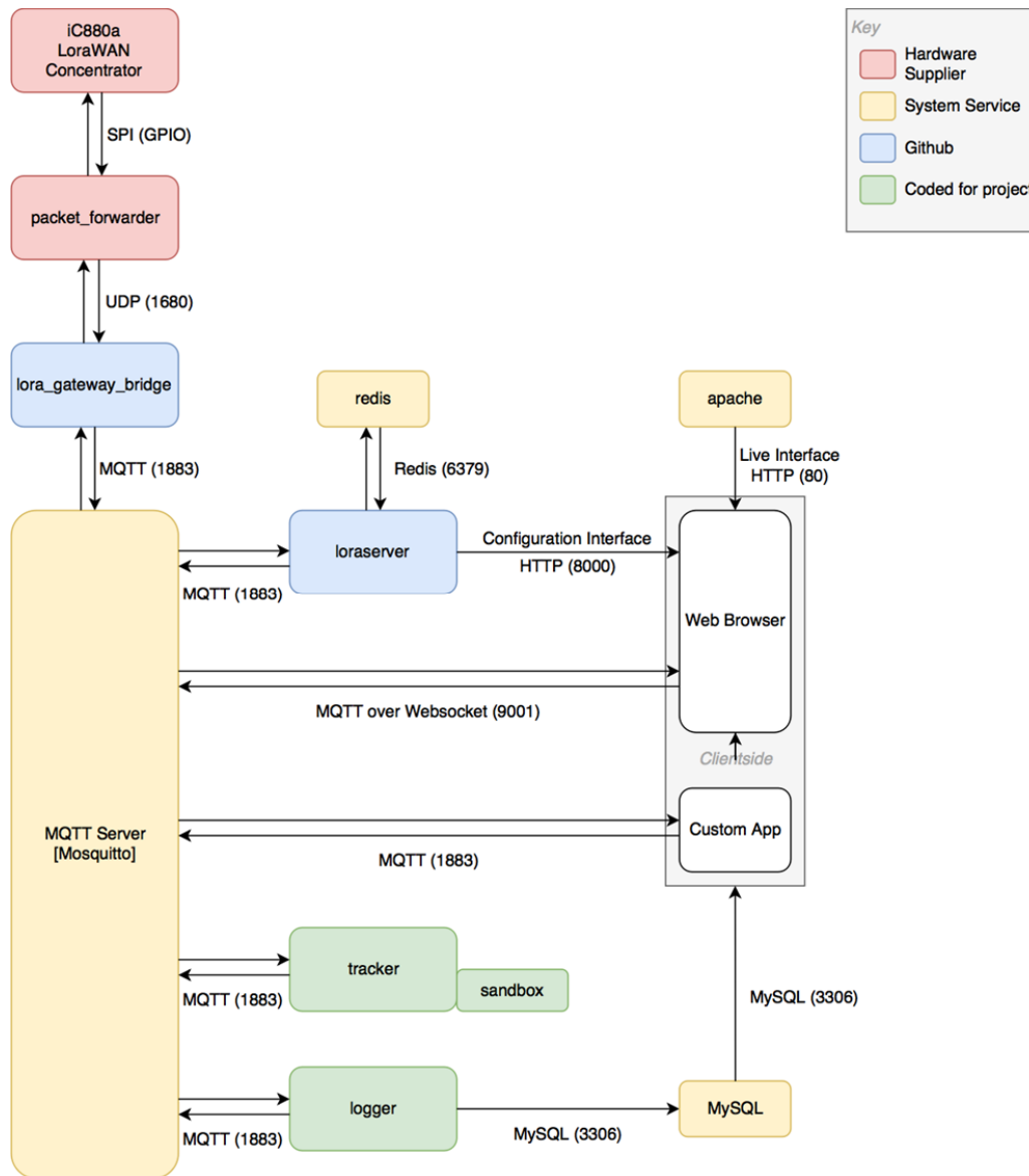
Fig. 2 Base Station Block Diagram
