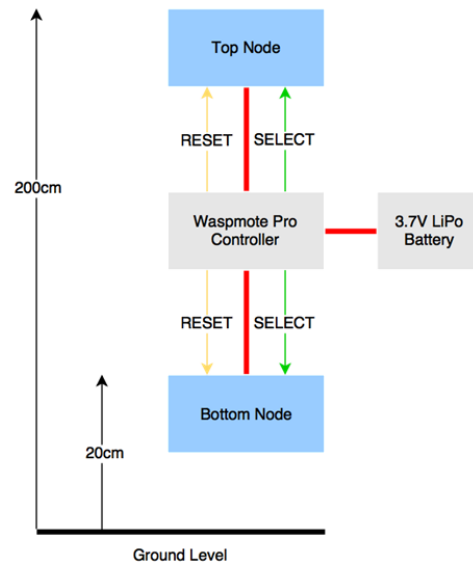
Fig. 4 Block diagram of range test apparatus
