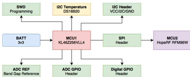
Fig. 3 Node Block Diagram
