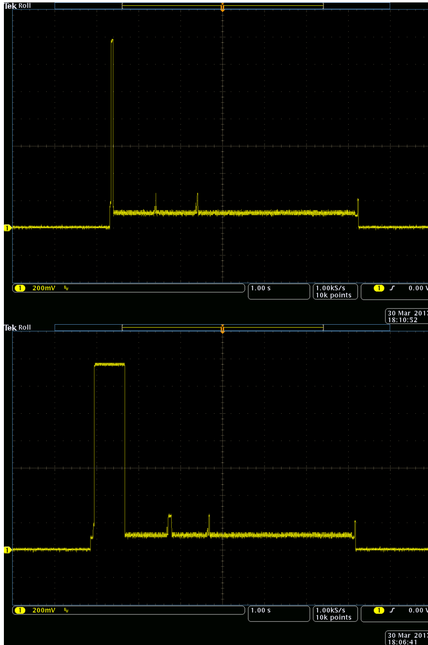
Fig. 12 Power usage against time. (Left:DR_SF7, Right: DR_SF11)
