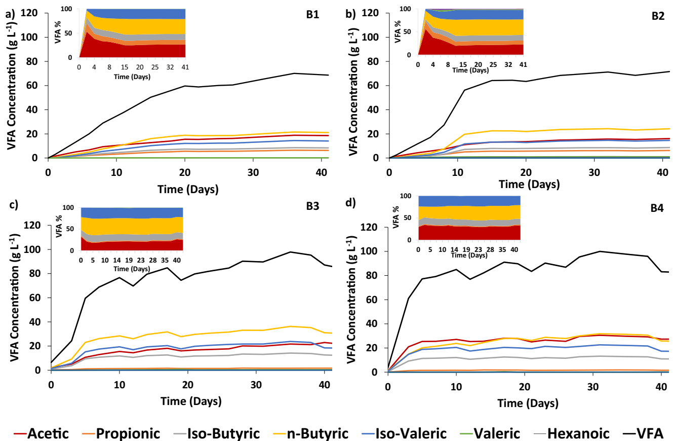
Fig. 1 VFA profiles over the course of the 1-L batch experiment. a Reactor B1. b Reactor B2. c Reactor B3. d Reactor B4. The embedded images correspond to the VFA composition for each reactor
