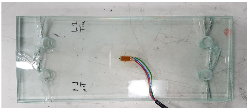
Fig. 4 The mid-length regions of the reference annealed glass specimens were undamaged
