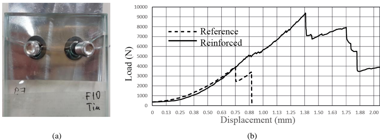
Fig. 3 (a) Failure of glass in the vicinity of the joint in annealed glass reference test specimen (b) Applied load – displacement relationships of the reference and reinforced bolted joints in annealed glass
