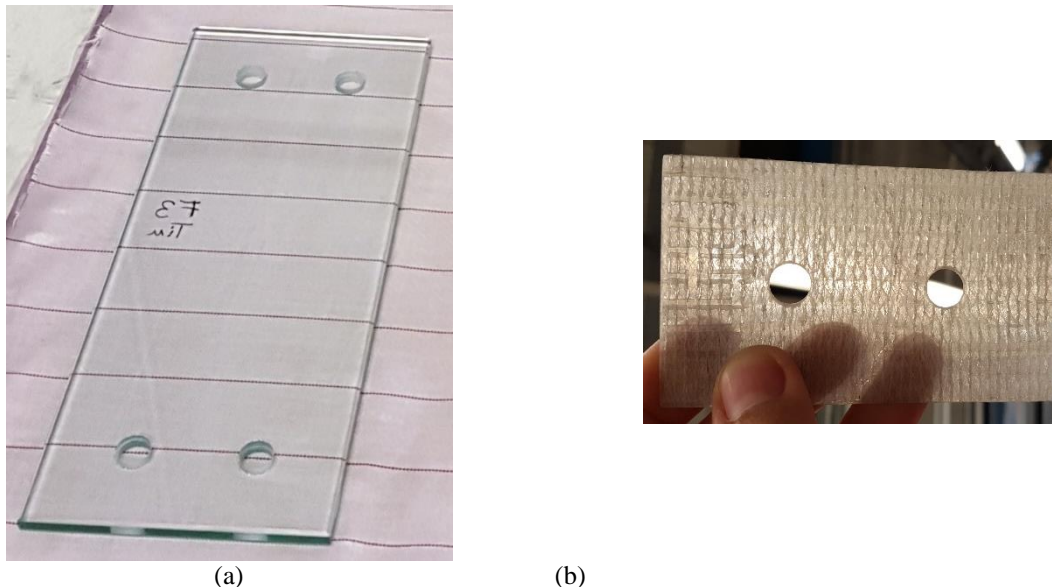
Fig. 1 (a) 250 mm x 100 mm glass specimens with four 11 mm diameter drilled holes (b) 60 mm x 100 mm GFRP strip with two 11 mm diameter drilled holes
