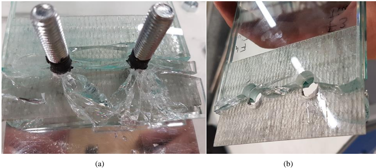
Fig. 7: Failure of glass in a reinforced annealed glass joint configuration (a) Glass fractured in the vicinity of the bolts (b) The GFRP strip remains intact although the glass has fractured
