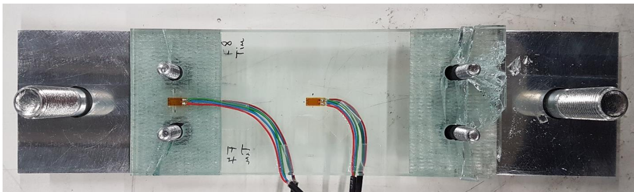
Fig. 6 Failure pattern of a reinforced annealed glass test specimen
