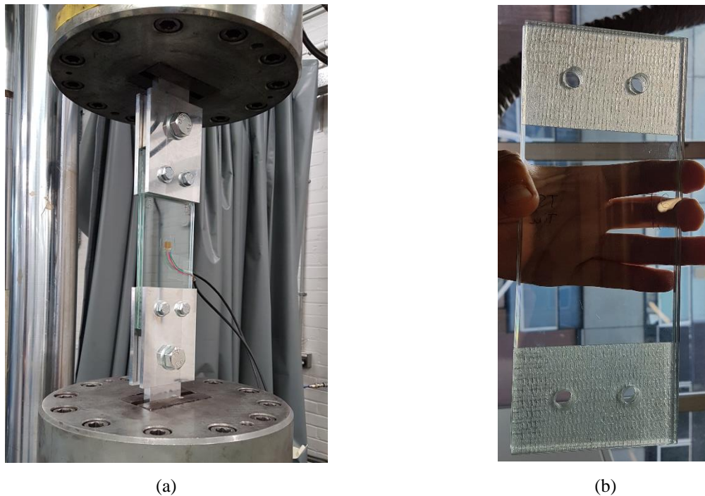
Fig. 2 (a) Test arrangement of a reference test specimen (b) Two glass pieces with an adhesively bonded GFRP strip between the two glass pieces
