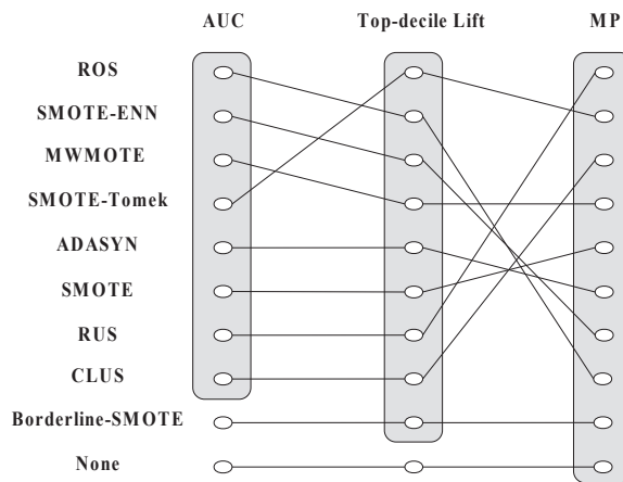
Figure 4: Rankings of sampling techniques with SVM
