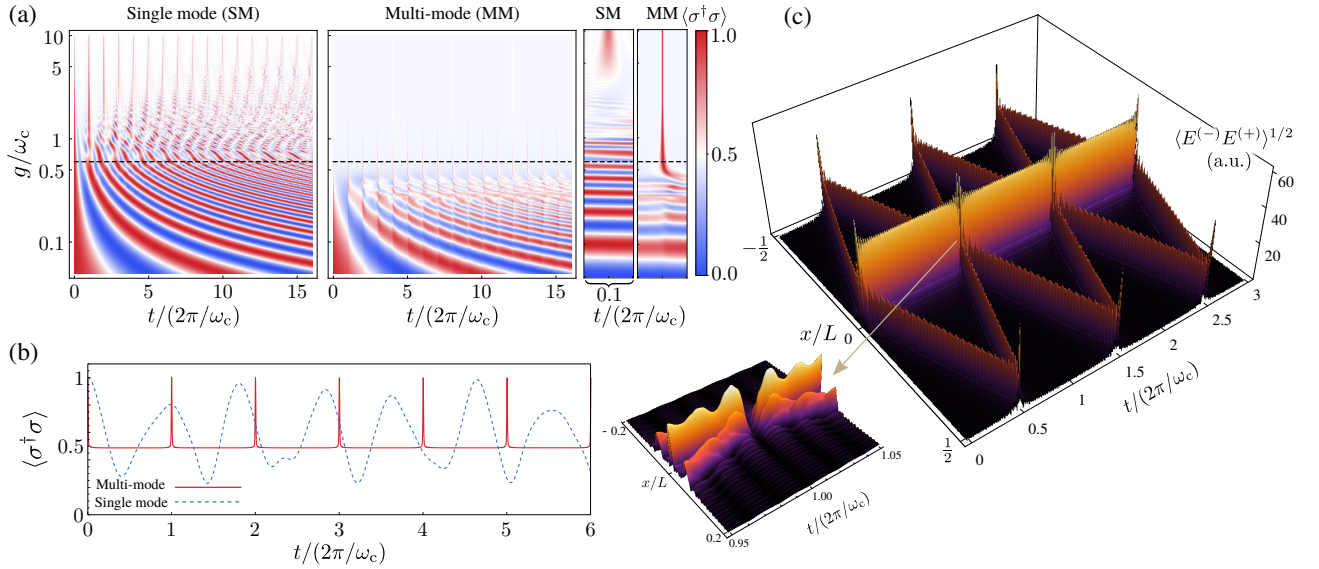
FIG. 2: Breakdown of the Rabi model observed through the system dynamics. (a) Contour plot of the TLS population versus time and coupling rate. The dashed line marks the value g/\omega_c \approx 0.6 chosen for the rest of the simulations. Above this value, the single-mode Rabi model differs drastically from the multi-mode model. Insets on the right show a zoom view around a revival peak. (b) Population of an initially excited TLS versus time for the single-mode (blue, dashed) and multi-mode (red, solid) cases, for a coupling rate of g/\omega_c = 0.6 . (c) Amplitude of the electric field inside the cavity (square root plotted for clarity) as a function of space and time, for g/\omega_c = 0.6 . The inset focus on the precise moment when the field is perfectly absorbed by the emitter, giving rise to the revival peaks in the population of the TLS. Computed using the technique of MPS including 50 cavity modes.
