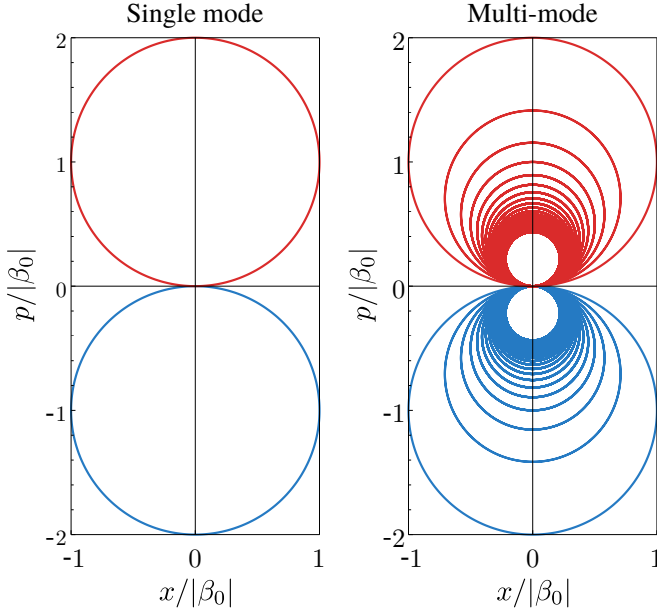
FIG. 3: Phase space trajectories of the cavity modes. Trajectories in phase space for the single-mode case (left) and the multi-mode case (right), in which the trajectories of successive modes are plotted up to n = 20 . Red (blue) curves correspond to the trajectories for an initial |+\rangle ( |-\rangle ) state in the TLS.
