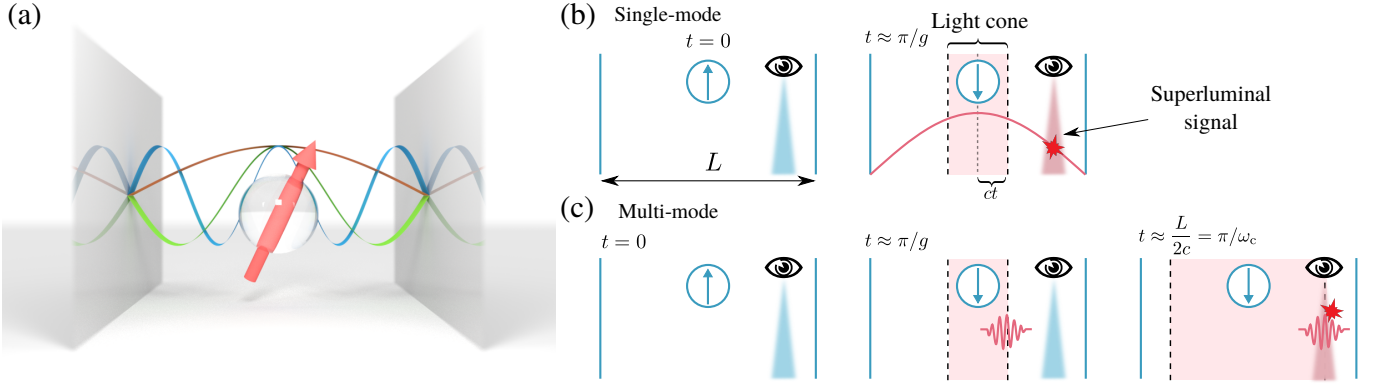
FIG. 1: The problem of superluminal signalling in the single-mode Rabi model. (a) Schematic view of a qubit embedded in a perfect 1D cavity, together with the depiction of the three lowest cavity modes. When the qubit is only coupled to the fundamental mode, the system is described by the Rabi Hamiltonian. (b) Violation of relativistic causality by the single-mode Rabi model in regimes where g \approx \omega_c . An observer placed close to the cavity edge can retrieve information about the initial state of the TLS before light is able to reach its position. (c) A multi-mode description is able to capture the spatio-temporal structure of the light field necessary to comply with causality.
