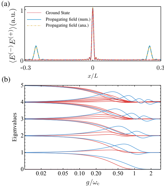
FIG. 4: Ground state and eigenvalues of the multi-mode Rabi model. (a) Red, dashed line: Amplitude of the electric field inside the cavity corresponding to the ground state of the system for g/\omega_c = 0.6 . Solid, blue (dashed-dotted, yellow): numerical (analytical) calculation of the electric field for an initial state |e\rangle|0\rangle after evolving for a time t = \pi/2\omega_c , confirming that the dynamics of the system is given by the independent evolution of two freely propagating wavepackets plus a localized cloud of photons corresponding to the ground state of the light-matter system. (b) Low-energy spectrum of the single-mode (red) and multi-mode (blue) Rabi Hamiltonian as a function of the coupling rate. For each value of g , the eigenvalues are expressed with respect to the ground state. Here, \omega_x = \omega_c .
