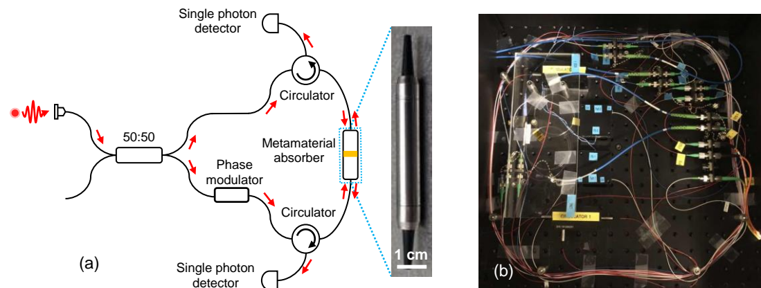
Fig. 1. Fiber-optic quantum network for active single photon switching using a fiberized plasmonic metamaterial absorber (inset shows a picture of the packaged metadevice): (a) schematics; (b) photograph.
