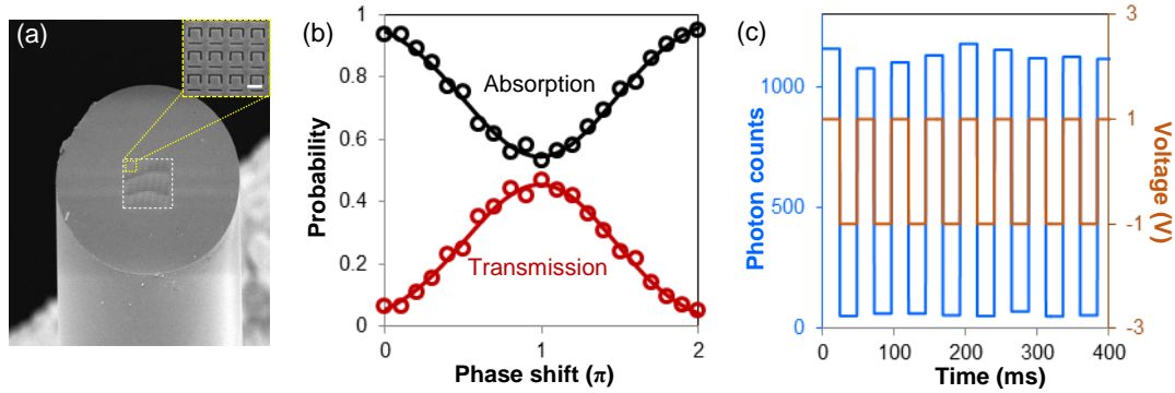
Fig. 2. a) SEM image of the plasmonic metamaterial absorber deposited on the end-facet of the optical fiber (inset shows the SEM image of individual asymmetric split ring resonators, scale bar is 500 nm); b) Single photon absorption and transmission probability by continuous phase shift modulation; c) Demonstration of single photon switching with 20 ms acquisition time: blue line shows the photon counts level, brown line shows the control voltage applied to phase modulator.
