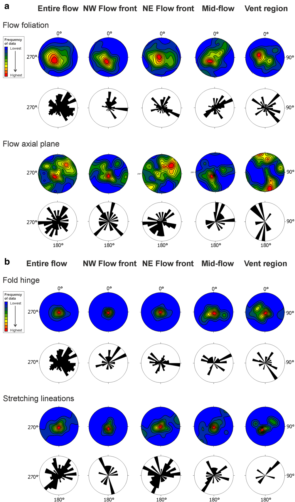
Fig. 7 Planar and linear data projected as density plots and rose diagrams (see divisions in Fig. 4). Statistical summary data available in Electronic supplementary material 2
