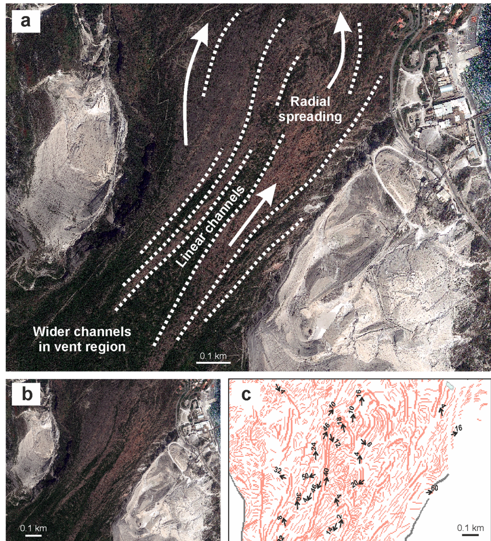
Fig. 8 Linear flow channel ridges mid-flow. a Interpretation of GeoEye-1 image with traced flow channels and radial spreading beyond channel. b Original GeoEye-1 image. c Structural measurements of stretching lineations in mid-flow region, the majority of measurements trending approximately NE-SW (flow direction)
