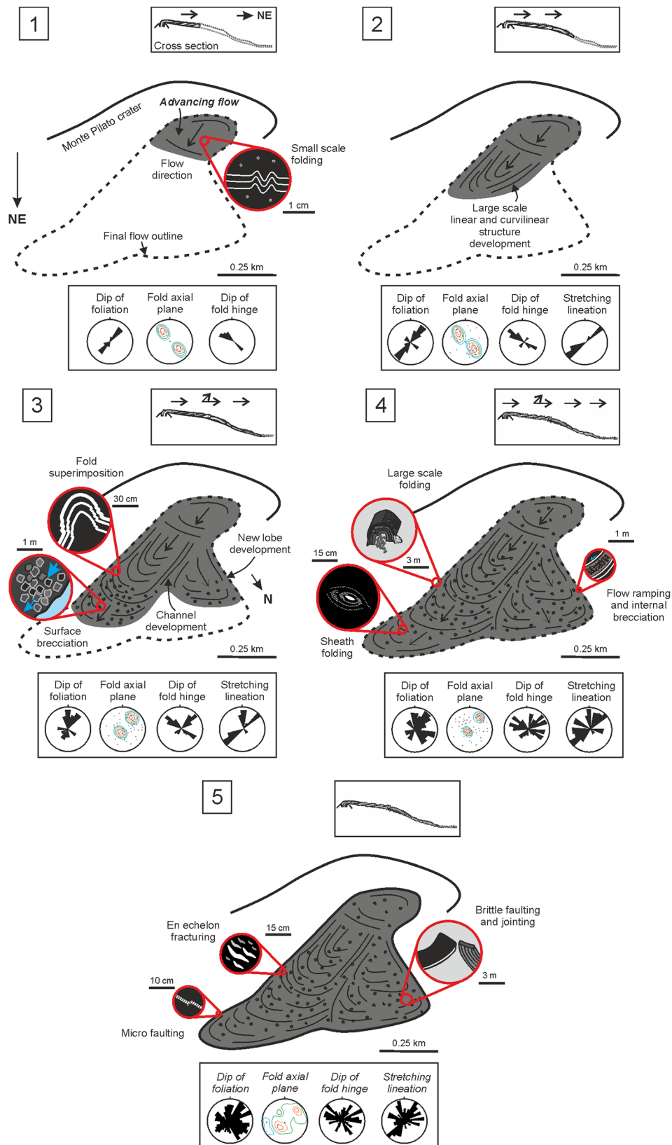
Fig. 9 Model for the emplacement of the Rocche Rosse lava flow, emplaced sequentially over five stages: (1) Initial extrusion (moving NE), crustal development and small-scale folding. (2) Extensional strain, stretching lineations and channel development over steeper topography. (3) Compression at topographic break, autobrecciation, lobe development
