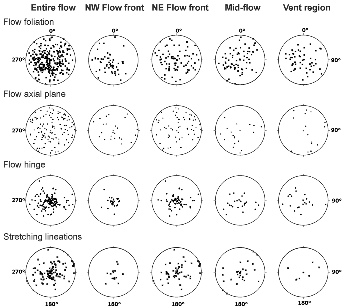
Fig. 6 Stereographic plots of flow foliations, fold axial planes, fold hinges and stretching lineations (equal area projection, lower hemisphere). Data divided into a entire flow, b NW flow front, c NE flow front, d mid flow and e vent region (see Fig. 4)
