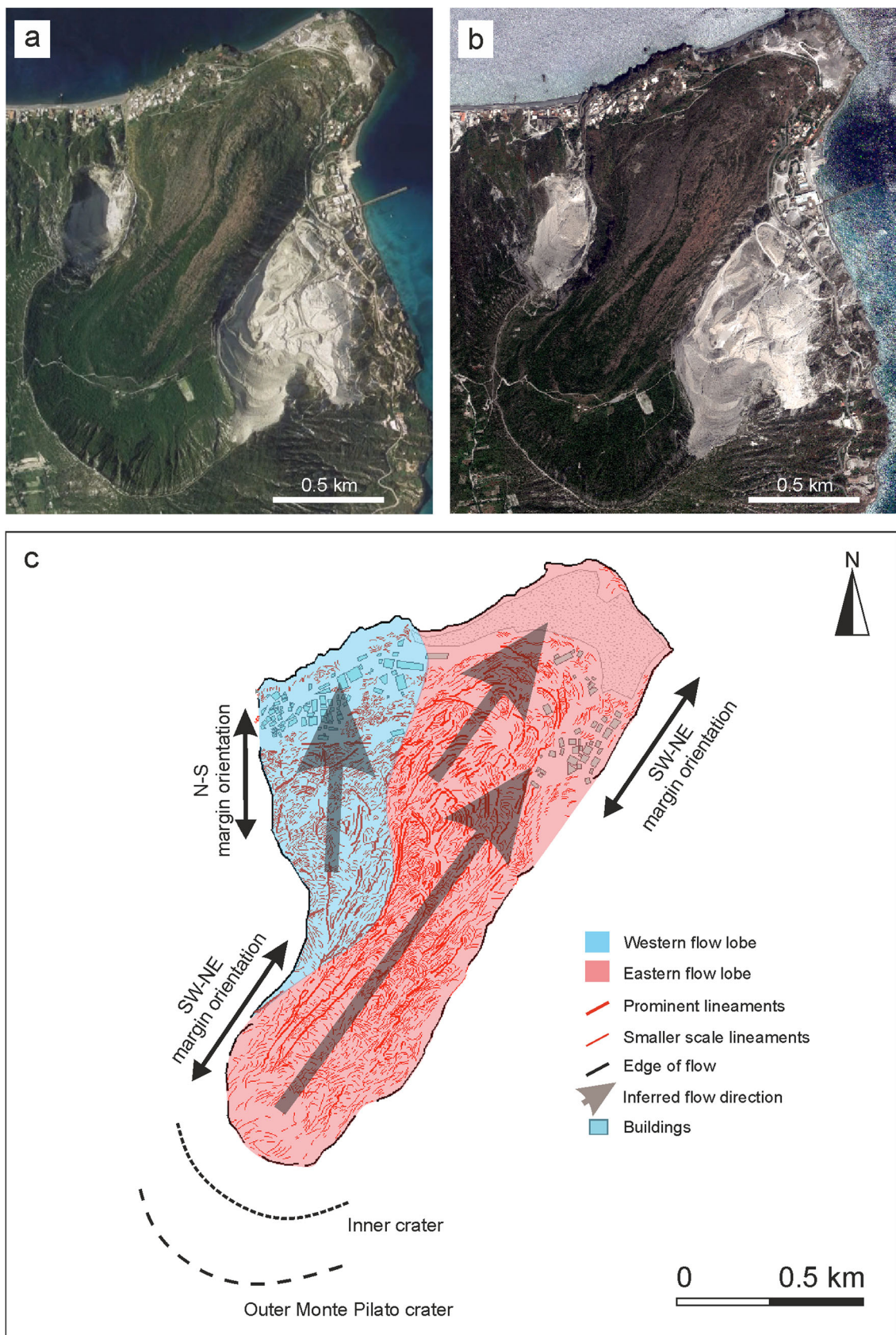
Fig. 3 a Google Earth image (Map data: SOI, NOAA, U.S. Navy, NGA, GEBCO, TerraMetrics, ©2018 Google) and b GeoEye-1 image of the Rocche Rosse rhyolitic lava flow. c Annotations of the Rocche Rosse lava
