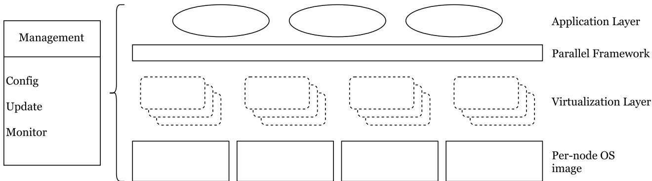
Figure 3: Schematic diagram of typical Single Board Computer (SBC) cluster configuration.
