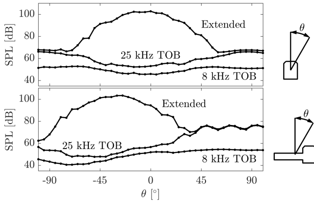
FIG. 11. Directivity of hairdryer 2 taken at 5 degree increments for the extended SPL and the TOBs of the two prominent tones: Top - horizontal directivity, Bottom - vertical directivity.
