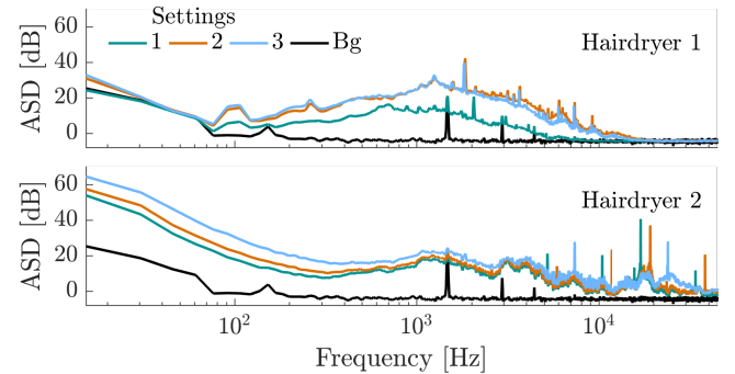
FIG. 10. (Color online) Autospectral density of the two hairdryers on three setting.
