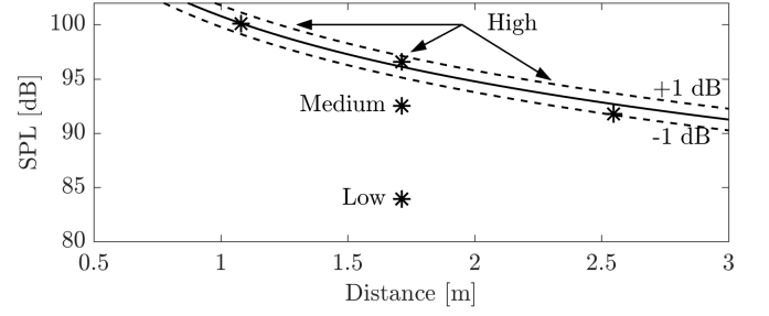
FIG. 1. Z-40-weighted SPL of the Balcony Guard for three settings at one distance and three distances at the high setting. The solid line is a best-fit assuming spherical spreading. The \pm 1 dB dashed lines show that the three distances fall within that bound.
