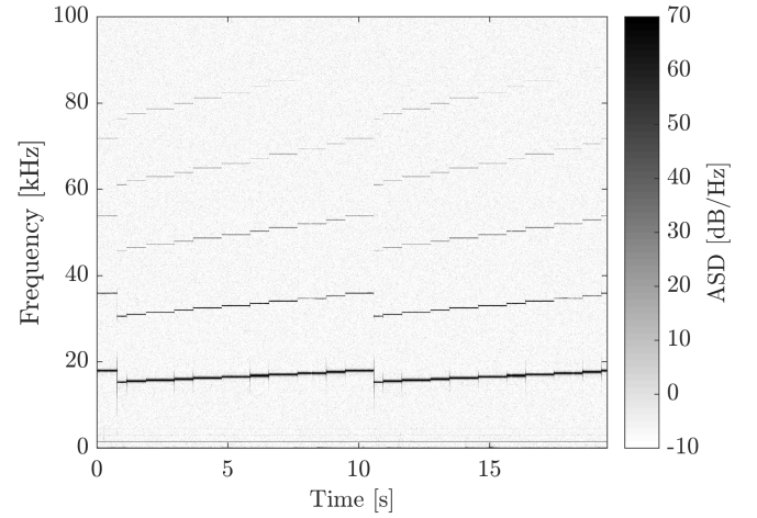
FIG. 5. Spectrogram of the multipurpose pest deterrent on the first setting.
