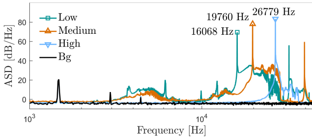
FIG. 3. (Color online) Autospectral Density of the Balcony Guard on the low, medium, and high settings along with the background noise floor (Bg) of the measurements. The highest amplitude tones are marked and labeled with the frequency at which they occurs.
