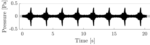
FIG. 7. Time series showing the signal envelope of the spider deterrent. Analysis period in black.
