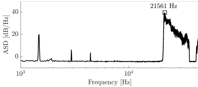
FIG. 8. ASD for the spider deterrent. The highest amplitude is marked with as square and labeled with the frequency at which it occurs.
