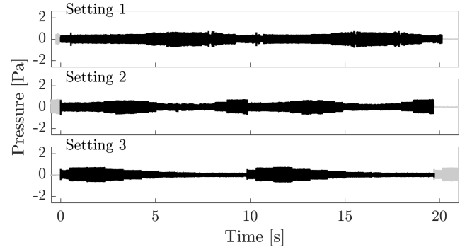
FIG. 4. Time series showing the signal envelope of the multipurpose pest deterrent on the settings 1, 2, and 3. Analysis period in black.
