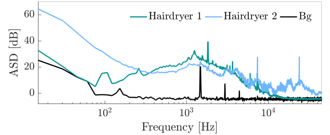
FIG. 9. (Color online) Autospectral density of the hairdryers on the highest setting.
