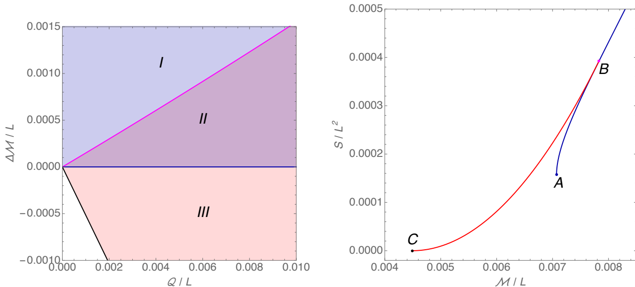
FIG. 1: Left Panel: Region of existence of solutions. We plot the quasiloal mass difference \Delta\mathcal{M} = \mathcal{M} - \mathcal{M}_{ext} (between a given solution and the extremal caged RN BH with the same charge Q ) as a function of the quasiloal electric Q for e = qL = 3.5 . Caged RN black holes exist in regions I and II . The magenta line with positive slope splitting these two regions describes the onset curve of the superradiant instability (RN BHs are unstable in region II ). The black line with negative slope describes the soliton family. Hairy black holes exist in between these two lines, i.e. in regions II and III (red shaded area). Right Panel: Phase diagram in the microcanonical ensemble i.e. adimensional entropy S/L^2 as a function of the adimensional quasiloal mass \mathcal{M}/L at constant value of the quasiloal charge Q/L = 0.005 and e = 3.5 . The blue line starting at A (extremality) is the RN black hole and the red line BC is the hairy back hole branch that ends at the soliton C . The merger point B (superradiant instability onset) signals a second order phase transition.
