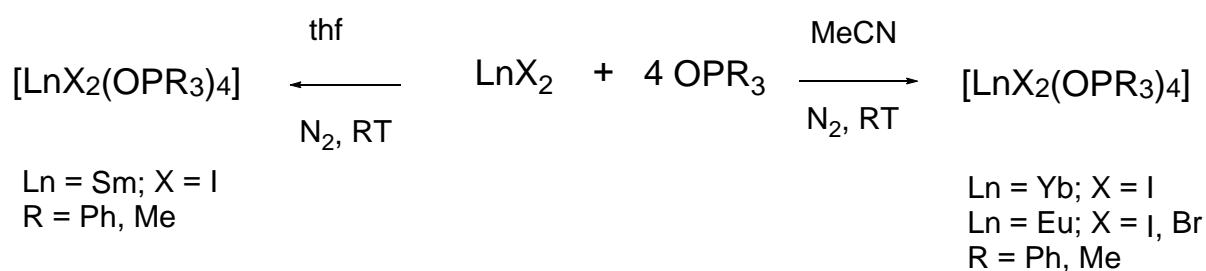
Scheme 1: Synthesis of \text{LnX}_2 phosphine oxide complexes
