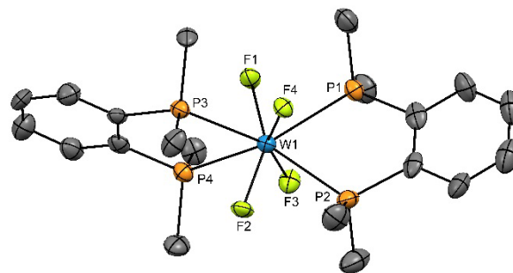
Fig. 1. The cation present in [\text{WF}_4\{o\text{-C}_6\text{H}_4(\text{PMe}_2)_2\}_2][\text{WOF}_5]_2 \cdot \text{MeCN} showing the atom numbering scheme and with ellipsoids drawn at the 50% probability level. H atoms are omitted for clarity. Selected bond lengths ( \text{\AA} ) and angles ( ^\circ ): \text{W}(1)\text{--F}(3) = 1.91(4) , \text{W}(1)\text{--F}(2) = 1.92(4) , \text{W}(1)\text{--F}(1) = 1.92(4) , \text{W}(1)\text{--F}(4) = 1.93(4) , \text{W}(1)\text{--P}(3) = 2.572(17) , \text{W}(1)\text{--P}(1) = 2.579(18) , \text{W}(1)\text{--P}(2) = 2.582(18) , \text{W}(1)\text{--P}(4) = 2.592(18) , \text{P}(3)\text{--W}(1)\text{--P}(4) = 72.6(6) , \text{P}(1)\text{--W}(1)\text{--P}(2) = 72.8(6) .
