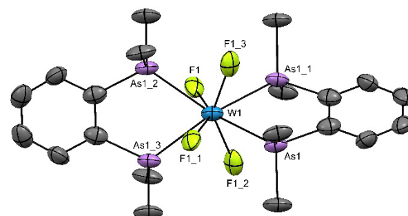
Fig. 2. The cation present in [\text{WF}_4\{o\text{-C}_6\text{H}_4(\text{AsMe}_2)_2\}_2][\text{WF}_8]_2 showing the atom numbering scheme and with ellipsoids drawn at the 50% probability level. Hydrogen atoms are omitted for clarity. Selected bond lengths ( \text{\AA} ) and angles ( ^\circ ): \text{W}(1)\text{--F}(1) = 2.114(6) , \text{W}(1)\text{--As}(1) = 2.6279(10) , \text{As}(1)\text{--W}(1)\text{--As}(1)\#1 = 75.74(4) . Symmetry operators: \#1 = -x+5/4, -y+5/4, z ; \#2 = x, -y+5/4, -z+1/4 ; \#3 = -x+5/4, y, -z+1/4 .
