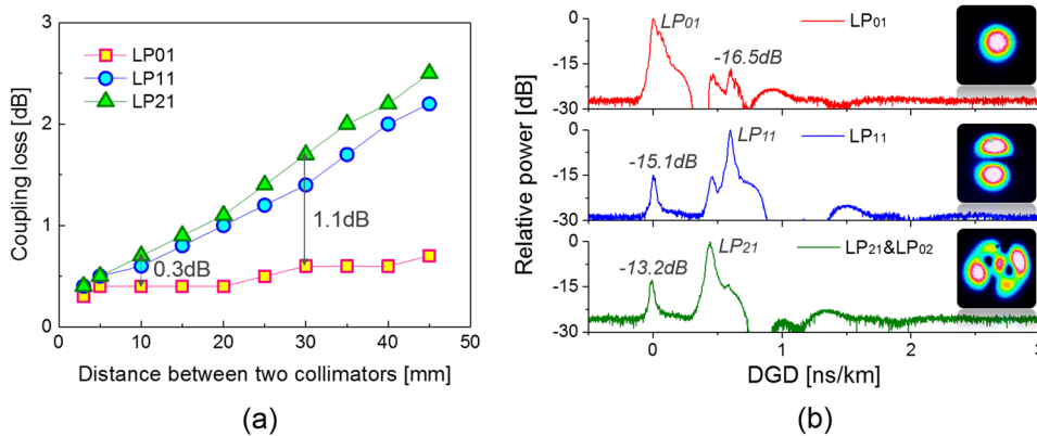
FIG. 3. (a) Mode dependent coupling loss as a function of distance between two 4-mode group fiber collimators and (b) impulse response from a pair of four mode group fiber collimators.
