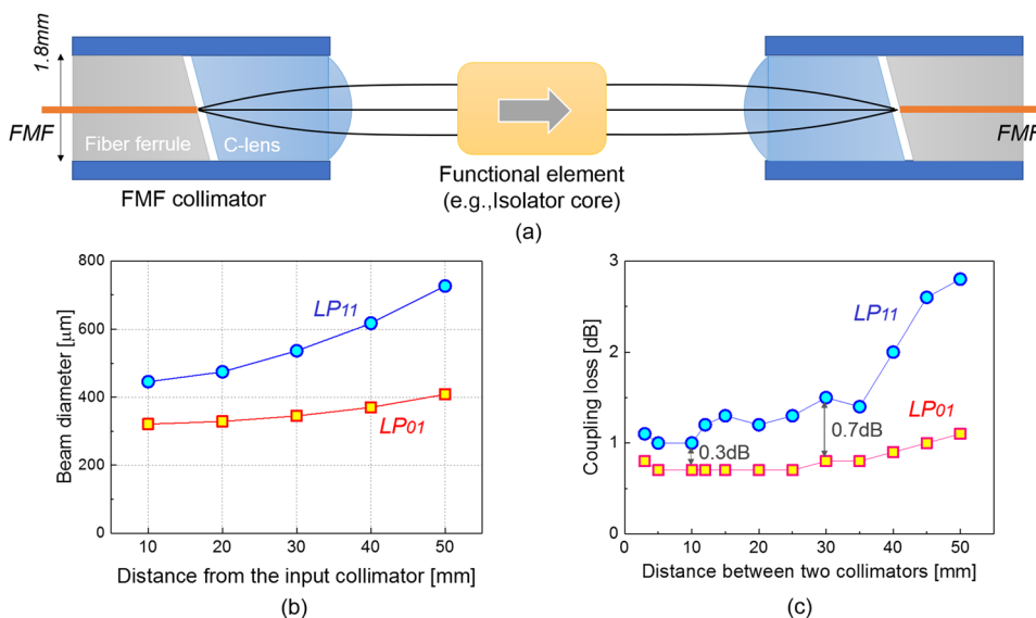
FIG. 1. (a) Schematic of a few-mode fiber (FMF) collimator assembly incorporating an optical isolator as a functional element. (b) The measured beam diameters of both LP_{01} and LP_{11} modes as a function of distance from the input fiber collimator and (c) the mode dependent coupling loss between two collimators.
