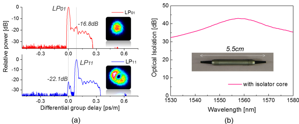
FIG. 2. (a) The estimated modal purity based on temporal impulse response measurements from a pair of FMF collimators incorporated at the input to a 10 km length of FMF and (b) optical isolation of the FMF isolator.
