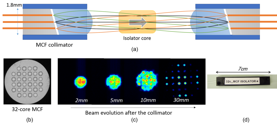
FIG. 4. (a) Schematic of a 32-core MCF isolator. (b) The cross section of the 32-core MCF, (c) the measured beam profiles as a function of distance from the collimator, and (d) the fully integrated and packaged isolator.
