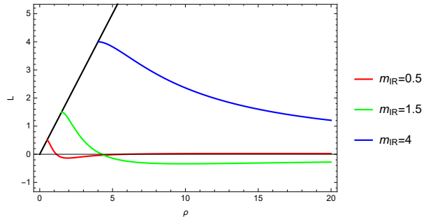
FIG. 2: The functions L(\rho) with m = 0 in the far UV for N_f = 9 . In the IR we cut off scales below where the quarks become on mass shell when L(\rho = m_{IR}) = m_{IR} . Here the BF bound is violated at r = 11 .
