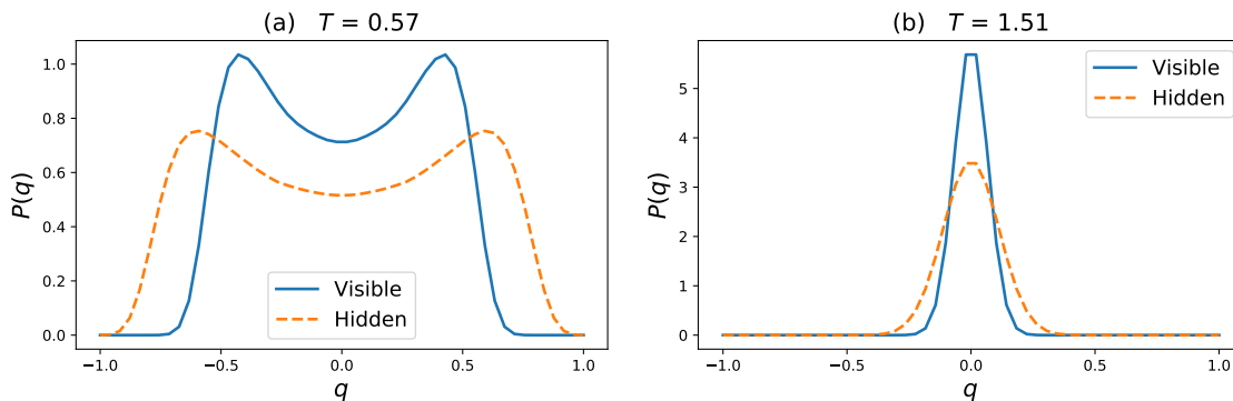
Figure 9: Overlap distribution, P(q) , for the visible spins (blue, solid) and the hidden spins (orange, dashed), for (a): a temperature in the spin glass phase, and (b): a temperature in the paramagnetic phase. The distributions are estimated from N = 400 , \alpha_h = 0.25 MC samples using Parzen windows with a standard deviation of 0.05. In an infinite RSB analysis, one would expect delta function peaks at the maximal values of q , though these divergences are difficult to capture with finite- N simulations.
