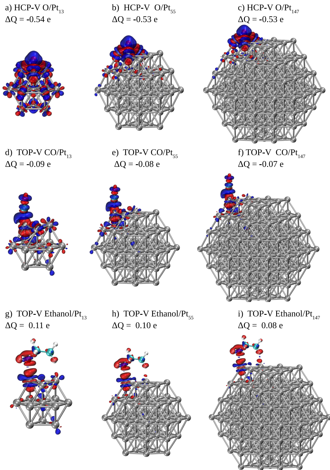
Fig. 6 Electronic density differences plots for O, CO and ethanol interacting with Pt 13 , Pt 55 , and Pt 147 nanoparticles (Isosurface at 0.02e/\text{\AA}^3 ), where blue (red) represents electron accumulation (depletion). The numbers associated with each plot are overall Mulliken charge differences calculated for each adsorbate, where a negative number represents adsorbate receiving electrons. We show the results for O interacting in the HCP-V adsorption site and CO and ethanol adsorbed on TOP-V sites.
