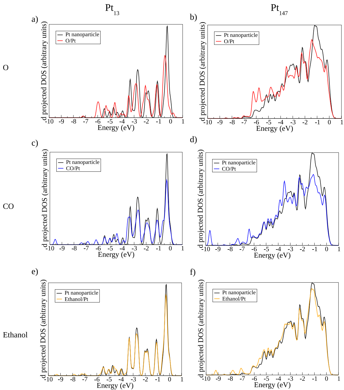
Fig. 7 Local density of states projected on the d-band of surface Pt atoms in the interacting region of the (111) facet. Figure a), c), and e) show the density of states for Pt 13 interacting with O, CO, and ethanol. Figure b), d), and f) show O, CO, and ethanol interacting with Pt 147 .
