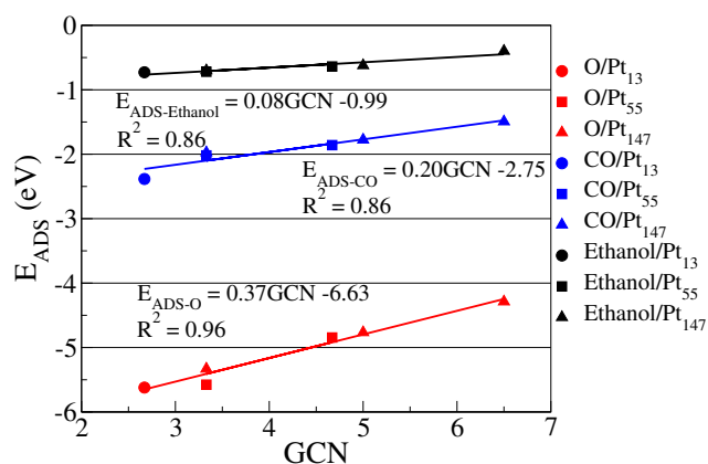
Fig. 4 Adsorption energies for oxygen (red), carbon monoxide (blue), and ethanol (black) interacting with different top sites on (111) facets versus the generalized coordination number relative to each adsorption site. Circles, squares, and triangles represent Pt 13 , Pt 55 , and Pt 147 nanoparticles.
