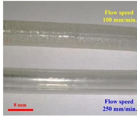
Fig. 2 Extruded structures with different filament feeding speeds at T = 240 °C.
