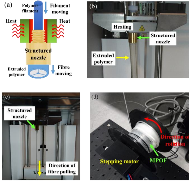
Fig.3 (a) Schematic and (b) photograph of the experimental setup used to extrude MPOF. (c) Fiber drawn from the heated structured nozzle. (d) MPOF wrapped onto the 3D printed spool connected to the stepper motor.
