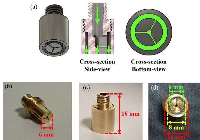
Fig.1 (a) Structured nozzle design including a 3D model, a side- and a bottom-view cross-sections, from left to right respectively. Green arrows and green colours represent the direction of filament moving and cross-section of extruded polymer from structured nozzle. (b-d) Micromachined structured nozzle: (b) body, (c) body + cover, (d) after MPOF drawing.
