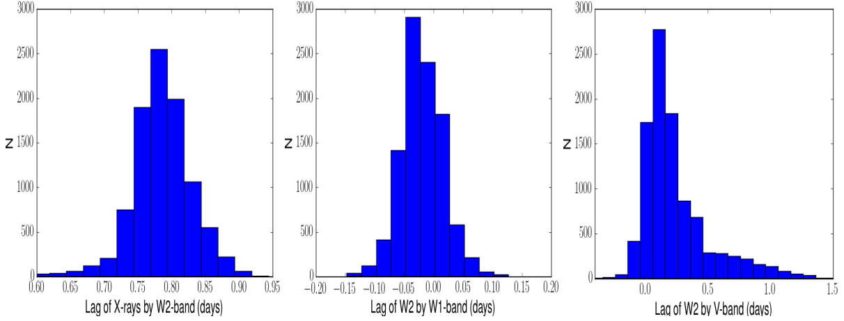
Figure 6. Lag probability distributions from JAVELIN for (left panel) UVW2 relative to the X-rays, (centre) UVW1 relative to UVW2 and (right) V-band relative to UVW2.
