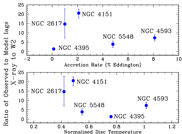
Figure 17. As for Fig. 16 except that the ratio of observed to model lags is for the X-ray to W2 band lag.
