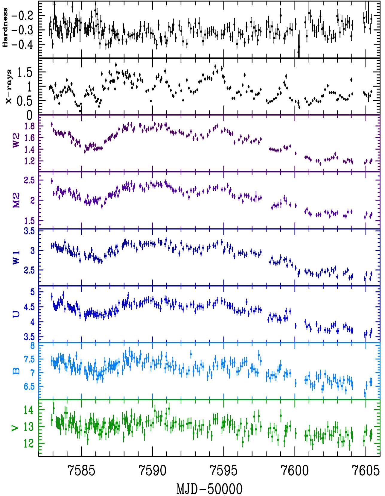
Figure 1. XRT and UVOT lightcurves of NGC 4593. The top panel is the hardness ratio defined as H-S/H+S where H is the 2-10 keV count rate and S is the 0.5-2 keV count rate. The second from top panel is the 0.5-10 keV count rate for each visit. The lower panels are the UVW2 through to V-band fluxes in units of mJy.
