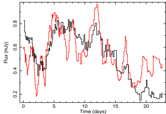
Figure 12. Observed UVW2 lightcurve (black) with model UVW2 lightcurve (red) based on a simple disc reprocessing. The normalisation of the simulated lightcurve is arbitrary. The zero point is the start of the intensive monitoring period.
