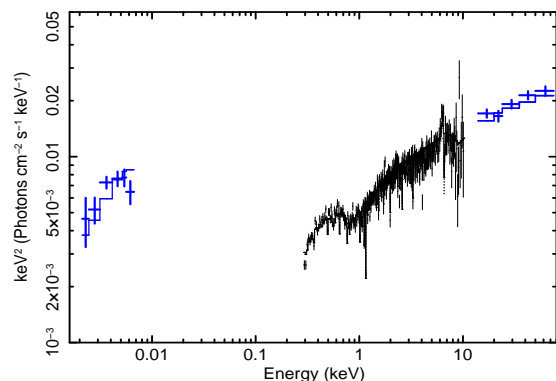
Figure 14. Broad band \nu F(\nu) SED of NGC 4593, including the variable UVOT components, fitted to the same model as in Fig. 2, together with a disk black body in the UVOT bands.
