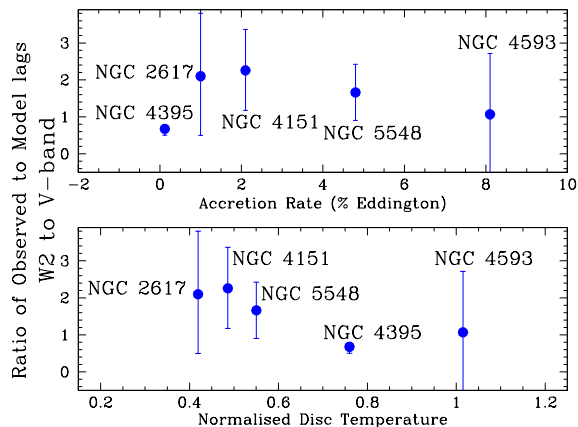
Figure 16. The ratio of observed to model lags for the W2 to V band lag. In the upper panel the ratio is plotted as a function of accretion rate and in the lower panel as a function of normalised disc temperature, i.e. (\dot{m}_E/M)^{1/4} . The model assumes reprocessing of X-rays by a standard optically thick accretion disc (Shakura & Sunyaev 1973). The data from which this plot is produced are given in Table 3.
