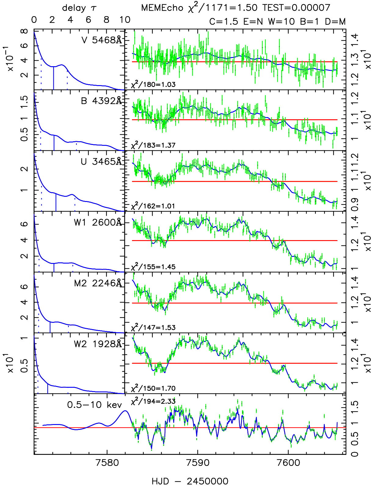
Figure 15. MEMEcho fit of the linearised echo model to Swift lightcurves of NGC 4593. Bottom panel: X-ray (0.5-10 keV) lightcurve data along with the fitted model X(t) . Left column: Delay distributions \Psi(\tau|\lambda) for three UV (UVW2, UVM2, UVW1) and three optical (U, B, V) bandpasses. Right column: Swift lightcurve data along with the echo lightcurves obtained by convolving X(t) with \Psi(\tau|\lambda) . Vertical (blue) lines indicate the median (solid) and quartiles (dashed) of the delay distributions. Horizontal (red) lines indicate the reference levels X_0 for the X-ray lightcurve and F_0(\lambda) for the echo lightcurves. The fit shown is for \chi^2/N = 1.5 with W = 10 to make X(t) 10 times more flexible than \Psi(\tau|\lambda) . Note the two-component structure of the delay maps, with a prompt response peak at \tau = 0 and extended response reaching to \tau = 10 d.
