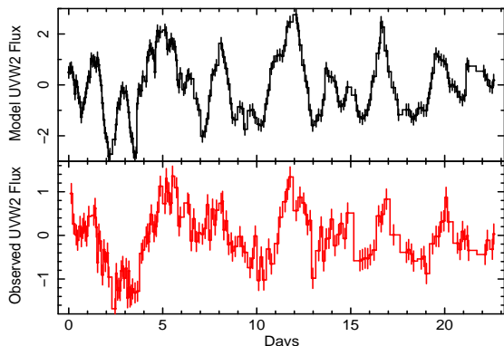
Figure 13. The model (upper panel) and observed (lower panel) UVW2 lightcurves from Fig. 12 following subtraction of the mean level derived from smoothing with a 5d wide boxcar.
