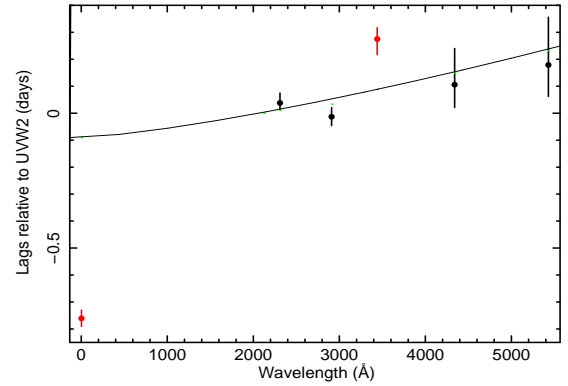
Figure 8. Lags relative to UVW2 derived using JAVELIN Zu et al. (2011, 2013) . The thin line is a power law fit with index 4/3 to the model lags (shown as small green dots). Here the model lag is the time for half of the light to be received.
