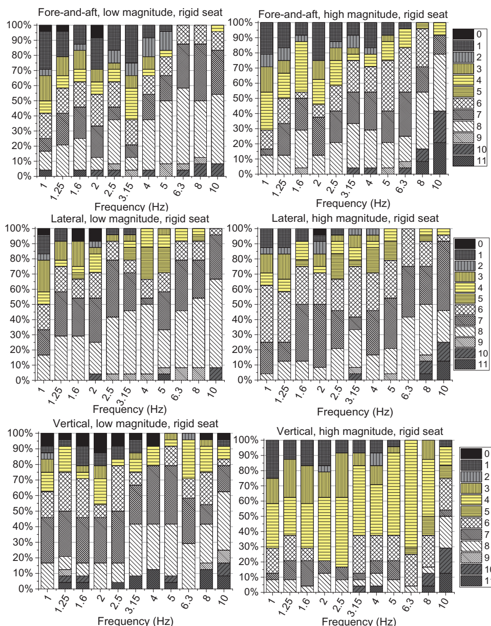
Figure 6. Reported body locations of most discomfort in each axis of vibration, at 'low' magnitudes ( 0.088 \text{ ms}^{-2} r.m.s., weighted) and 'high' magnitudes ( 0.70 \text{ ms}^{-2} r.m.s., weighted) with a rigid seat. Body locations – 0: 'no discernible location'; 1: head; 2: neck; 3: shoulders; 4: chest; 5: arms; 6: lower abdomen; 7: ischial tuberosities; 8: lower thighs; 9: upper thighs; 10: legs; and 11: feet.
