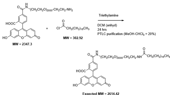
Scheme 1. Synthesis of Fluorescein-PEG-stearate
