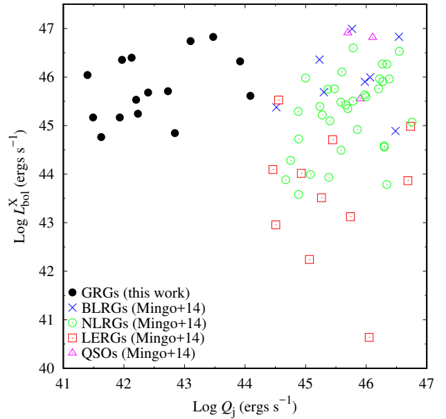
Figure 3. Bolometric luminosity estimated from the 2–10 keV luminosity versus jet power estimated from the relation of Willott et al. (1999). Black dots denote the GRGs of our sample, overlaid in the plot of Mingo et al. (2014).
