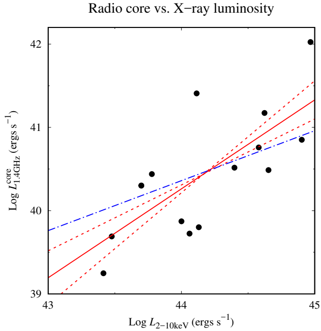
Figure 1. Radio core 1.4-GHz luminosity versus X-ray 2–10 keV luminosity. The red solid line represents a linear fit in the log-log space, while the red dashed lines correspond to the 90 per cent error on the slope and normalization. The blue dot-dashed line represents the relation of Merloni et al. (2003) for a black hole mass of 10^8 solar masses.
