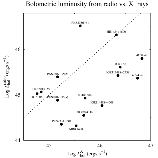
Figure 2. Bolometric luminosity estimated from the radio luminosity of the lobes (y-axis) versus that estimated from the 2–10 keV luminosity (x-axis). The dashed line represents the identity y = x .
