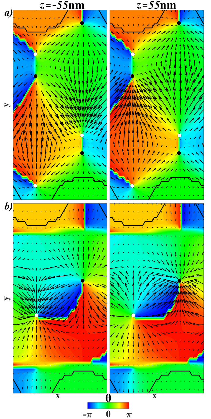
FIG. 7. The SAM density projected on the xy -plane at z = \pm t/4 for the TE_1^+ (a) and TE_1^- (b) modes. The projection is represented by the black arrows, the phase pattern of the magnetic fields \theta by the colored plot and topological charges l = \pm 1 by white and black circles respectively.
