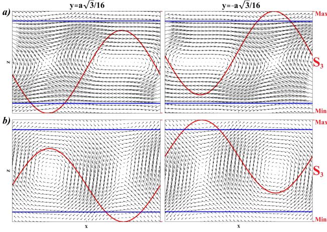
FIG. 9. The OAM density of the TE_1^+ (a) and TE_1^- (b) modes in the xz -plane represented by black arrows and superimposed on the Stokes Parameter S_3(x,y,0) plotted in red for y = \pm a\sqrt{3}/16 . The structure is outlined by blue lines.
