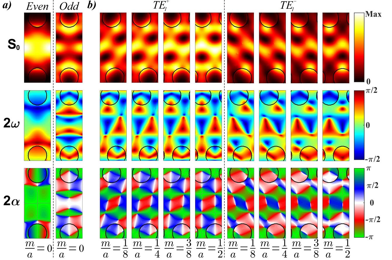
FIG. 4. Polarization characteristics of the pair-wise modes in the symmorphic structure (a) and of the TE_1^+ and TE_1^- modes for different m (b). The top panels represent the Stokes parameter S_0 which is normalized with respect to the highest field intensity in each graph. The middle and bottom panels describe the angles 2\omega and 2\alpha within the PCW unit-cell respectively.
