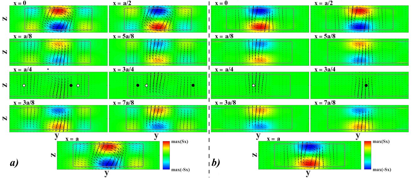
FIG. 6. SAM density of the TE_1^+ (a) and TE_1^- (b) modes along the propagation direction at different x positions in the unit-cell. The arrows describe the components S_y and S_z transverse to the propagation while the colored plot represents the longitudinal component S_x . The vortices centers with topological charges l = \pm 1 are represented by white and black circles respectively.
