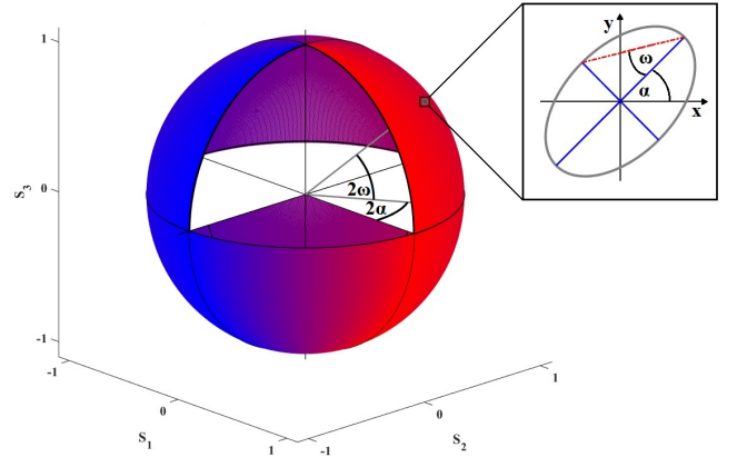
FIG. 3. The Poincaré sphere can be represented with the Stokes parameters S_1, S_2 and S_3 in the Cartesian coordinate system or in the spherical coordinate system with the angles \alpha and \omega , parametrizing the polarization ellipse (inset), times a factor 2.
