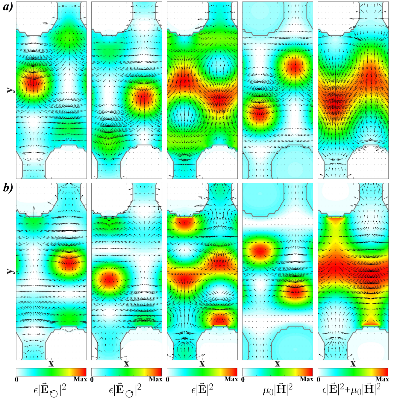
FIG. 8. The linear AM density components of the TE_1^+ (a) and TE_1^- (b) modes represented by black arrows and superimposed on the energy density profiles from left to right: the LCP contributions, the RCP contributions of the electric field, the total electric fields, the magnetic fields and the total electromagnetic fields.
