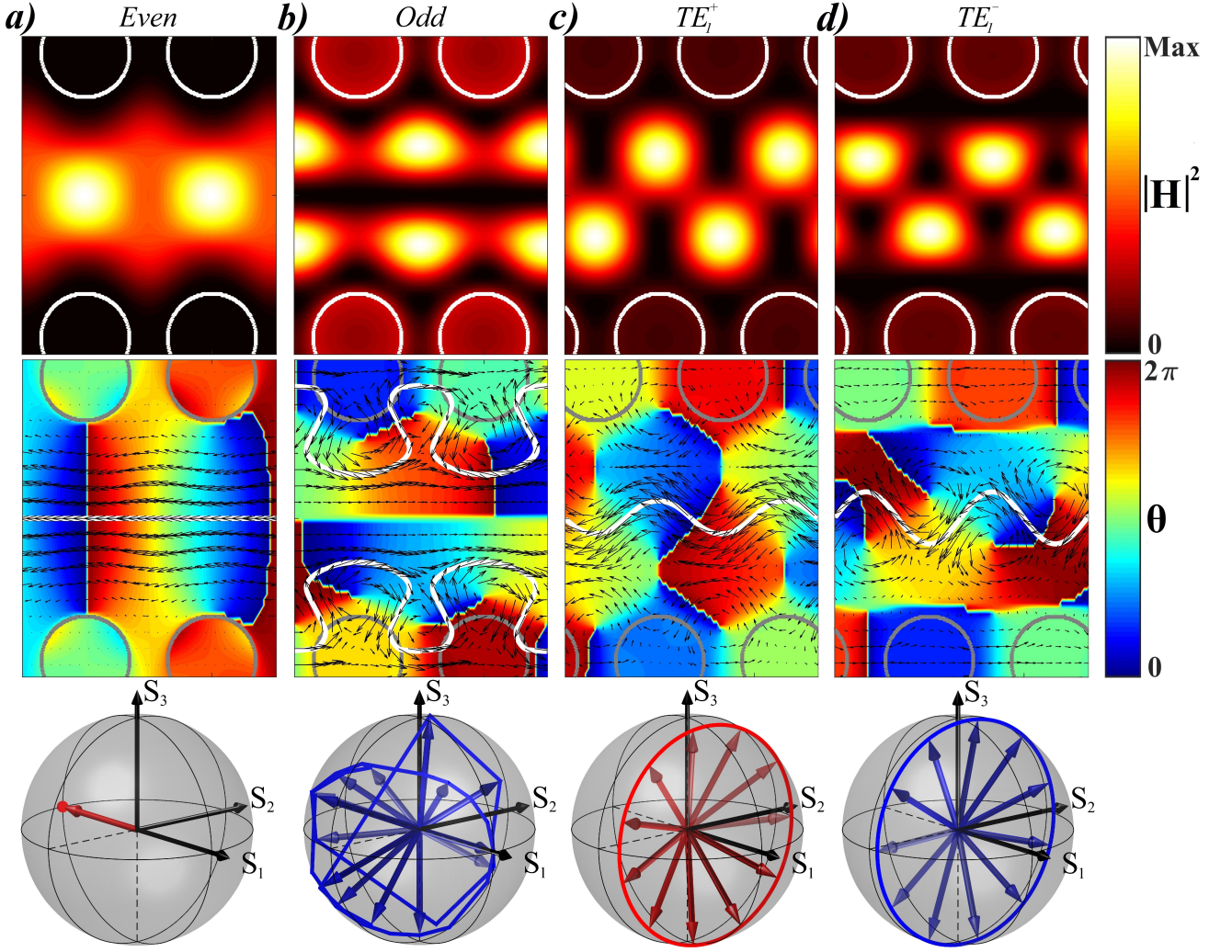
FIG. 5. Magnetic Field properties of the even (a), odd (b), TE_1^+ (c) and TE_1^- (d) modes in the plane of symmetry of the PCWs. The top panels represent the magnetic field intensity of the modes |H|^2 . On the middle panels, the phase patterns \theta of the modes are represented by the contour plots on which the black arrows, corresponding to the Poynting vector \vec{P} , have been superimposed. The white lines are the major energy streamlines. The polarization along these streamlines has been plotted on the Poincaré sphere in the bottom panel of the relevant figures. The opacity of the polarization vector increases along the propagation. For simplicity, only the streamline in the upper part of the PCW ( y > 0 ) is represented for the odd mode (b).
