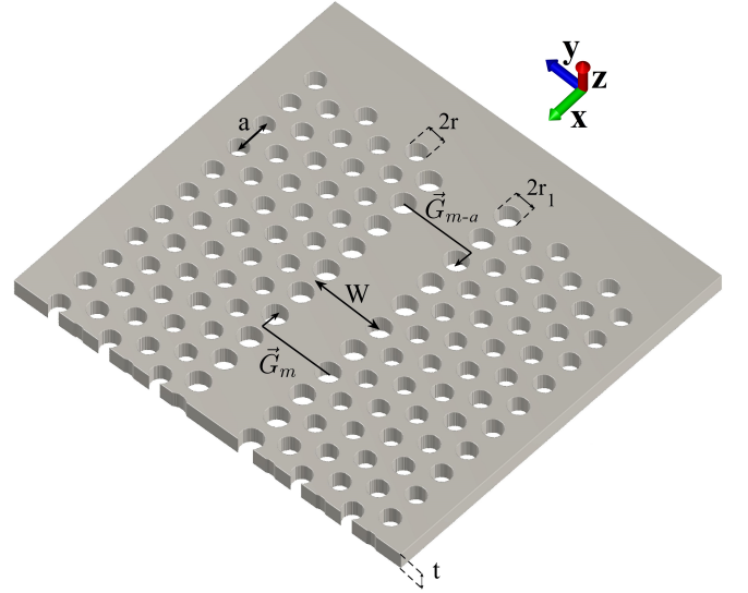
FIG. 1. The PhC is an hexagonal lattice of period a = 0.415\text{nm} patterned with holes of radii r = 0.3a in a Si slab of thickness t=220\text{nm} . The waveguide has a width W = 1.3\sqrt{3}a and the first rows of holes have a modified radius of r_1 = 0.35a . One side of the PhC is shifted along the propagation direction by an offset m with respect to the other, such as the mirror symmetry is replaced by the glide-plane axis \vec{G}_m and \vec{G}_{m-a} .
