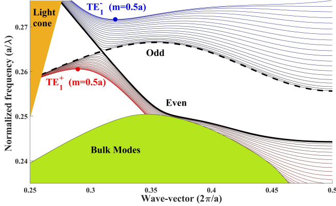
FIG. 2. Bandstructures of the PCW for different offset m between the two side of the PhC. The PhC bulk modes are represented in green and the light-cone in orange. The dispersion relation for the symmorphic structure ( m=0 ) is represented in dashed and full black lines for the odd and even modes respectively. The offset couples the odd and even modes which gives rise to the TE_1^+ and TE_1^- modes in shades of red and blue respectively. These modes are represented in red and blue for the maximum offset m = 0.5a and their anomalous ZGV points are represented with red and blue circles respectively.
