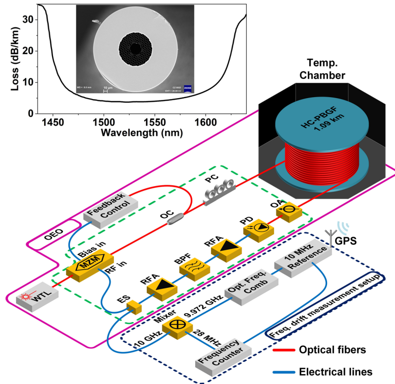
Figure 3. Experimental setup of the OEO. The oscillator cavity consists of the length of HC-PBGF (end face and spectral transmission characteristics shown in inset) placed in a thermally-controlled chamber and with the remaining components (inside the green-dashed-border) being thermally shielded. The blue-dot-bordered part is dedicated to generating a stable 9.972-GHz RF signal reference and using it to measure the OEO frequency drift. WTL: Wavelength-tunable laser; MZM: Mach-Zehnder amplitude modulator; OC: Optical coupler; PC: Polarization controller; OA: Optical Attenuator; PD: Photodiode; RFA: RF amplification; BPF: Band-pass filter; ES: RF splitter; GPS: Global positioning system.
