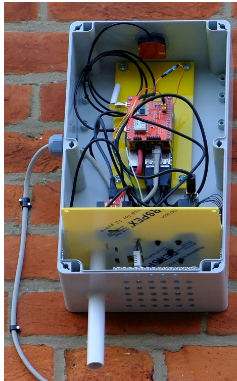
Figure 2. Version 1 of the Air Quality (AQ) Internet of Things (IoT) device, without the enclosure lid; installed on an external wall.
