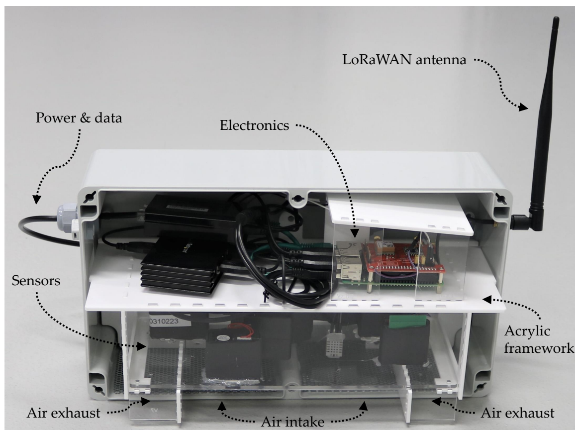
Figure 6. Version 2 of the Air Quality (AQ) Internet of Things (IoT) device in a landscape orientation with the enclosure lid removed. The acrylic framework comprises of i) the electronics section containing a Raspberry Pi 3, Dragino LoRaWAN Hardware Attached on Top (HAT) and power distribution hardware; ii) the sensor housing containing five Particulate Matter (PM) sensors, one temperature & humidity sensor and; iii) the air intake and exhaust, separated by the two vertical acrylic partitions.
