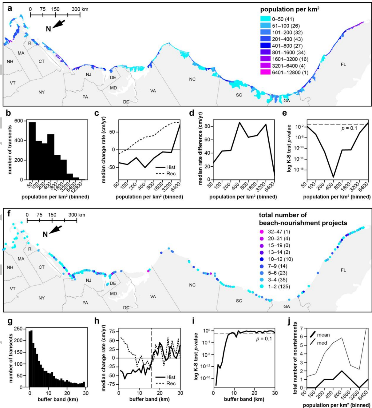
Figure 3. (a) Map of population density (population per km 2 ) for coastal ZIP Code zones along the U.S. Atlantic Coast. (b) Histogram showing the distribution of transects versus population density (binned). (c) Median historical and recent erosion rates (cm/yr) and (d) the difference between them versus population density. (e) Plot of p -values from a Kolmogorov-Smirnov test of historical versus recent erosion rates for transects within each population density; values below the dotted line are significant (the relative distributions are quantifiably different from each other) at p < 0.1 . (f) Map of total number of beach-nourishment projects since 1960 at sites along the U.S. Atlantic Coast. (g) Histogram showing distribution of transects
