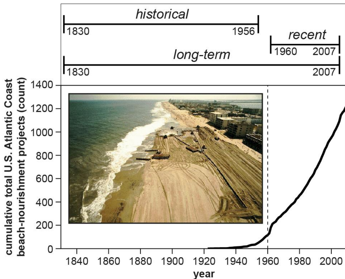
Figure 1. Ranges of survey dates used to calculate historical, recent, and long-term rates of shoreline change (see also Fig. S1), with the cumulative number of nourishment projects along the U.S. Atlantic Coast plotted over time. Dashed vertical line marks 1960. Inset photo shows an oblique aerial view of a beach-nourishment project (courtesy of NOAA).
