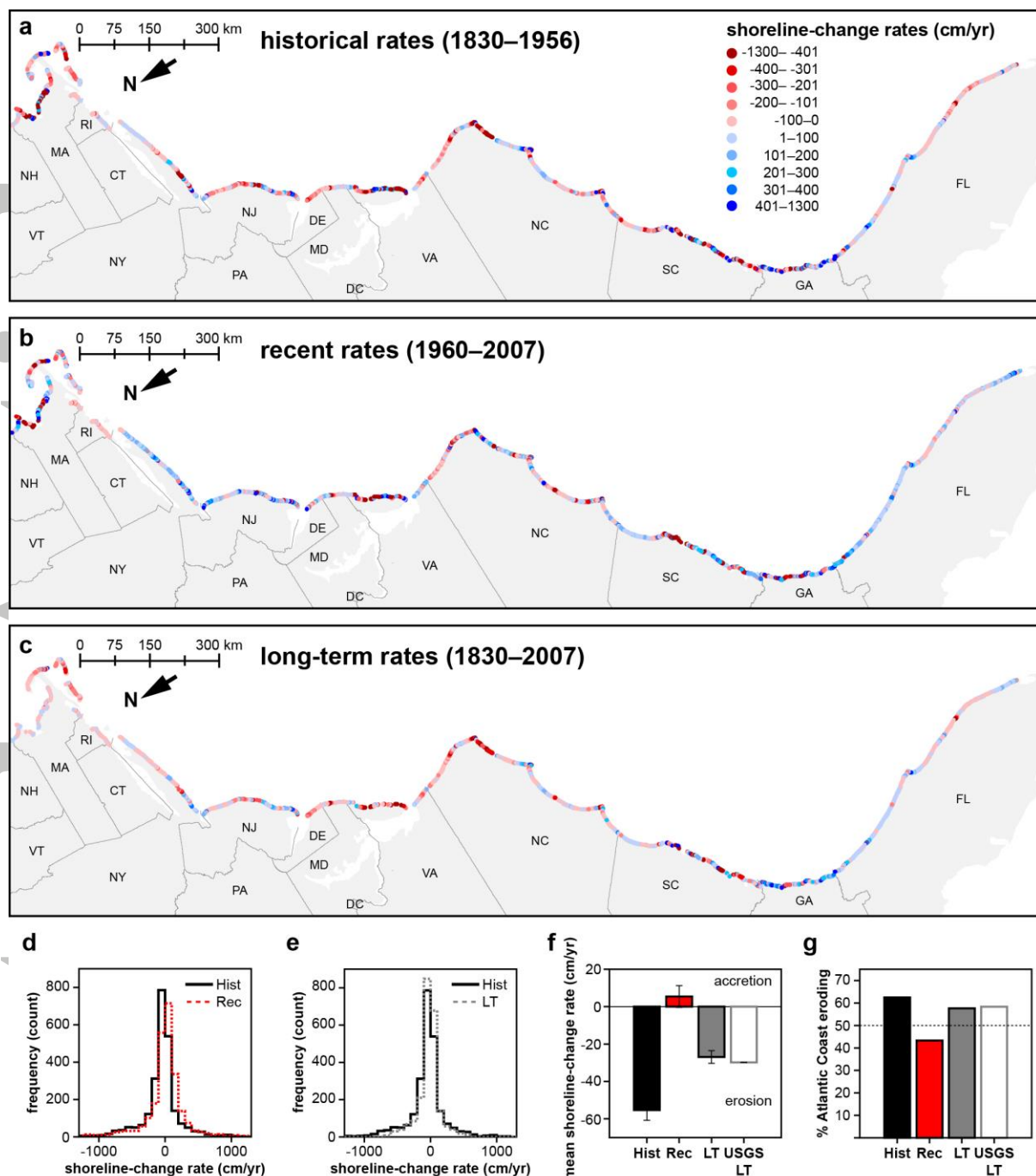
Figure 2. (a) Historical, (b) recent, and (c) long-term rates of shoreline change along the U.S. Atlantic Coast. Color represents the rate (cm/yr) at each 1 km alongshore. (Rates are also detailed in Fig. S2.) Histograms show the relative distributions of (d) historical (black, solid) versus recent (red, dotted) rates, and (e) historical (black, solid) versus long-term rates (gray, dotted). Bar charts compare historical, recent, long-term, and USGS long-term rates, for (f) mean erosion rate (cm/yr; whiskers \pm 1 standard error of the mean), and (g) the percentage of the U.S. Atlantic Coast that is eroding. (Descriptive statistics are listed in Table S2.)
