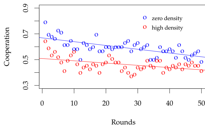
Figure 1. Cooperation variable calculated as the average cooperation per group per round. Zero density condition promotes cooperation compared to high density groups. The fraction of subjects cooperating in each round is shown averaged over groups, for the zero (blue circles) and high (red circles) density conditions.
