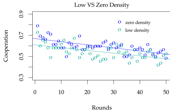
Figure 2. Cooperation variable calculated as the average cooperation per group per round. Cooperation in the zero and low density conditions is not significantly different, but we can observe an overall lower level of cooperation in the low density groups, compared to the zero density one. The fraction of subjects cooperating in each round is shown averaged over groups, for the zero (blue circles) and low (red circles) density conditions.
