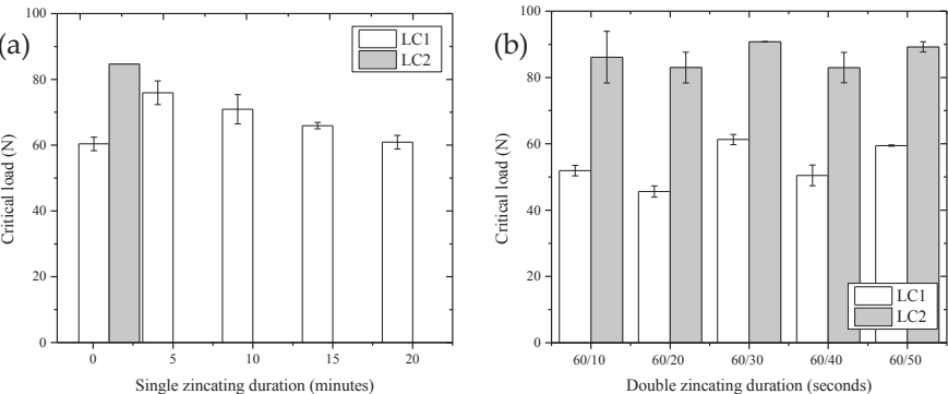
Figure 8: Average critical loads of nickel electrodeposited on AA7075 produced at various (a) single and (b) double zincating durations
