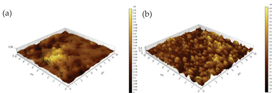
Figure 2: AFM images of AA7075 substrate after (a) conventional single zincating process at 1 minute and (b) modified single zincating process at 20 minutes
