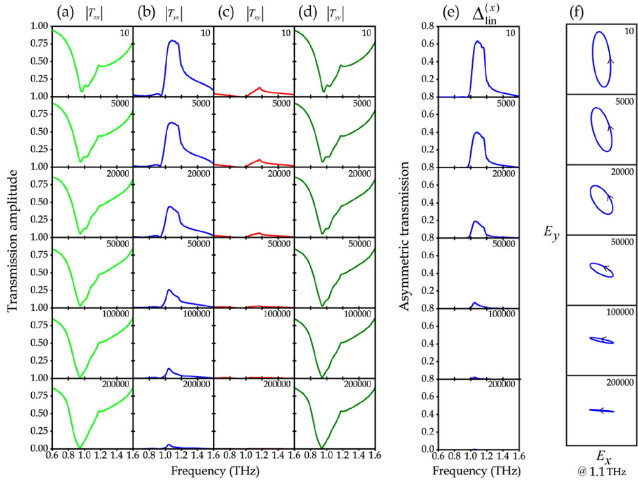
Figure 4. Simulated frequency dependence of co- and cross-polarized transmission amplitudes for x - and y -polarized waves incident on the metamaterial's front with VO 2 conductivity ranging from 10 S/m to 200000 S/m. Columns (a), (b), (c), and (d) show |T_{xx}| , |T_{yx}| , |T_{xy}| , and |T_{yy}| respectively. (e) Frequency dependence of the asymmetric transmission parameter for linearly polarized waves, and (f) transmitted polarization state at 1.1 THz for incident x -polarization.
