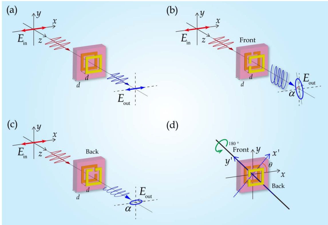
Figure 2. Metamaterial unit cells exhibiting symmetric and asymmetric transmission. (a) A unit cell with two identical metallic square rings on both sides of a dielectric spacer, where the two square rings are aligned along the z direction, transmits electromagnetic waves symmetrically. (b, c) Illumination of (b) front and (c) back of the unit cell for the proposed asymmetric transmission metamaterial composed of two 90^\circ -twisted structurally identical SRRs separated by a dielectric spacer. 19, 20 Illumination of the back of the sample is achieved by rotating the sample by 180^\circ around the y axis. (d) Illustration of the asymmetric transmission metamaterial's axis of twofold rotational symmetry.
