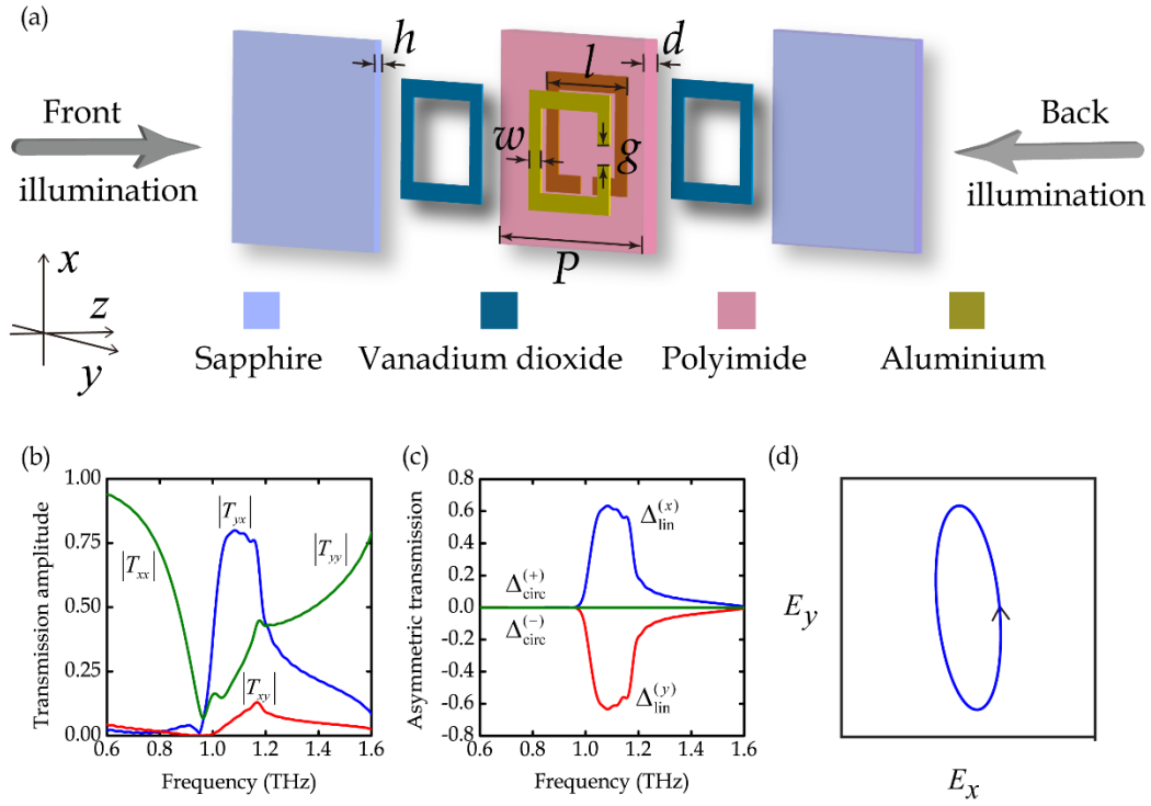
Figure 3. Metamaterial structure and simulated electromagnetic properties at room temperature. (a) Schematic of the unit cell exhibiting asymmetric transmission of linearly polarized waves, with parameters g = 5 \mu\text{m} , w = 8 \mu\text{m} , l = 49 \mu\text{m} , d = 11 \mu\text{m} , h = 500 \mu\text{m} and P = 82 \mu\text{m} . (b) Co- and cross-polarized spectral response |T_{xx}| , |T_{yx}| , |T_{xy}| , and |T_{yy}| of the metamaterial, where T_{ij} represents the transmission coefficient describing i -polarized transmitted waves resulting from j -polarized illumination of the metamaterial's front. (c) Asymmetric transmission for linearly and circularly polarized incident waves, where '-' and '+' correspond to left- and right-handed circularly polarized waves. (d) Polarization ellipse of the transmitted wave at 1.1 THz for x -polarized illumination of the metamaterial's front.
