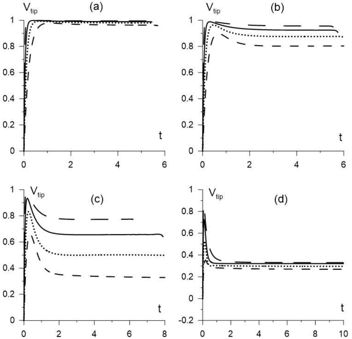
FIG. 6. The velocity of the meniscus's tip for the numerical runs with M = 10^{-1} (a), M = 10^{-2} (b), M = 10^{-3} (c), and M = 10^{-4} (d). The other parameters are Pe = 10^4 , Cn = 4 \cdot 10^{-4} , and different Reynolds numbers, Re = 0.25 (long-dashed lines), Re = 0.5 (solid lines), Re = 1 (dotted lines), and Re = 2 (dashed lines).
