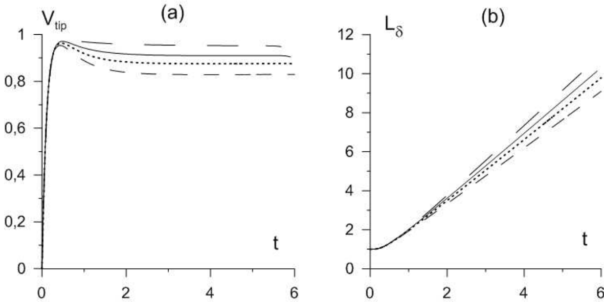
FIG. 2. (a) The velocity of the tip of the liquid/liquid meniscus and (b) the length of the meniscus vs. time. The data are obtained for Pe = 10^4 , Re = 1 , M = 10^{-2} for different Cahn numbers (different interface thicknesses, as \delta = \sqrt{2Cn} ) Cn = 5 \cdot 10^{-5} (long-dashed lines), Cn = 2 \cdot 10^{-4} (solid lines), Cn = 4 \cdot 10^{-4} (dotted lines), and Cn = 8 \cdot 10^{-4} (dashed lines).
