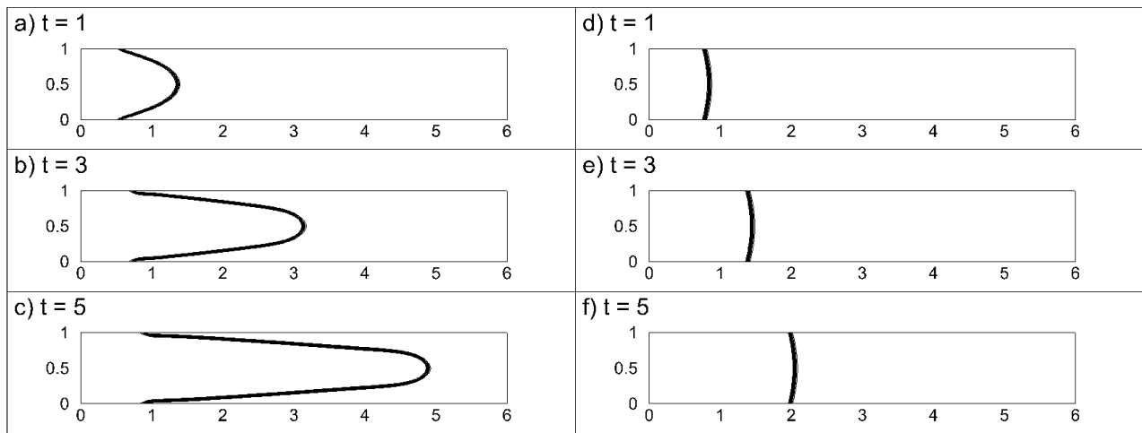
FIG. 3. The typical fields of concentration for different time moments. The data are obtained for Pe = 10^4 , Cn = 4 \cdot 10^{-4} , Re = 1 , and two different Mach numbers, M = 10^{-2} (a,b,c) and M = 10^{-4} (d,e,f).
