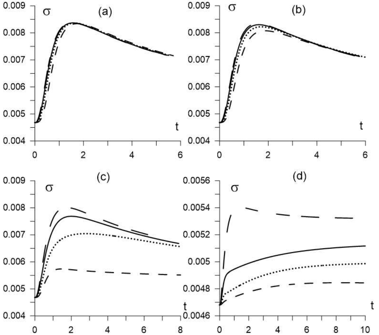
FIG. 11. The time evolution of the surface tension coefficient. The parameters are the same as in figure 6.
