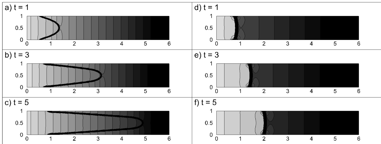
FIG. 4. The typical fields of pressure for different time moments. All parameters as in Figure 3.
