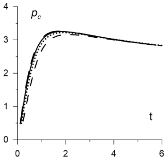
FIG. 14. The capillary pressure as calculated from equation (23) vs. time. The curves are plotted for M = 10^{-2} and other parameters as in figure 6.
