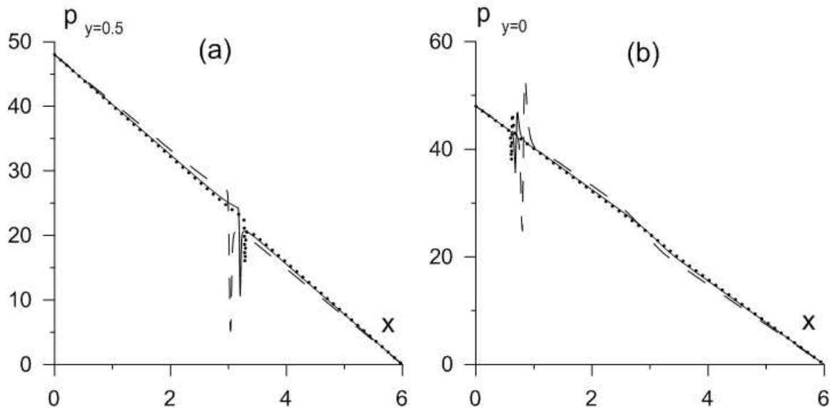
FIG. 10. The pressure profiles along the centreline and along the wall for M = 0.01 , Re = 1 , Pe = 10^4 and three different Cahn numbers, Cn = 8 \cdot 10^4 (dashed line), Cn = 2 \cdot 10^4 (solid line) and Cn = 5 \cdot 10^5 (dotted line). The profiles are shown for t = 3 .
