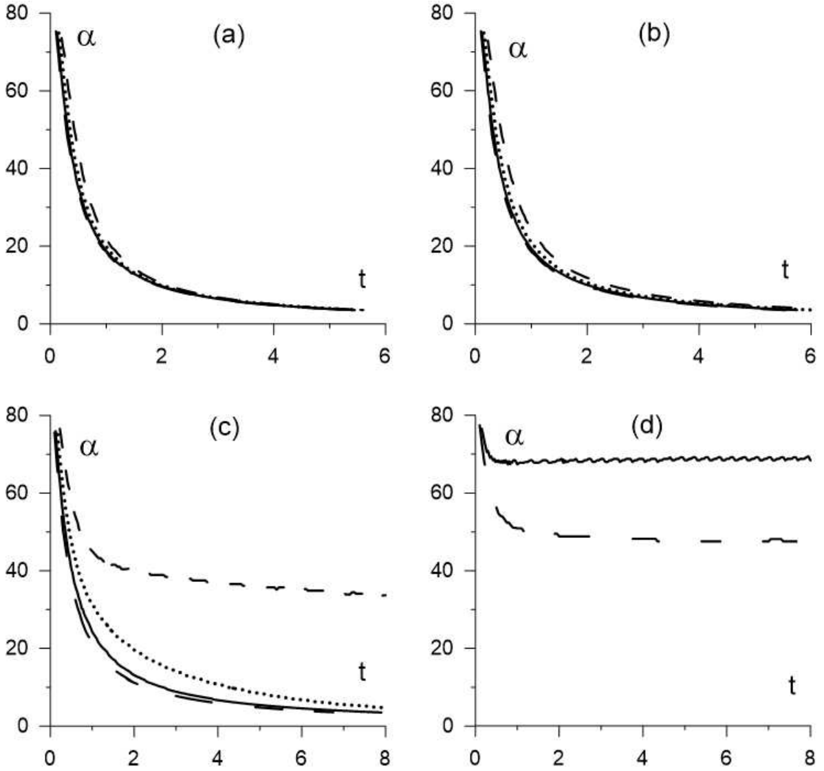
FIG. 12. The time evolution of the dynamic contact angle. The parameters are the same as in figure 6. In (d), only two curves are shown for Re = 0.25 and Re = 0.5 , as the adopted algorithm for calculations of the contact angle generates too noisy results for higher Reynolds numbers.
