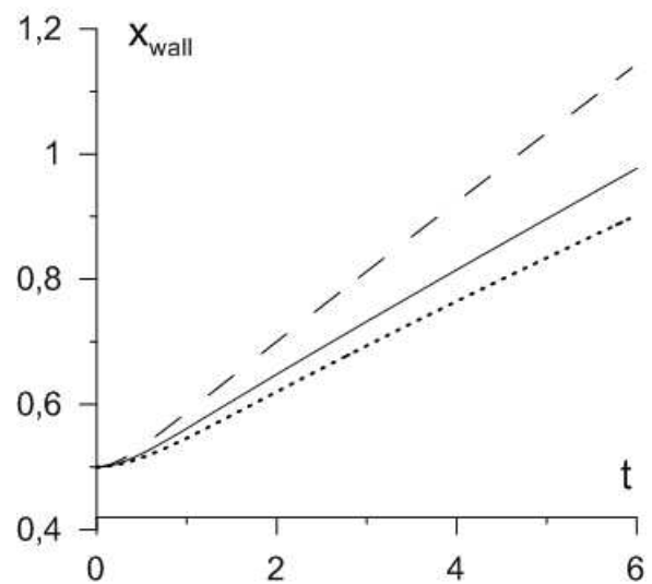
FIG. 15. The position of a meniscus on a wall vs. time. The curves are plotted for M = 10^{-2} , Re = 1 , Cn = 4 \cdot 10^{-4} and three different Peclet numbers, Pe = 10^3 (dashed line), Pe = 10^4 (solid line), and Pe = 10^5 (dotted line).
