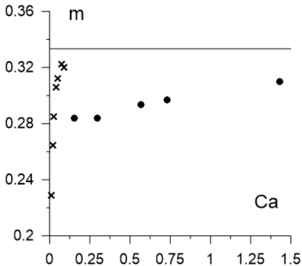
FIG. 13. The mass fraction (20) vs. capillary number. The results are shown for Pe = 10^4 , Cn = 4 \cdot 10^{-4} , and different Reynolds numbers. Circles correspond to the fingering displacement, and crosses depict the piston-like displacements.
