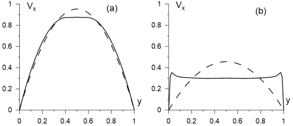
FIG. 8. The profiles of the x -component of the velocity across the tube at the points of the meniscus' tip (solid lines) and near the inlet/outlet (dashed lines). The data are obtained for for t = 3 , Pe = 10^4 , Re = 1 , Cn = 4 \cdot 10^{-4} , and two different Mach numbers, M = 10^{-2} (a) and M = 10^{-4} (b).
