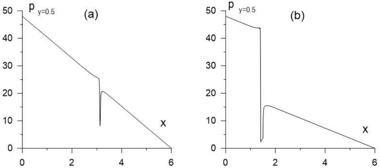
FIG. 9. The profiles of the pressure along the centreline of the tube. The parameters are the same as in figure 8.
