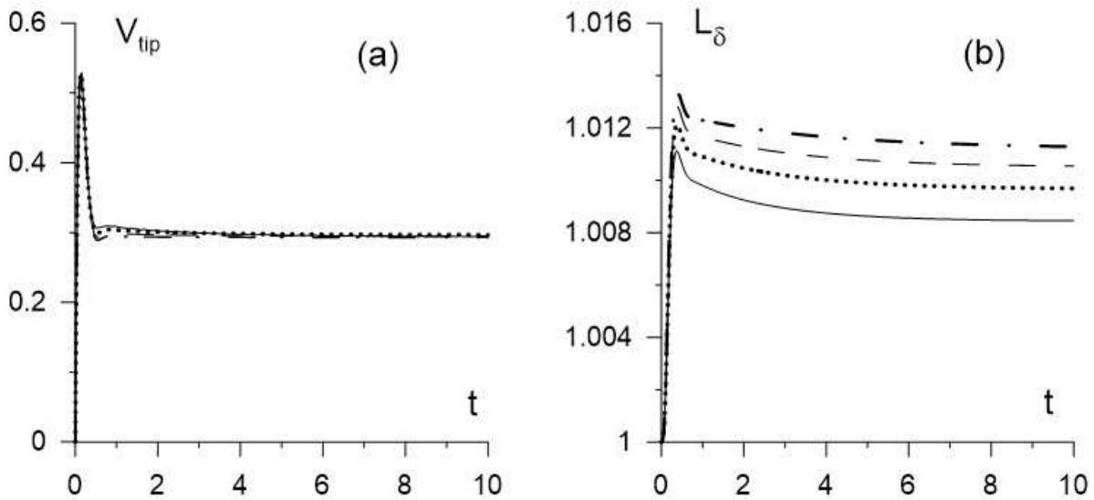
FIG. 1. (a) The velocity of the tip of the liquid/liquid meniscus and (b) the length of the meniscus vs. time. The data are obtained for Pe = 10^4 , Cn = 4 \cdot 10^{-4} , Re = 1 , M = 10^{-4} using the numerical grids with the grid size of 1/250 (solid lines), 1/300 (dotted lines), 1/350 (dashed lines), and 1/400 (dash-dotted lines).
