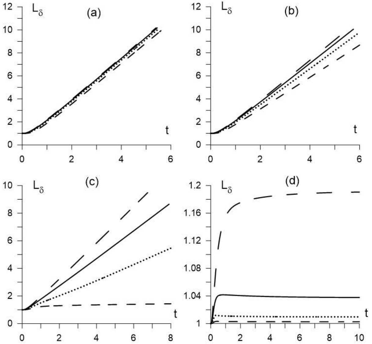
FIG. 7. The time changes of the meniscus' length. The parameters are the same as in figure 6.
