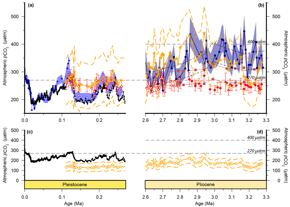
Figure 6. Cell size corrections to \text{CO}_2(\epsilon_{\text{p-alk}}) . Ornamentation is the same as Fig. 1, with the addition of cell-size-corrected \text{CO}_2(\epsilon_{\text{p-alk}}) . The smaller liths than modern E. huxleyii across all of our records mean that a direct application of the method of Henderiks and Pagani (2007) results in substantially lower \text{CO}_2(\epsilon_{\text{p-alk}}) throughout (open orange stars; c , d ). As the main interest is in the effect of the Plio-Pleistocene change in cell size we observe, we adjusted the b' term so that \text{CO}_2(\epsilon_{\text{p-alk}}) matched our uncorrected \text{CO}_2(\epsilon_{\text{p-alk}}) record during the last interglacial (filled orange stars; a , b ).
