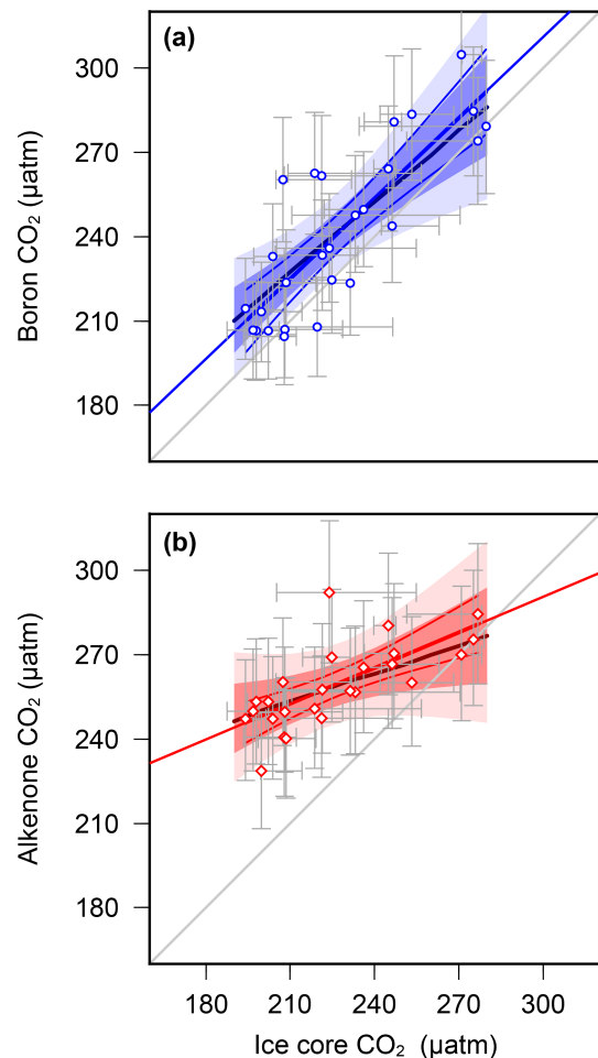
Figure 5. Regression analyses of proxy-based p\text{CO}_2 with ice core data (a) \text{CO}_2(\delta^{11}\text{Bplank}) (Chalk et al., 2017) and (b) \text{CO}_2(\epsilon_p\text{-alk}) vs. ice core data (Bereiter et al., 2015 and Table 1) for MIS5–8, interpolated in the age domain. Regression lines (in red/blue) are linear fits with 68 % and 95 % confidence intervals, calculated by bootstrapping the uncertainties in proxy p\text{CO}_2 (Monte Carlo method described in the methods section). Uncertainty in the ice core values is by estimated by applying a 3000 uncertainty in the age model during interpolation. Uncertainty envelopes considering data points alone (no bootstrap) are solid lines, with p_{\text{max}} regressions in the thicker, darker colours. A 1 : 1 line is shown in grey for comparison. Statistical calculations were performed in R (R Core Team, 2015).
