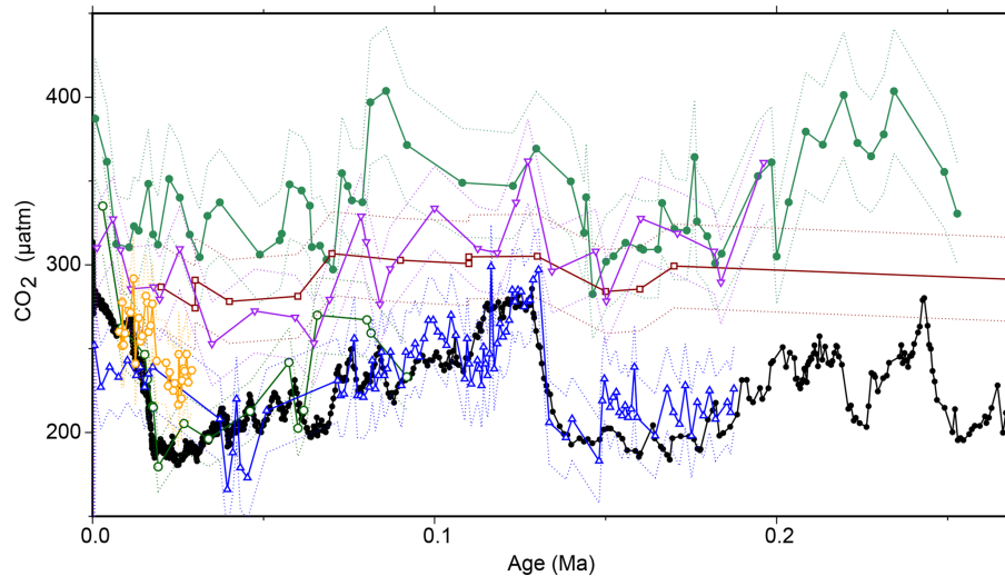
Figure 7. Recalculated \text{CO}_2(\varepsilon_{\text{p-alk}}) . Previous work (Jasper and Hayes, 1990; Jasper et al., 1994) calculated \text{CO}_2(\varepsilon_{\text{p-alk}}) using a different model; here, we recalculate the earlier work using the modern methodology and Monte Carlo propagation applied to our other sites. All previous records have been recalculated using the same methodology as our new record, with some corrections and adjustments (for example, for growth rate or lith size) removed to allow direct comparisons. Records are from MANOP site C from the central equatorial Pacific ( 0^{\circ}57.2' \text{ N} , 138^{\circ}57.3' \text{ W} ; filled green circles; Jasper et al., 1994), DSDP Site 619 in the Pigmy Basin, northern Gulf of Mexico ( 27^{\circ}11.6' \text{ N} , 91^{\circ}24.5' \text{ W} ; open green circles; Jasper and Hayes, 1990), site 05PC-21 from the Sea of Japan ( 38.40^{\circ} \text{ N} , 131.55^{\circ} \text{ E} ; open blue triangles; Bae et al., 2015), site NIOP464 in the Arabian Sea ( 22.15^{\circ} \text{ N} , 63.35^{\circ} \text{ E} ; open orange hexagons; Palmer et al., 2010), site GeoB 1016-3 in the Angola Current ( 11.59^{\circ} \text{ S} , 11.70^{\circ} \text{ E} ; inverted purple triangles; Andersen et al., 1999), and ODP Site 925 ( 4^{\circ}12.25' \text{ N} , 43^{\circ}29.33' \text{ W} ; open dark red squares; Zhang et al., 2013). Ice core data are shown as filled black circles and lines (Bereiter et al., 2015 and Table 1). Dashed lines are 2\sigma uncertainties from Monte Carlo error propagation as described elsewhere in the text.
