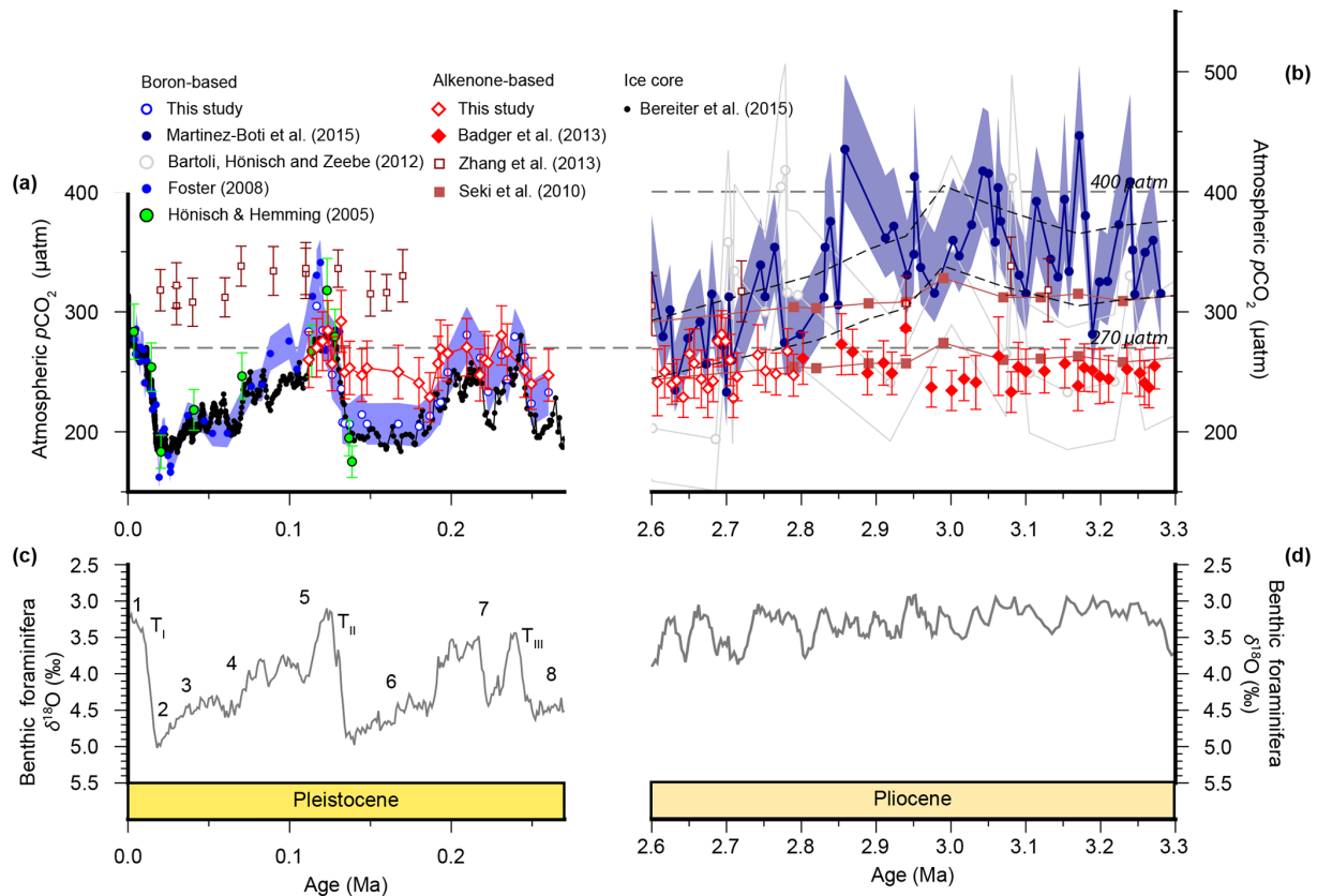
Figure 2. Atmospheric CO 2 reconstructions through the Plio-Pleistocene. (a) Published boron isotope CO 2(δ 11 B plank ) records from ODP Site 999: open blue circles (Chalk et al., 2017), filled bright blue circles (Foster, 2008; recalculated as described in the text), open grey circles (Bartoli et al., 2011), and filled dark blue circles (Martínez-Botí et al., 2015); and Deep Sea Drilling Project (DSDP) Site 668: filled green circles (Hönisch and Hemming, 2005). (b) Published CO 2(ε p-alk ) records from ODP Site 925: open maroon squares (Zhang et al., 2013); ODP Site 999: filled red diamonds (Badger et al., 2013a); and ice core records: filled black squares (Bereiter et al., 2015 and Table 1), as well as our new alkenone isotope records from ODP Site 999 (open red diamonds). The lith size-corrected (dashed black envelope) and uncorrected (solid red envelope) data of Seki et al. (2010) are also shown. All records are shown with 1σ uncertainties as described elsewhere. (c) The benthic foraminiferal stable oxygen isotope stack (Lisiecki and Raymo, 2005) with Marine Isotope Stage (MIS; numerals) and terminations ( T ) indicated.
