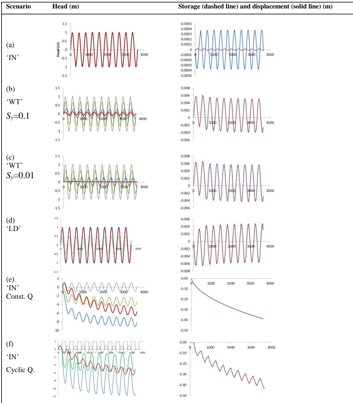
Figure 4. 1D model simulations for the GBM environment, showing results for the scenarios (a) 'IN', (b) 'WT' ( S_y=0.1 ), (c) 'WT' ( S_y=0.01 ), (d) 'LD', (e) 'IN' with constant pumping, (f) 'IN' with cyclic pumping, (see text for explanation). The x-axis is time in days, shown to 10 years (i.e. 3650 days). The amplitudes reported in the text are calculated from the max-min of the last annual cycle. Left: The y-axis is head, in metres (m). The surface head and/or mechanical load boundary conditions (black line) are expressed as equivalent m head (for the WT condition the unit variation of head is given and the S_y variation in mechanical load is not shown); results are in green (30 m depth), blue (100 m depth) and red (300 m depth) in all cases. For (a) results are co-linear at all depths; for (f) the intermittent pumping is shown as off/on by the square-wave dotted line. Right: The y-axis has dimension of length, in metres (m), showing changes in storage (dashed red line) and surface displacement (solid blue line) for each scenario.
