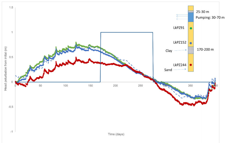
Figure 7. Laksmipur: comparison of observed heads (solid lines) and simulated heads (dashed lines) starting 31 May 2013, for ‘WT’ upper boundary condition ( S_y=0.8 ), for LkPZ91 (green), LkPZ152 (blue) and LkPZ244 (red). X axis is time in days. The surface loading is set equal to the observed head in LkPZ244, and the surface head is set to the observed head in LkPZ244 divided by S_y . The pumping rate is 0.04 \text{ m a}^{-1} for the period shown (1 for ‘on’, 0 for ‘off’).
