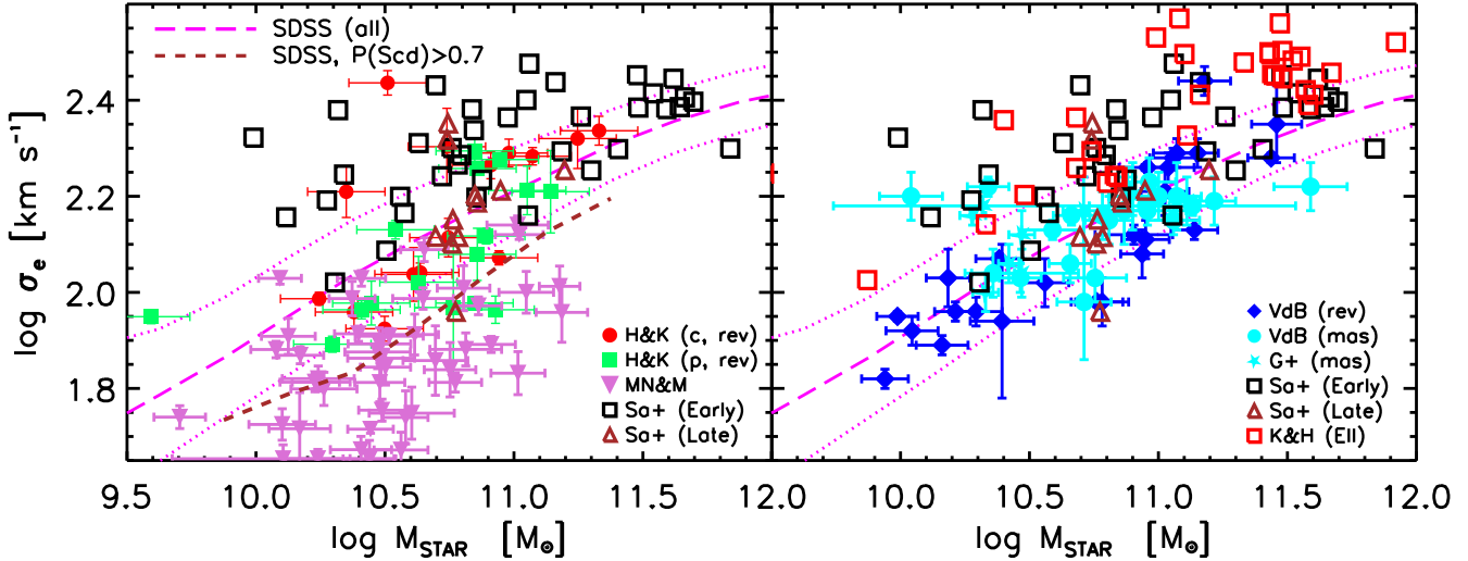
Figure 1. Left: Correlation between velocity dispersion and (total) stellar mass in SDSS for all galaxies (long-dashed magenta line; the dotted magenta lines show the region enclosing 68% of the objects at each M_{\text{star}} ) and also for later-type galaxies with a high probability P(\text{Scd}) > 0.7 of being classified as late spirals (brown dashed line). The data are the classical and pseudobulges from Ho & Kim (2014, red circles and green squares), and the low-mass Seyferts from Martín-Navarro & Mezcua (2018, orchid upside down triangles). Right: Same correlation between velocity dispersion and (total) stellar mass in SDSS for all galaxies, compared to the reverberation-based and masers from van den Bosch (2016, blue diamonds and cyan circles), and the megamasers from Greene et al. (2016, cyan stars). As in the left panel, open black squares and brown triangles are from Savorgnan & Graham (2016), while the open red squares are the elliptical quiescent supermassive black hole sample from Kormendy & Ho (2013). In contrast to the quiescent galaxies, AGN galaxies seem to follow very similar scaling relations to SDSS galaxies. For simplicity, in this and in all subsequent figures, masers are labelled as “mas”, while all other AGN samples with black hole masses based on direct reverberation mapping or reverberation-based (i.e., single-epoch/virial) techniques, are labelled as “rev”.
