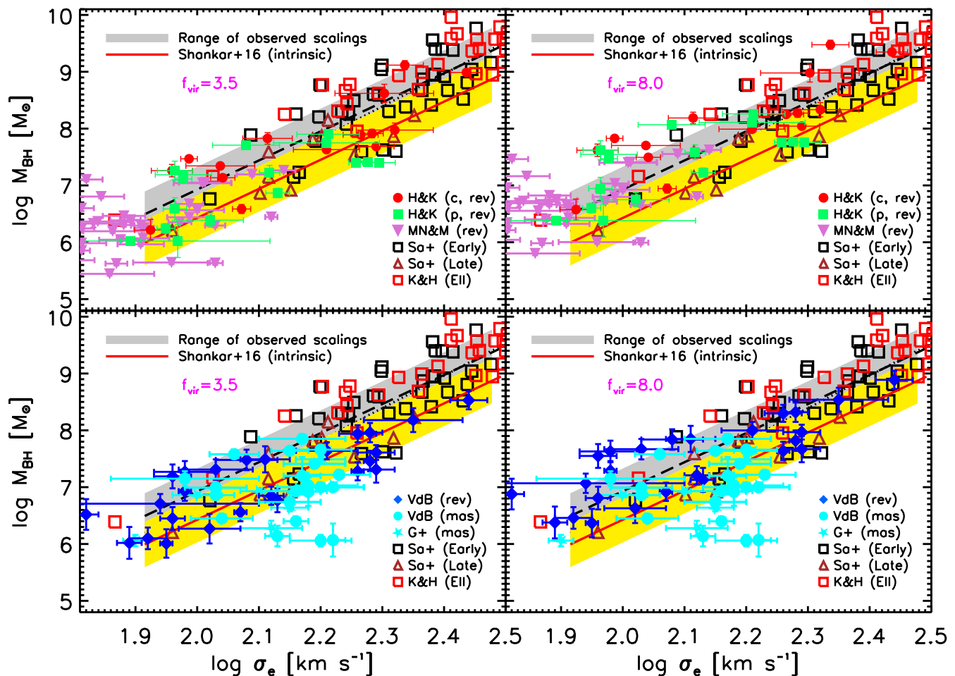
Figure 3. Same format as Figure 2 but for the correlations between M_{\text{bh}}-\sigma in the Savorgnan & Graham (2016) quiescent galaxies (black lines and grey band) and the “intrinsic” (unbiased) M_{\text{bh}}-\sigma relation predicted by Shankar et al. (2016, solid red line and yellow band). When adopting the mean virial factor of f_{\text{vir}} = 3.5 as constrained by Grier et al. (2017), most of the data tend to better line up with the Shankar et al. (2016) “intrinsic/unbiased” M_{\text{bh}}-\sigma relation (left panels), while substantially larger virial factors are required to match the M_{\text{bh}}-\sigma relation of quiescent galaxies (right panels). More quantitative estimates of the appropriate virial scaling factors are given in Figure 4.
