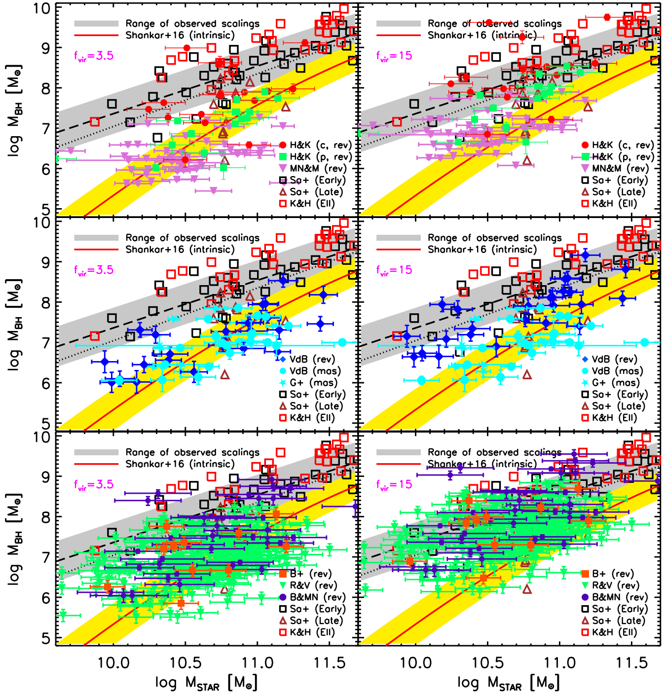
Figure 2. Left panels: Correlations between M_{\text{bh}}-M_{\text{star}} in quiescent galaxies (the black dotted line shows the fit to the all sample; black dashed line and grey band show the fit and rms-scatter for the early-type quiescent galaxies subsample, respectively) with data from Savorgnan & Graham (2016, open black squares and brown triangles) and the ellipticals from Kormendy & Ho (2013, open red squares), and the unbiased M_{\text{bh}}-M_{\text{star}} relation predicted by Shankar et al. (2016, solid red line and yellow band). The correlations are compared with a variety of samples of active galaxies for which a mean virial factor f_{\text{vir}} = 3.5 was used. The samples are from Ho & Kim (2014, red circles and green squares for classical and pseudobulges, respectively), Martín-Navarro & Mezcua (2018, orchid upside down triangles), in the top panel, van den Bosch (2016, blue diamonds and cyan circles), Greene et al. (2016, cyan stars), in the middle panel, and Busch et al. (2014, red squares), Reines & Volonteri (green upside down triangles 2015), and Bentz & Manne-Nicholas (2018, purple circles), in the bottom panel. Right panels: Same format as left panels but adopting a mean virial factor of f_{\text{vir}} = 15 for all virial-based active black hole mass measurements. When adopting the mean virial factor of f_{\text{vir}} = 3.5 as constrained by Grier et al. (2017), most of the active galaxies tend to better line up with the Shankar et al. (2016) “intrinsic/unbiased” M_{\text{bh}}-M_{\text{star}} relation (left panels), while substantially larger virial factors are required to match the M_{\text{bh}}-M_{\text{star}} relation of quiescent galaxies (right panels).
