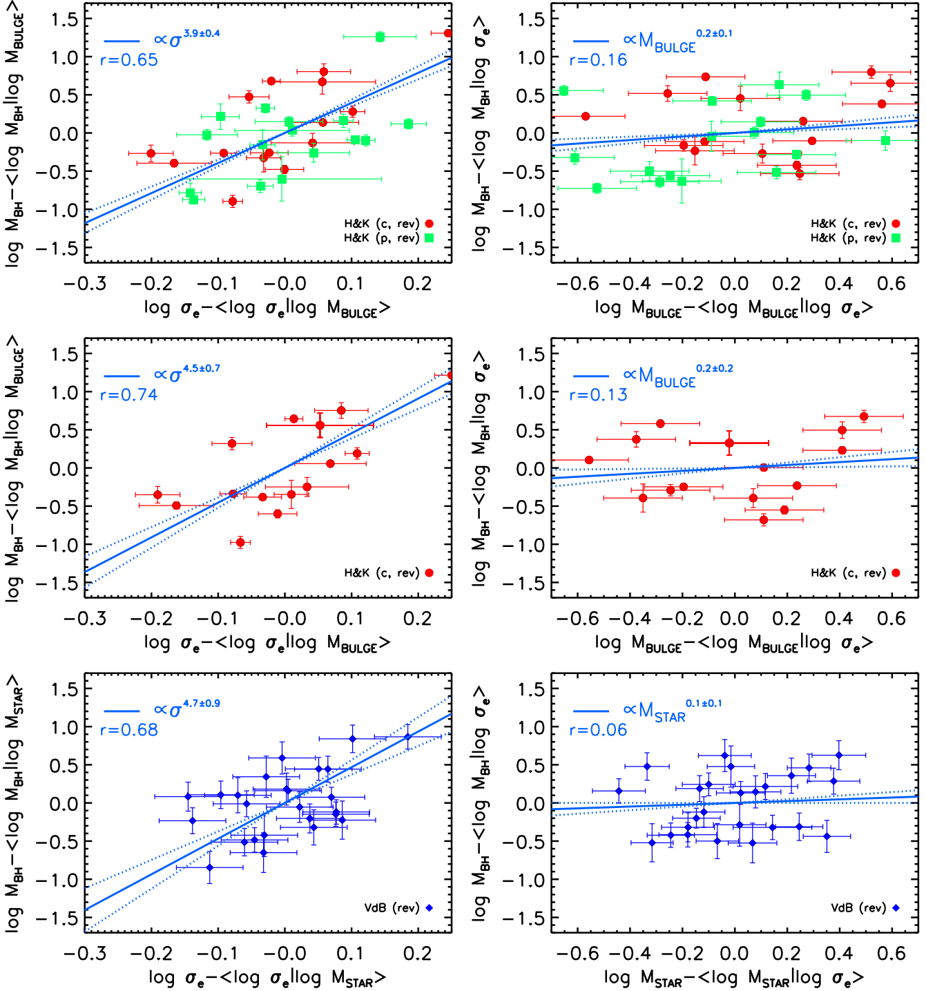
Figure 5. Correlations between residuals from the observed scaling relations, as indicated. Red circles and green squares in the top panels show, respectively, classical and pseudobulges from Ho & Kim (2014). The middle panels show the subsample of classical bulges. The blue filled diamonds in the bottom panels are the reverberation-based data from van den Bosch (2016). Correlations with velocity dispersion appear to be much stronger (left panels; Pearson coefficient r \sim 0.6 - 0.7 ) than those with bulge/total stellar mass (right panels; r \lesssim 0.1 - 0.2 ), in line with that observed for local samples of quiescent supermassive black holes with dynamical mass measurements.
