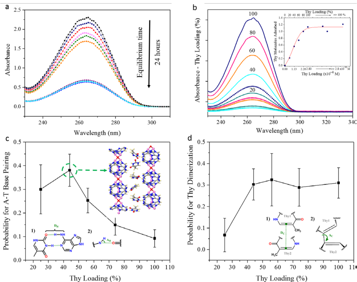
Figure 3. Solution thymine isotherms in SION-19' and probability of Adenine-Thymine pairing and Thymine-dimerization. a) Time dependency for Thy to reach equilibrium when loaded into SION-19', b) Solution isotherms of 20-100% (0.56-2.80 x 10 -4 M) Thy loaded into the pores of SION-19'. Inset: maximum uptake of Thy (~1.1 molecules). Here, multiple Thy concentrations (blue circles – above 100 % loading) were used to determine the saturation limit of Thy into the pores of SION-19'. c) Frequency of observed Ade-Thy base pair formation from MD simulations – Insets 1) and 2) show the metrics used for H-bonding formation between Ade-Thy from the MD simulations and d) the frequency in which Woodward-Hoffmann and Schmidt rules are satisfied for Thy dimerization in the MD simulations at different loadings. Insets 1) and 2) show the metrics used for satisfying the Woodward-Hoffmann and Schmidt rules.
