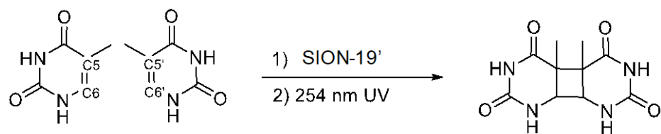
Figure 5: Synthetic conditions utilized for the photodimerization of Thy molecules using SION-19'.
