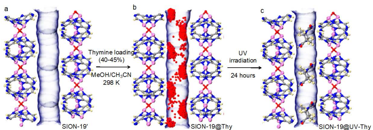
Figure 4. Schematic representation of thymine loading, location and dimerization within SION-19'. a) 1-dimensional base-pore surface for SION-19' prepared using HOLE2, b) Thy snapshots (red dots) from an MD trajectory of 44% thymine loading in the base pore of SION-19. Here, Ade acts as a structure directing agent that 'locks' Thy molecules into positions close enough to another Thy molecule for photodimerization to occur. c) DFT optimized positions of Thy<->Thy dimers arising from a 44% loading of Thy. Atom color code: pink, Zn; red, O; blue, N; grey, C; light yellow, H.
