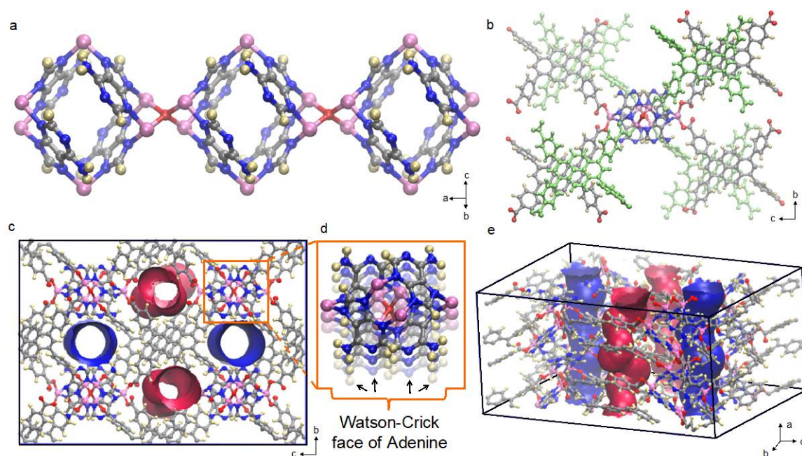
Figure 1. Structural representation of SION-19. a) A Zn II (adeninate) octahedron cage is coordinated to six Zn II ions, four at the corners of the equatorial plane (Zn II eq ), and two at the apical positions (Zn II ap ). The Zn II (adeninate) cages are linked to each other via the Zn II eq to form 1-dimensional columnar building blocks, b) The Zn II (adeninate) columnar building blocks are linked to each other via fully deprotonated TBAPy ligands – grey TBAPy is bound to Zn II ap whereas the lime green is bound to Zn II eq , c-d) Connolly surface representation of SION-19 viewed along the a -axis, revealing that the coordination of TBAPy ligands to the Zn II (adeninate) columns leads in the formation a 3-dimensional structure possessing two distinct types of 1-dimensional pores: the base-pore (blue) and the acid-pore (red). Highlighted in d) are the Watson-Crick faces of Ade which point into the base pore and e) Connolly surface representation of SION-19 in a 3-dimensional view. Atom color code: pink, Zn; red, O; blue, N; grey, C; light yellow, H.
