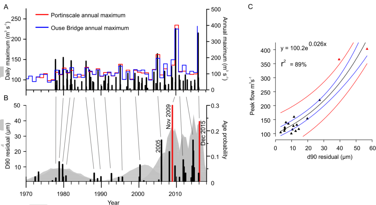
Figure 5. A. Gauged annual maximum (AMAX) river discharges at Portinscale (red line) and Ouse Bridge (blue line) gauging station, alongside daily maximum flow data from Portinscale (black bars) all in \text{m}^3 \text{s}^{-1} . B. D90residual ( \mu\text{m} ) (black bars) and 2 \sigma age probabilities (grey) for sedimentary flood layers. C. Relationship between D90residual ( \mu\text{m} ) and the equivalent gauged peak river flow ( \text{m}^3 \text{s}^{-1} ) for the given year at Portinscale. Shown with 1 sigma (blue) and 2 sigma (red) uncertainties. (Colour version online).
