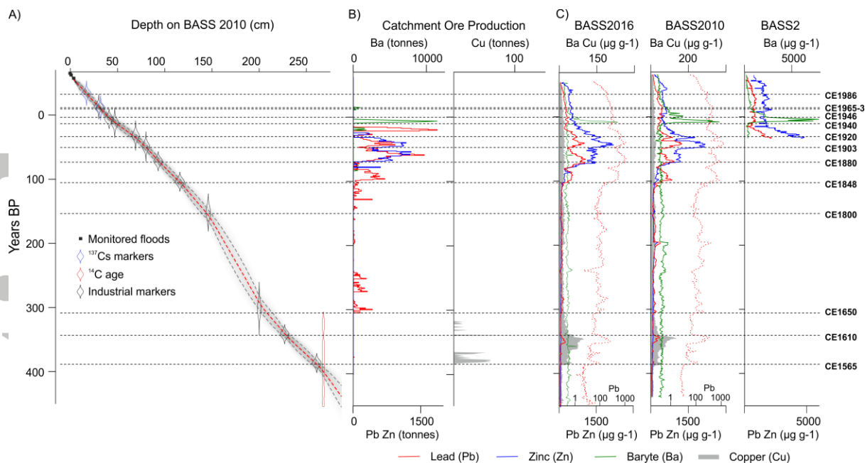
Figure 2. Age-depth information for Bassenthwaite Lake and the metal pollutant stratigraphy.
