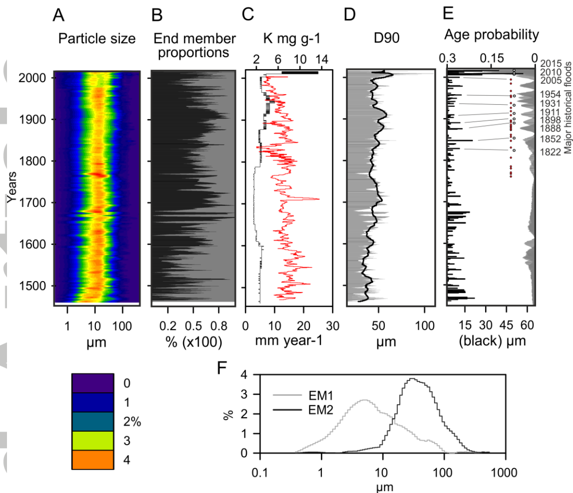
Figure 4. For BASS-2016, A. 3-dimensional colour contour plot of volume percent PSD. B. Proportions of the particle size distributions of end members EM1 and EM2. C. Sedimentation rates (SR) mm year -1 and K concentrations measured by XRF (mg g -1 ). D. 90th percentile (D90; grey) of the PSDs fitted with a 25-period centrally weighted smoothing function (D90smoothed; black). E. The positive D90 residuals (black line: D90 minus D90smoothed) and 2 \sigma age probabilities for flood layers ( >115 \text{ m}^3 \text{ s}^{-1} ) showing major and minor floods from the Chronology of British Hydrological Events entries for the Derwent/Cocker catchment ( http://www.cbhe.hydrology.org.uk/ ) (Black and Law, 2004). F. PSDs of the statistically significant particle size end members. (Colour version online).
