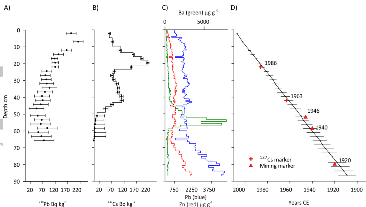
Figure 3. Age depth information for BASS-2 showing: A) supported ^{210}\text{Pb} records, B) ^{137}\text{Cs} records, C) dry mass elements concentrations of Pb, Zn and Ba measured by XRF, D) ^{210}\text{Pb} age-depth model compared with mining and artificial radionuclide ( ^{137}\text{Cs} ) markers.
