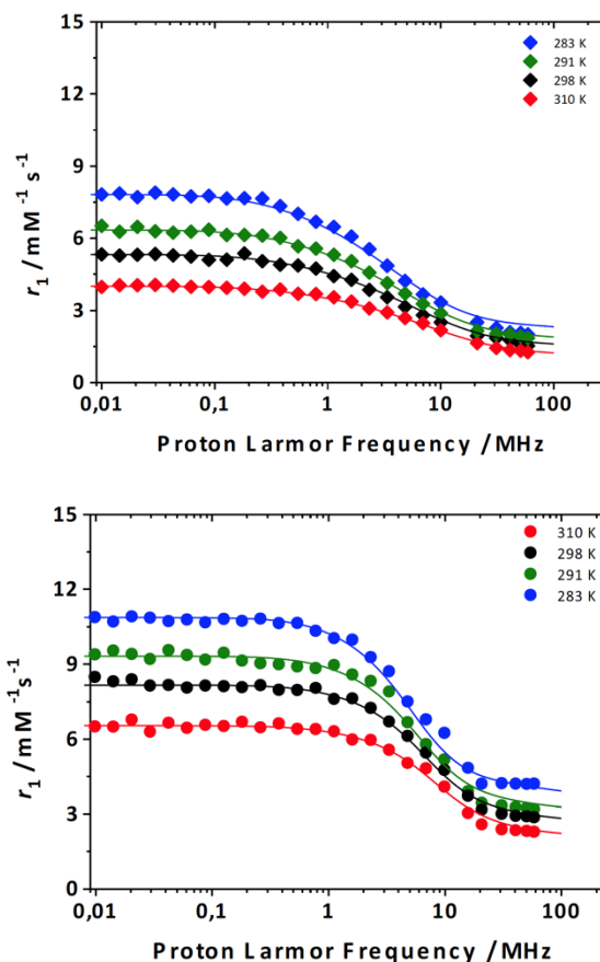
Figure 7 1 H NMRD profiles of [Gd.L 1 ] (0.34 mM; pH 6.9) – top, and [Gd.L 3 ]Cl 3 (0.59 mM; pH 6.4) – bottom measured at different temperatures (283, 291, 298 and 310 K). The curves were calculated with the parameters shown in Table 2.
