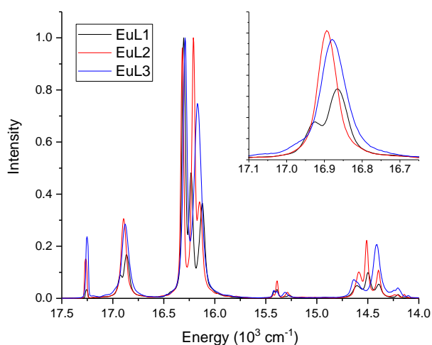
Figure 2 Room temperature emission spectra of [Eu.L 1 ], [Eu.L 2 ] and [Eu.L 3 ] 3+ in methanol, showing the splitting of the \Delta J = 1 manifold (inset). These spectra are quite different in water, where the ligand field splitting of [Eu.L 1 ] for example, is exactly half of that observed in methanol. 12
