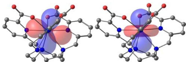
Figure 5 Comparison of the PCS field 200 ppm iso-surfaces (blue – negative shift, red – positive shift) for the DFT optimised structures of [Yb.L1] 3 ; (left) without symmetry constraint and (right) the symmetrised one. Images were generated with Chemcraft software.
