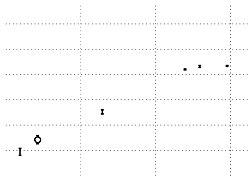
Figure 4 Axiality of the magnetic susceptibility tensor ( \text{Å}^3 \text{ SI units} ), extracted from the room temperature ^1\text{H} NMR spectra, plotted against the Bleaney constant C_i for each lanthanide. A linear fit, predicted by Bleaney's model (line), shows a rather poor correlation with the experimental data (circles).
