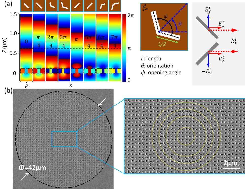
FIG. 2. (a) Eight V-shaped metamolecules of different size, opening angle and orientation providing different levels of phase retardation, from 0 to 7\pi/4 (dashed reference line), were used in the lens design. FDTD simulations show phase distributions in the light scattered by the metamolecules located in the positions indicated by dashed boxes, and light illuminates along the z direction. Field maps for light polarized perpendicular to the incident light polarization are presented; \lambda=800 nm, Period P=300 nm. Top-view sketches of the metamolecule designs are shown under corresponding field maps; see details in the text. Note increased phase retardation from left to right. (b) SEM image and zoomed-in view of the superoscillatory metalens, fabricated by focused ion beam milling on a 100 nm-thick gold film deposited on silica glass for D_s=0.39\lambda and \Delta_s=1.6\lambda (SOL8). The metalens contains 15366 metamolecules spread over 61 concentric zones (the inner four zones are highlighted with yellow dashed circles).
