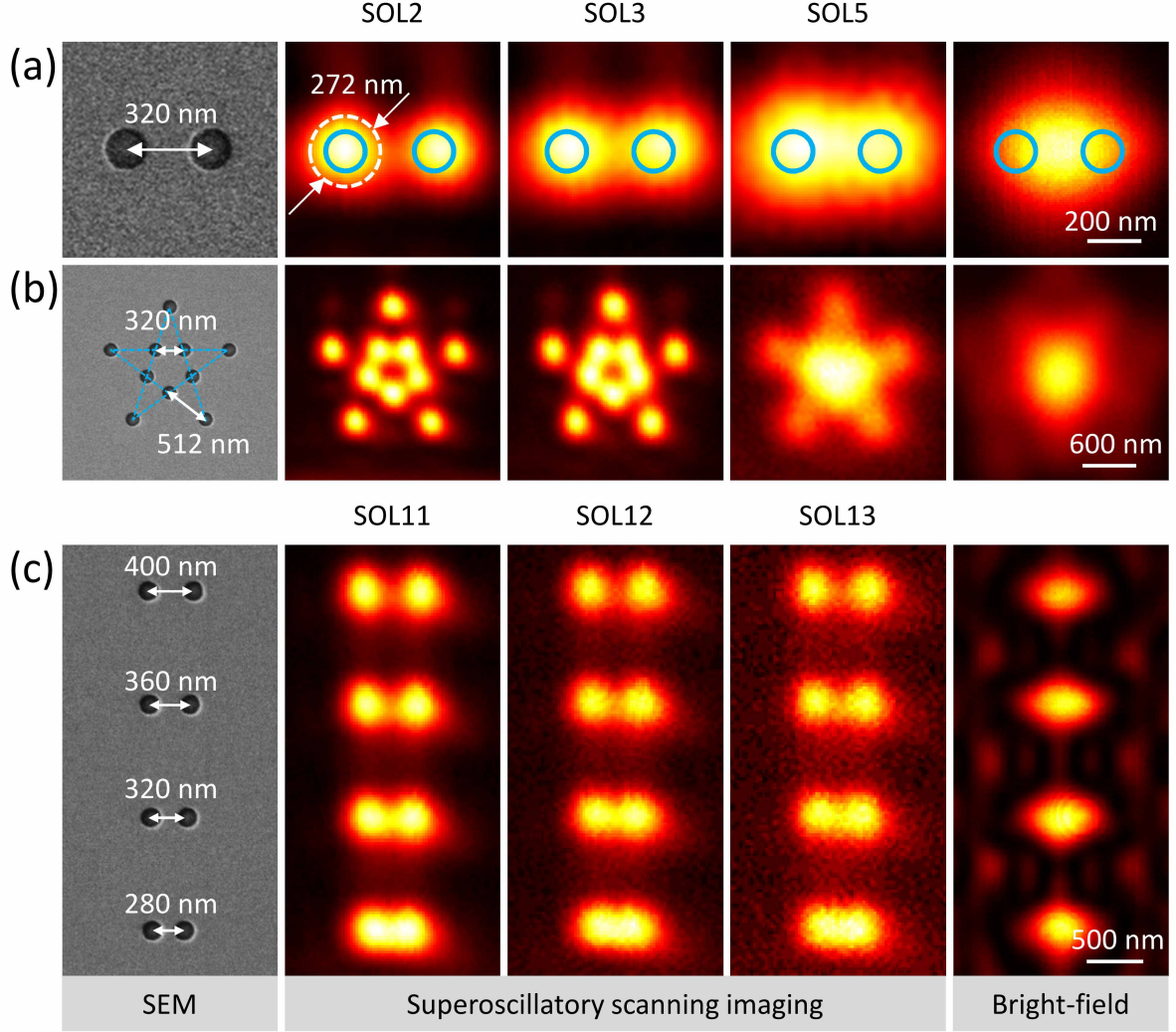
FIG. 5. Imaging with metamaterial superlenses at the wavelength of \lambda=800 nm. The first column shows SEM images of the test samples: (a) a pair of holes with diameter of 160 nm and center-to-center separation of 320 nm ( 0.4\lambda ), (b) a star-shaped constellation of holes, each with 160 nm diameter; (c) Pairs of holes with diameter of 160 nm with separations of 400 nm ( 0.5\lambda ), 360 nm ( 0.45\lambda ), 320 nm ( 0.4\lambda ) and 280 nm ( 0.35\lambda ). Rows (a-b) shows imaging results with superoscillatory illumination using metamaterial superlenses with different hotspot sizes of D_N = 0.33\lambda (SOL2), 0.39\lambda (SOL3), 0.56\lambda (SOL5) and identical field of view \Delta_N = 1\lambda . Row (c) show imaging results with superoscillatory illumination using metamaterial superlenses with different fields of view \Delta_N = 2\lambda (SOL11), 4\lambda (SOL12), 6\lambda (SOL13) and identical hotspot size of D_N = 0.39\lambda .
