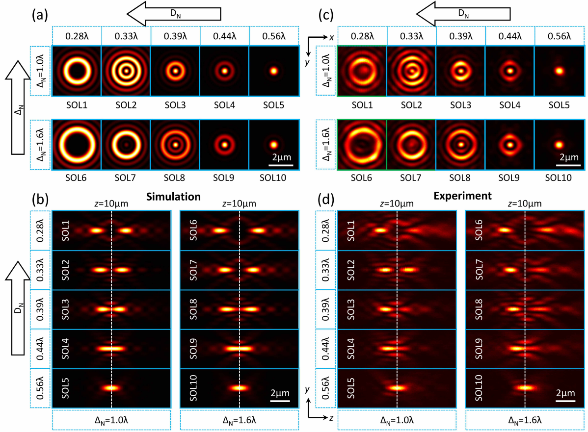
FIG. 3. Simulated intensity profiles in the (a) transverse ( z = 12.5\lambda ) and longitudinal (b) planes produced by coherent light diffraction of an ideal superoscillatory mask generator. Corresponding experimentally recorded intensity profiles in the transverse (c) and longitudinal (d) planes generated by the metamaterial superlens (see Figure 2) illuminated with a coherent laser source at \lambda = 800 nm.
