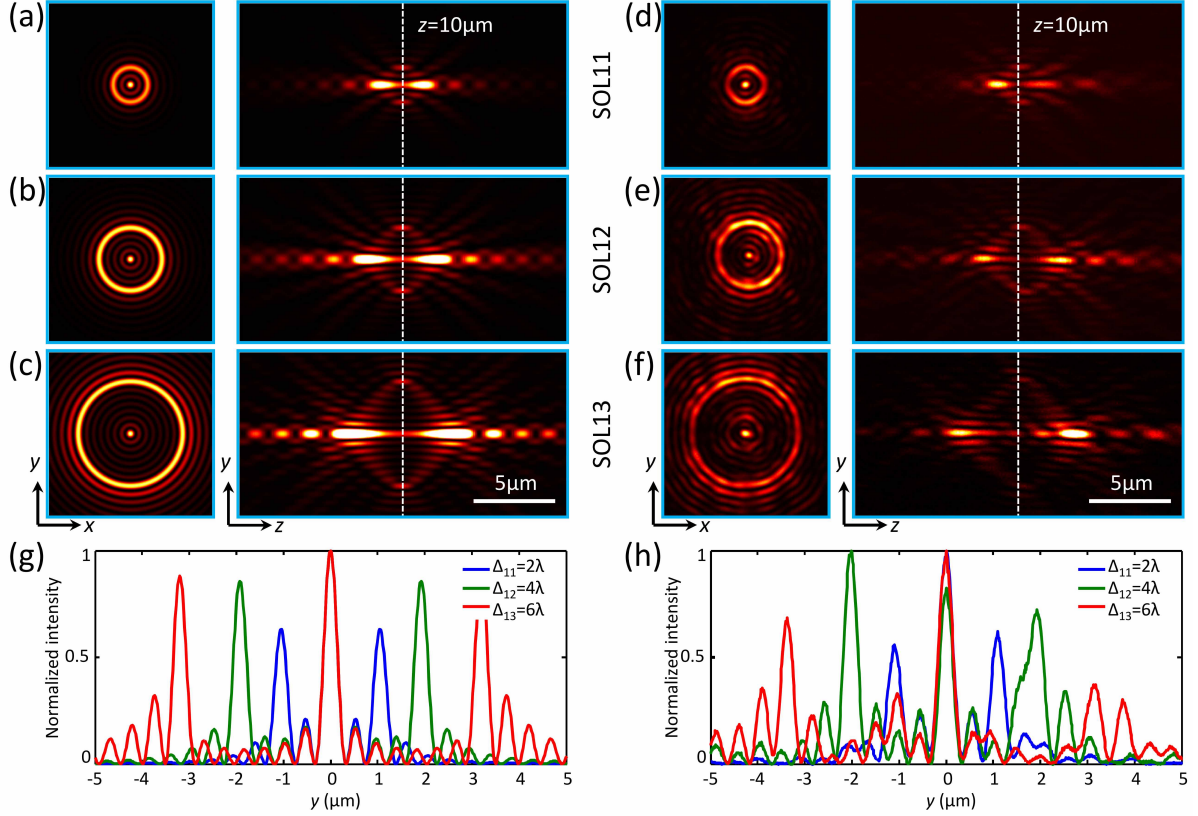
FIG. 4. Simulated superoscillatory spot cross-sections for D_N = 0.39\lambda and varying \Delta_N = 2\lambda (a), 4\lambda (b) and 6\lambda (c) in the transverse and longitudinal planes of the lens. Corresponding experimentally recorded intensity profiles (d-f) in the transverse and longitudinal planes generated by the metamaterial superlens illuminated with a coherent laser source at \lambda = 800\text{ nm} . g,h, Normalized line-scan intensity profiles at the focal plane z=10\mu\text{m} (indicated by vertical dashed lines): simulation (g) and experiment (h).
