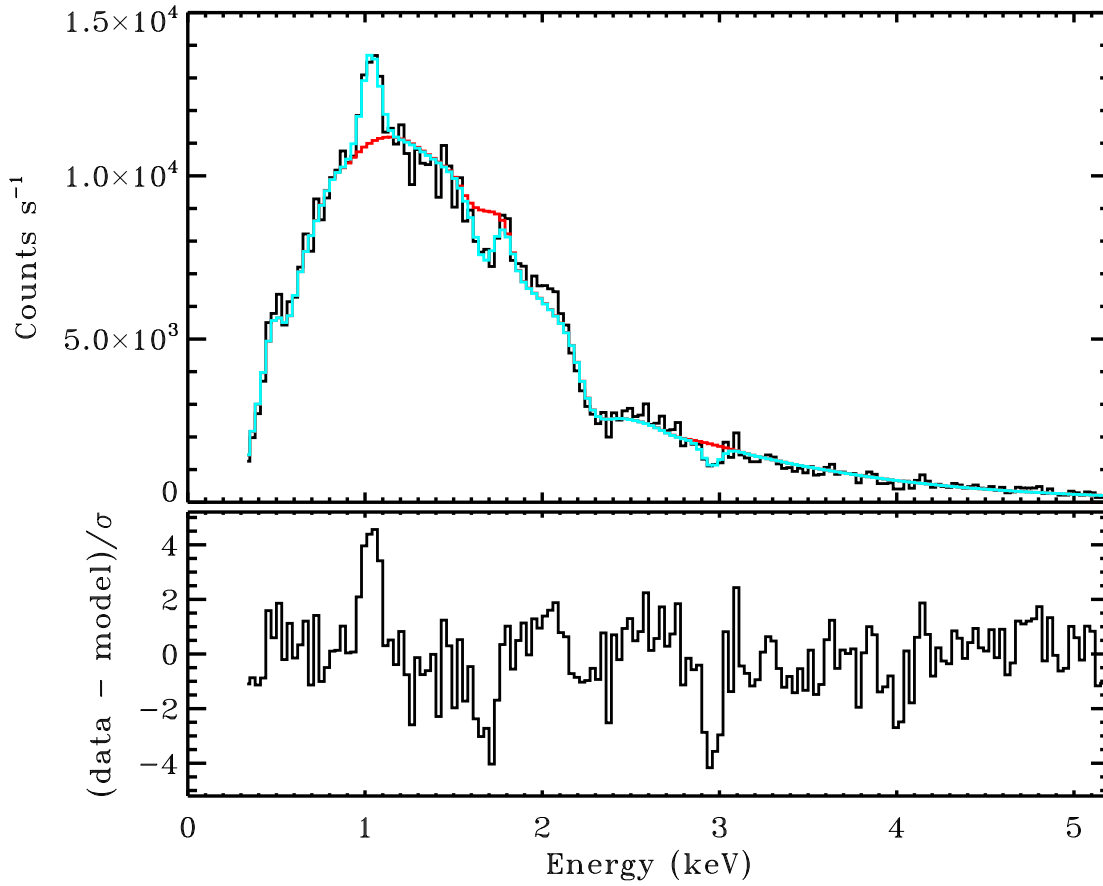
Figure 4. Co-added count rate spectrum of the PRE phases of bursts 1 and 3 (burst pair 1). The top panel shows the observed count rate as a function of energy. The red curve is the best fitting continuum model, and the cyan curve is the best fitting model including the continuum and three, narrow gaussian line components at 1, 1.7, and 3 keV. The fit residuals, in units of (\text{data} - \text{model})/\sigma , for the best fitting model with the line normalizations set to zero, are shown in the bottom panel. The excess emission is clearly evident near 1 keV, and a pair of absorption lines are indicated near 1.7 and 3 keV. See §2.3 for additional details.
