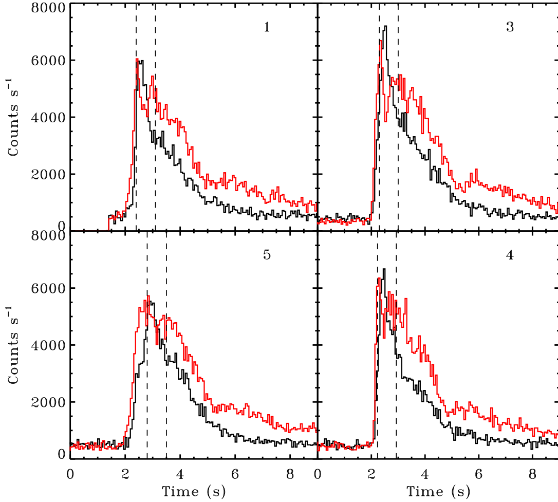
Figure 1. Light curves of four PRE X-ray bursts from 4U 1820 observed with NICER . Count rates computed in 1/16 s intervals in the 0.2 - 1.0 keV (black) and 2.0 - 10.0 keV (red) bands are shown. The vertical dotted lines mark the intervals used to extract PRE-phase spectra. Clockwise from upper left, the four panels correspond to bursts 1, 3, 4, and 5 (see Table 1).
