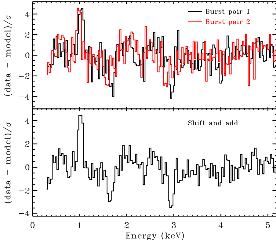
Figure 8. Fit residuals for both burst pairs 1 (black) and 2 (red) are shown in units of (\text{data} - \text{model})/\sigma (top). Here, the plotted residuals were obtained from the best-fitting model after setting the fitted line normalizations to zero. Also shown are the average (“shift and add”) residuals when the burst pair 2 spectrum is shifted in energy by the best fitting constant line ratio of 1.046 and averaged (see Figure 7 and §2.4).
