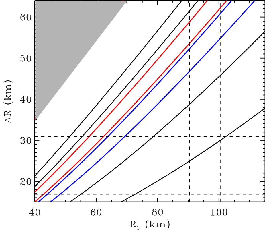
Figure 9. Contours of constant gravitational red-shift, expressed as an observed energy ratio, E_1/E_2 , are plotted versus R_1 and \Delta R = R_1 - R_2 . Here, R_1 and R_2 ( R_1 > R_2 ) are two radial sites of photon emission with the same rest-frame energy. Contours of constant line ratio consistent with our measured value of 1.046 \pm 0.006 are shown for neutron star masses of 1.5 (red) and 2.0 (blue) M_\odot . From bottom to top the black curves correspond to line ratios of 1.01, 1.02, 1.06, and 1.08 (for a neutron star mass of 1.5 M_\odot ). Ignore the grey shaded region as values were not computed there. The vertical and horizontal dashed lines mark representative ranges of the photospheric radii R_1 and \Delta R derived from co-added spectra of burst pairs 1 and 2 (see §2.3).
