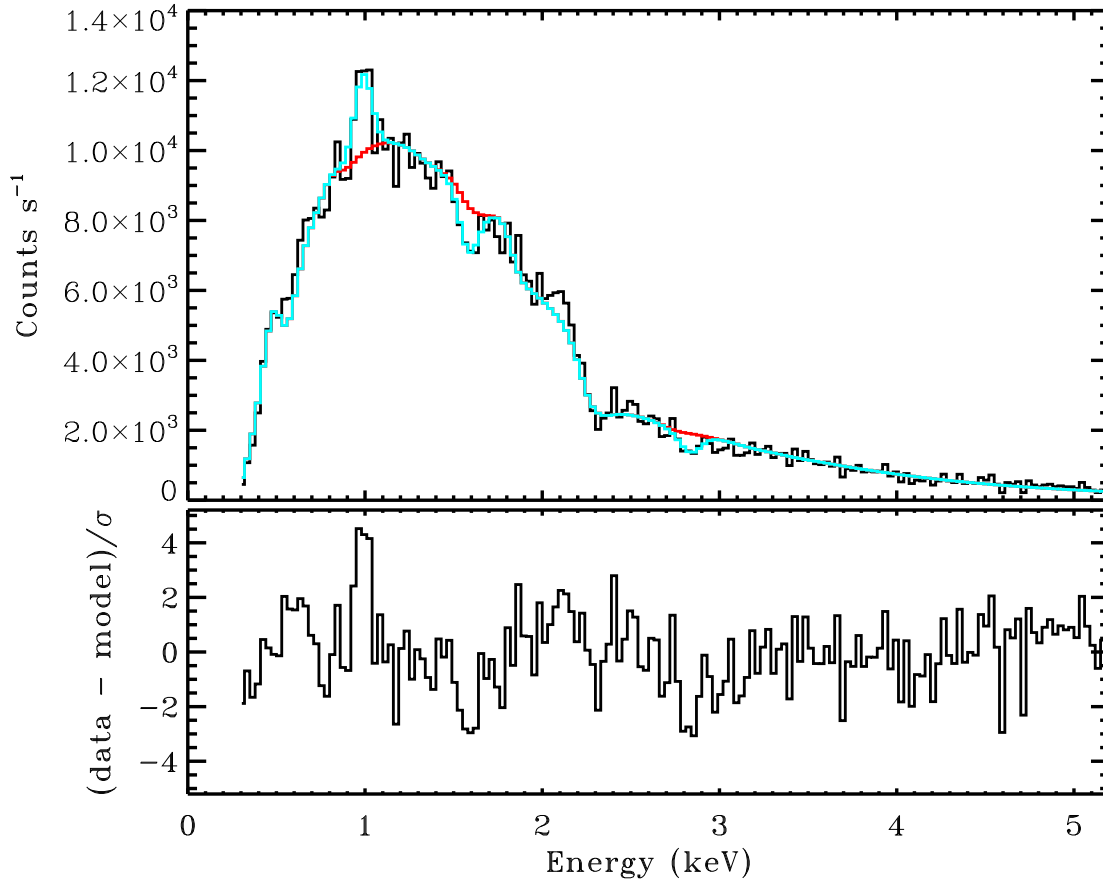
Figure 5. Co-added count rate spectrum of the PRE phases of bursts 4 and 5 (burst pair 2). Other details are the same as in Figure 4. Features similar to those evident in burst pair 1 (Figure 4) are also apparent in this spectrum. See §2.3 for further details.
