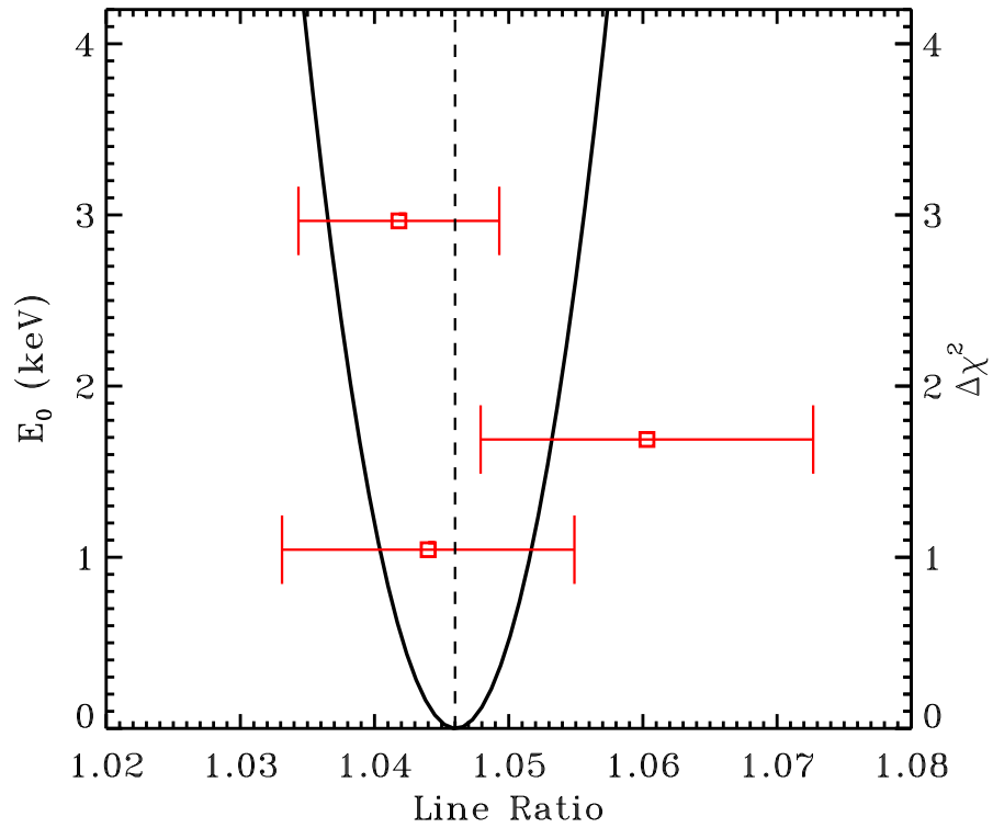
Figure 7. Measured line energy ratios and uncertainties of the 1, 1.7 and 3 keV line features obtained from burst pairs 1 and 2 (red symbols). Also shown on the right vertical axis are the \Delta\chi^2 values for a single parameter, constant line ratio fit (solid black curve). The best fitting value of the line energy ratio, s_0 = 1.046 \pm 0.006 ( 1\sigma , \Delta\chi^2 = 1 ) is marked by the vertical dashed line. A constant ratio is a good statistical description of the three observed line energy ratios.
