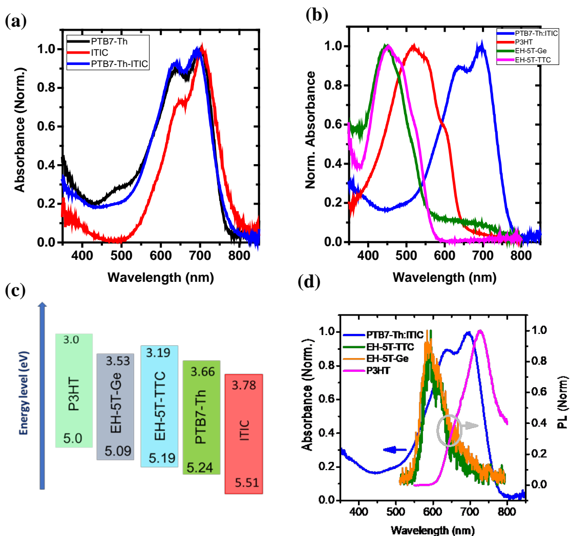
Figure 3. (a) UV-Vis absorption spectrum of the PTB7-Th:ITIC binary blend system and spectra of the individual components; (b) complementary UV-Vis absorption properties of the ternary component donor molecules and the binary PTB7-Th:ITIC blend; (c) energy level diagram of the PTB7-Th:ITIC blend with its ternary donor components; (d) PL spectra of the ternary donor components and the absorption spectra of the binary blend film.
