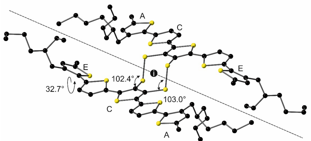
Figure 1. Molecular structure of EH-5T-TTC with hydrogens omitted for clarity. The inversion centre of the asymmetric unit is marked with the letter i.
