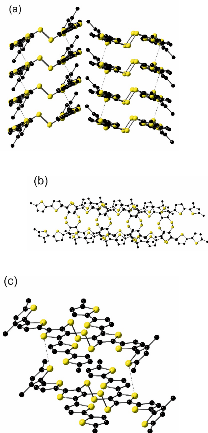
Figure 2. Packing diagrams of EH-5T-TTC with the ethylhexyl chains truncated for ease of viewing. The dashed lines represent S \cdots S close contacts.
