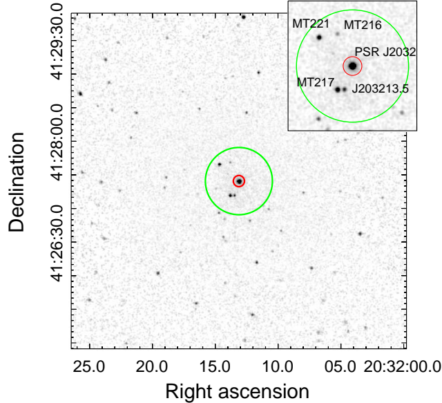
Figure 2. Exposure-corrected Chandra X-ray image of the field centered on J2032 in 0.5–7 keV range, lightly smoothed to 2'' resolution. The red and green circles have radii of 5'' and 30'' radius that indicate the extraction regions for Chandra and XMM-Newton spectral analysis, respectively. Inset: zoom-in of the image showing four nearby background sources: MT91 221, MT91 216, MT91 217, and CXOU J203213.5+412711 (see Appendix A).
