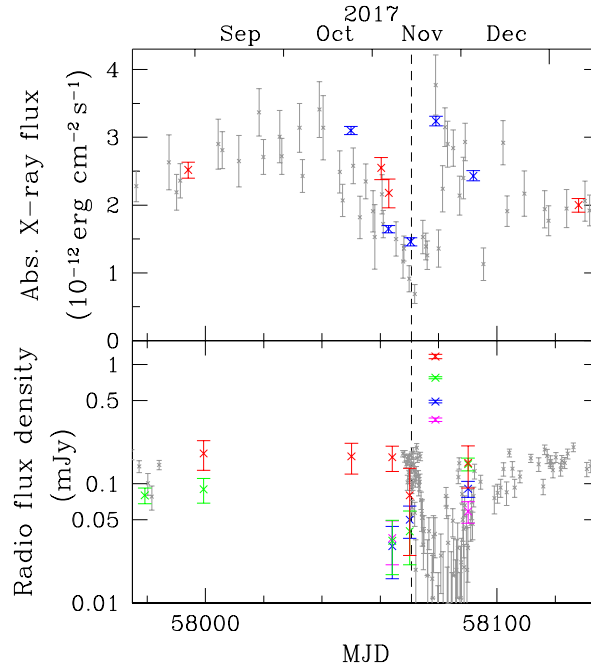
Figure 5. Top: X-ray flux of J2032 as in Fig. 3 (red: Chandra ; blue: XMM-Newton+NuSTAR ) compared with the Swift light curve (grey) around periastron. All these are absorbed flux in 0.5–8 keV range. Bottom: radio flux densities of J2032 over the same period. The VLA detections at the L, S, C, and X bands are shown in red, green, blue, and magenta, respectively. The grey data points indicate the pulsed flux density at the L band for comparison (Stappers et al. in prep.). The vertical dashed line marks the date of periastron passage.
