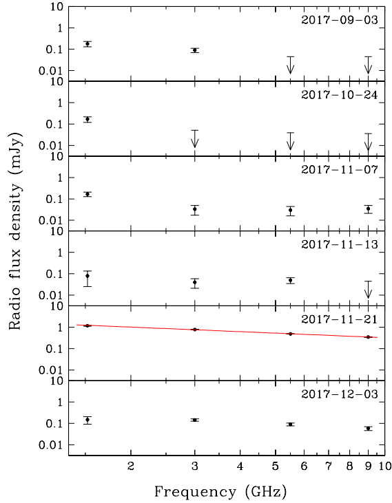
Figure 6. Radio spectrum of J2032 at different epochs measured with the VLA. In cases of non-detection, 3\sigma upper limits are plotted. The line shows the best-fit spectrum of S_\nu \propto \nu^{-0.71} when the emission was brightest.
