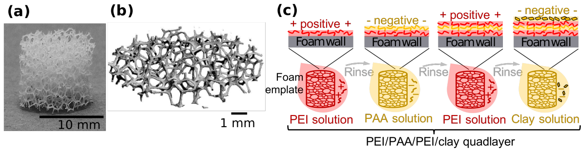
Figure 1. (a) PU foam template, (b) volumetric reconstruction of a 1 mm tall cross-section from a PU foam template, (c) LbL assembly sequence for depositing a single PEI/PAA/PEI/nanoclay QL onto a foam template, with schematics (top) depicting the coating multilayer structure.
