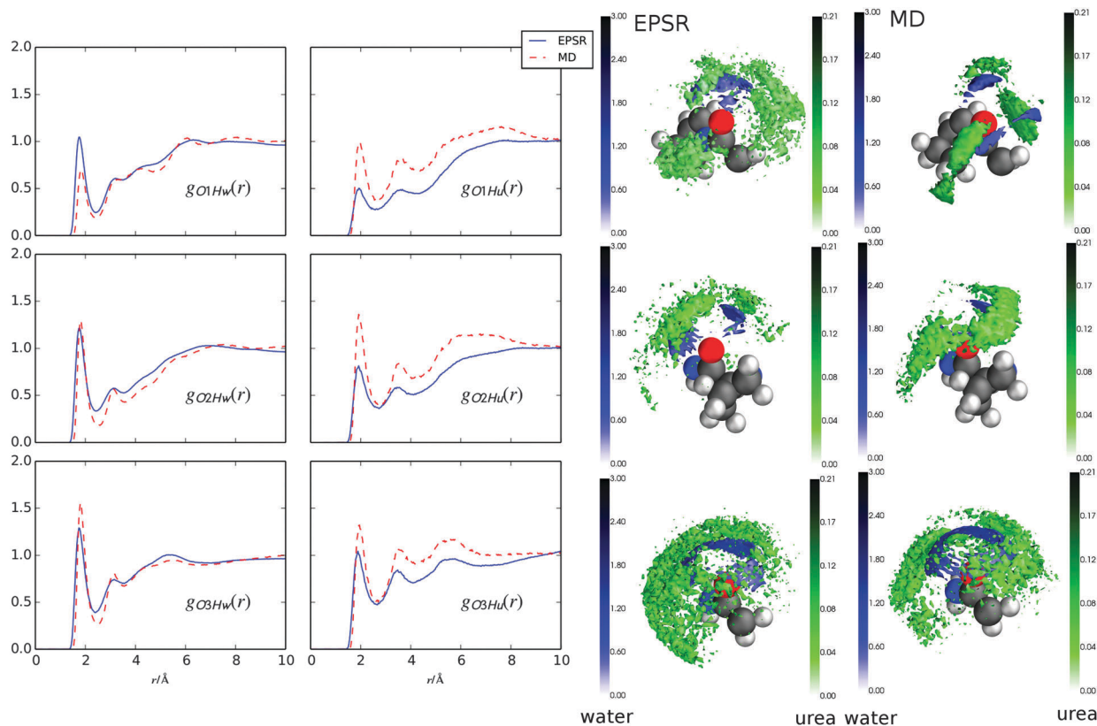
Fig. 4 Left column: radial distribution functions ( g(r) s) for GPG peptide bond carbonyl oxygens and H_w/H_u atoms from water and urea. Middle column: spatial density maps (SDMs) of O_w (blue clouds) and Cu (green clouds) around O1, O2 and O3 from EPSR. Right column: SDMs for water and urea around O1, O2 and O3 from MD. The 3D shells show the top 20% of all molecules in a distance range from 0–3.3 Å for water and 0–5 Å for urea around GPG oxygens on the central axis.
