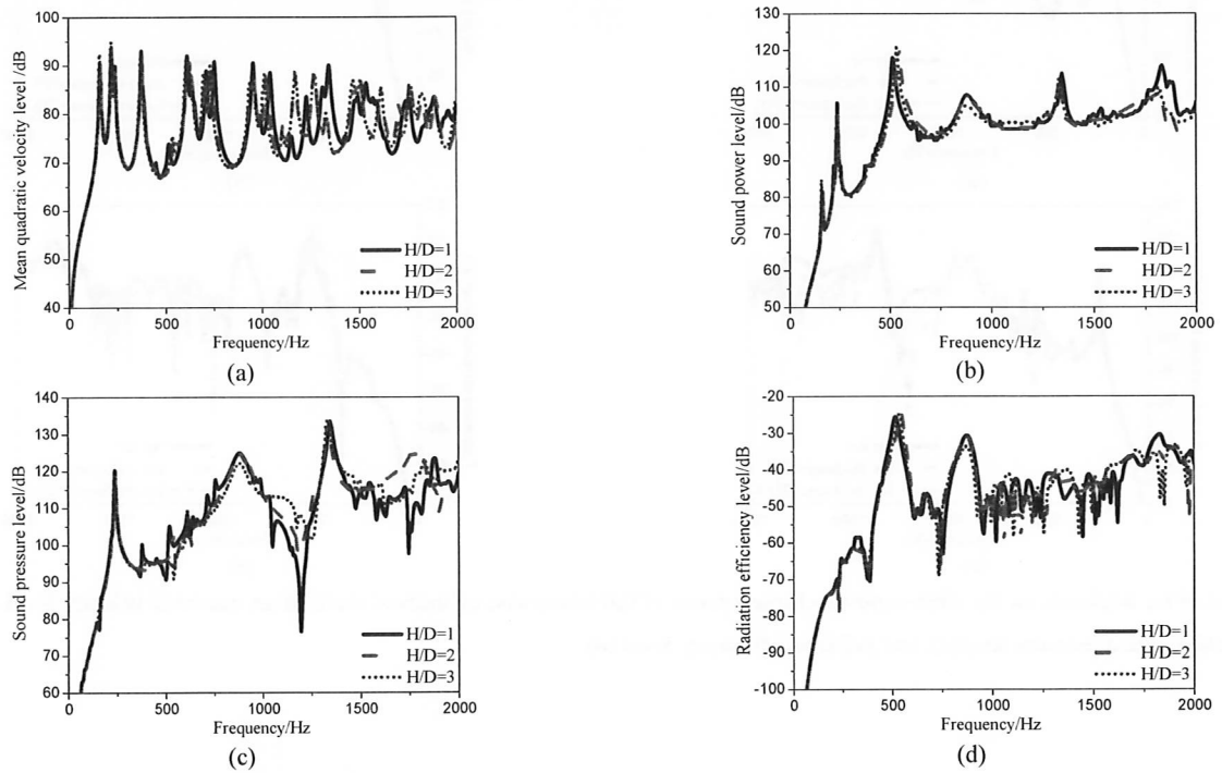
Fig.6 Effect of H/D on the vibro-acoustic characteristics of full immersion cylindrical shell. Mean quadratic velocity level (a), sound power level(b), sound pressure level(c), and radiation efficiency level (d).
