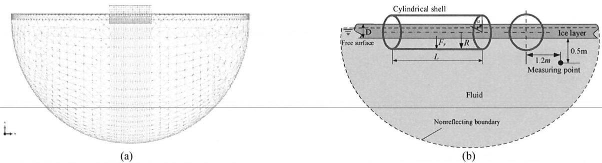
Fig.8 Schematic diagram of semi-submersible model. Finite element model (a), and illustration of partially immersed model (b).
