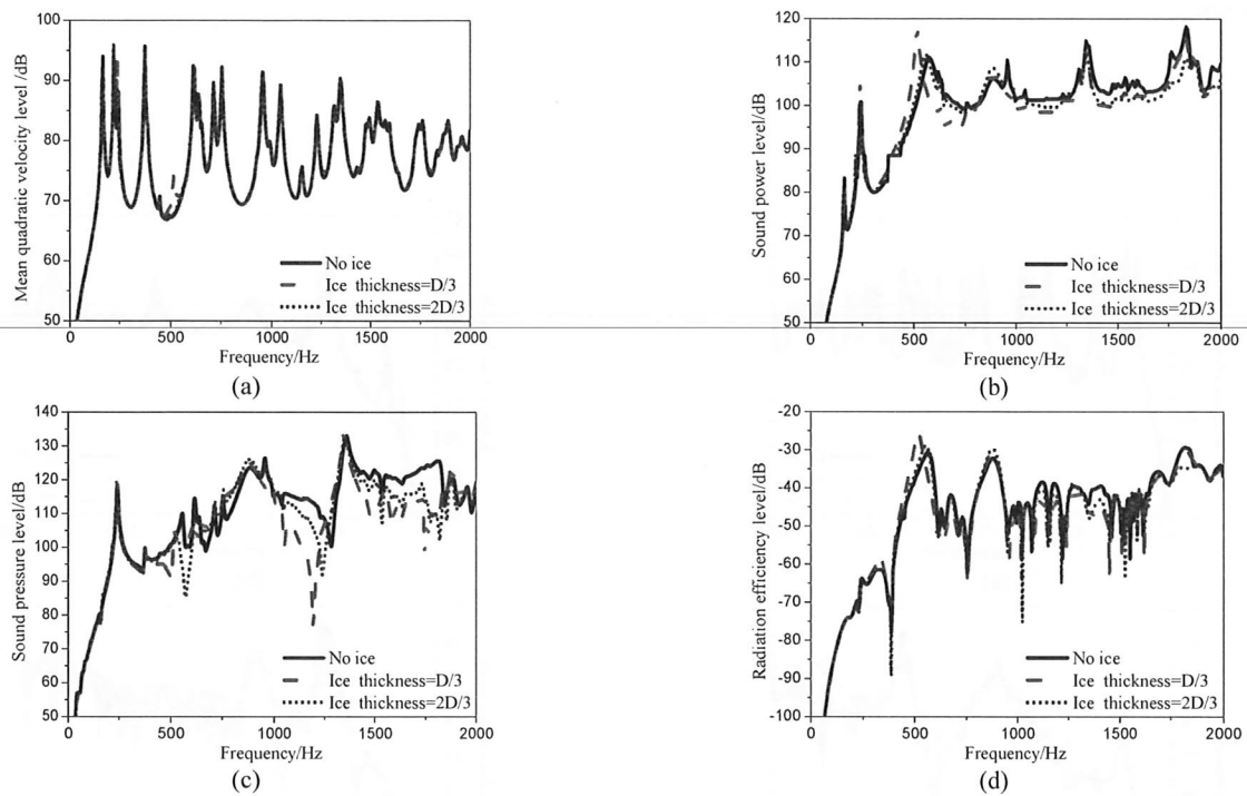
Fig.4 Effect of ice thickness on the vibro-acoustic characteristics of full immersion cylindrical shell. Mean quadratic velocity level (a), sound power level(b), sound pressure level(c), and radiation efficiency level (d).
