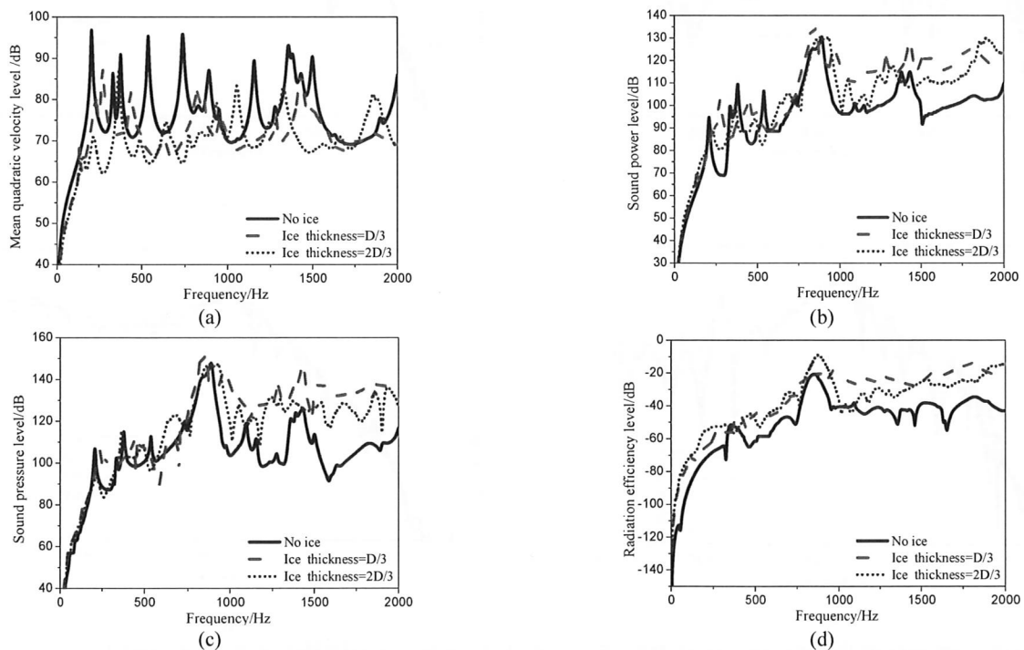
Fig.9 Influence of ice thickness on the vibro-acoustic characteristics of semi-submerged cylindrical shell. Mean quadratic velocity level (a), sound power level(b), sound pressure level(c), and radiation efficiency level (d).
