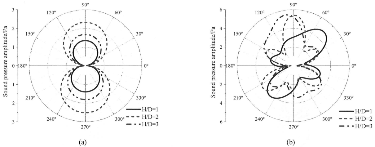
Fig.7 Influence of H/D on the sound directivity of full immersion cylindrical shell. Sound directivity at 600 Hz (a), and sound directivity at 1800 Hz (b).
