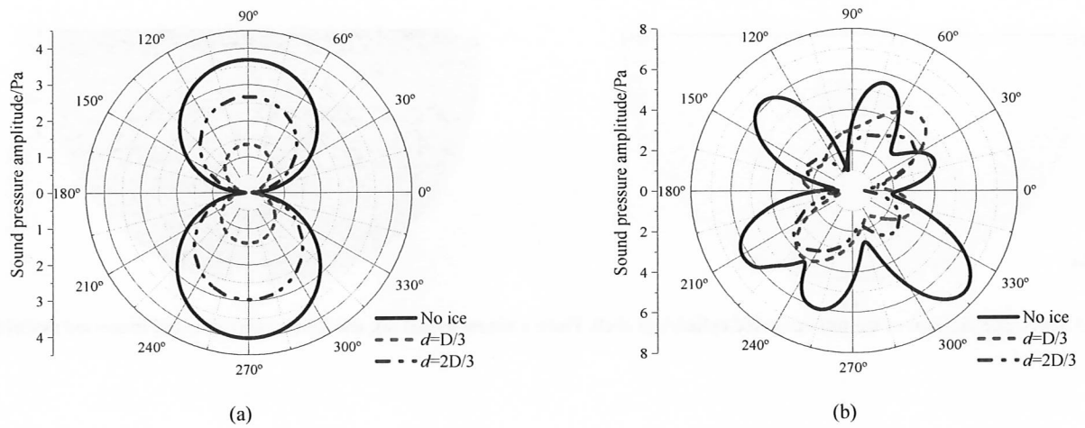
Fig.5 Effect of ice thickness on the sound directivity of full immersion cylindrical shell. Sound directivity at 600 Hz (a), and sound directivity at 1800 Hz (b).
