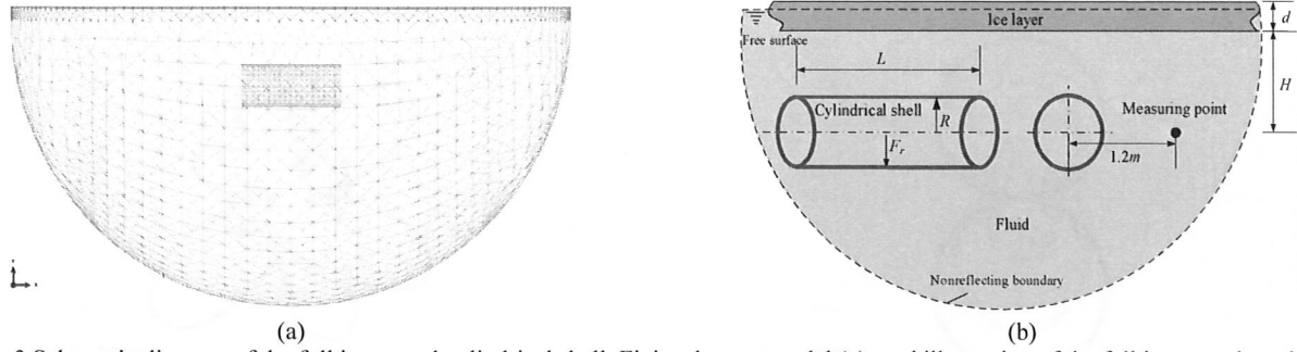
Fig.3 Schematic diagram of the full immersed cylindrical shell. Finite element model (a), and illustration of the full immersed model (b).
