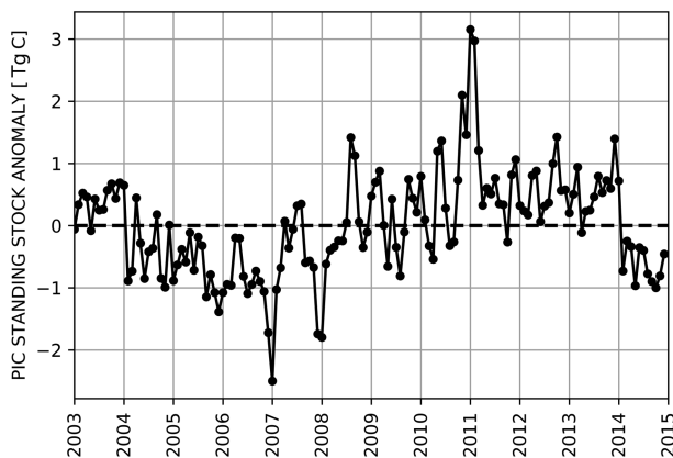
Figure 5. Interannual variability in average monthly global PIC standing stock integrated over the top 100 m of the water column (Tg PIC). Data represent anomalies from the annual climatology of PIC standing stock. PIC = particulate inorganic carbon.
