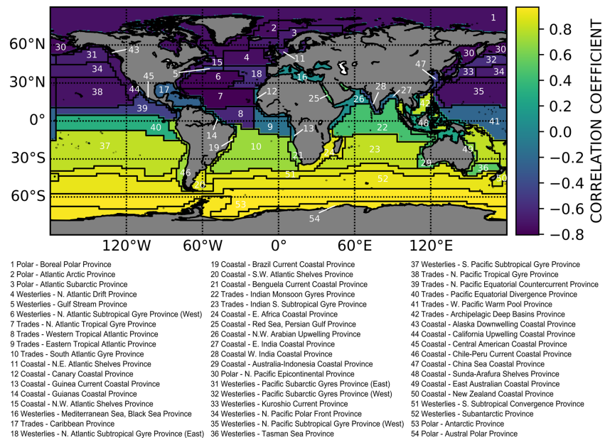
Figure 3. Correlation of province PIC standing stock time series with global PIC standing stock time series (Figure 2). Green to yellow represents a positive correlation coefficient, while green to blue indicates a negative correlation coefficient. Provinces with no color are where correlation is not significant at the 5% level. PIC = particulate inorganic carbon.
