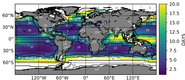
Figure 7. Spatial variability in PIC standing stock turnover times, calculated by dividing the integrated PIC standing stock by the integrated calcite production rate estimated according to Hopkins and Balch (2018). See Figure 3 for key to Longhurst (1998) province numbers. White areas represent regions where turnover times are >20 days or areas of no data due to low winter sun angle, water depth < 200 m, persistent cloud or ice cover. PIC = particulate inorganic carbon.
