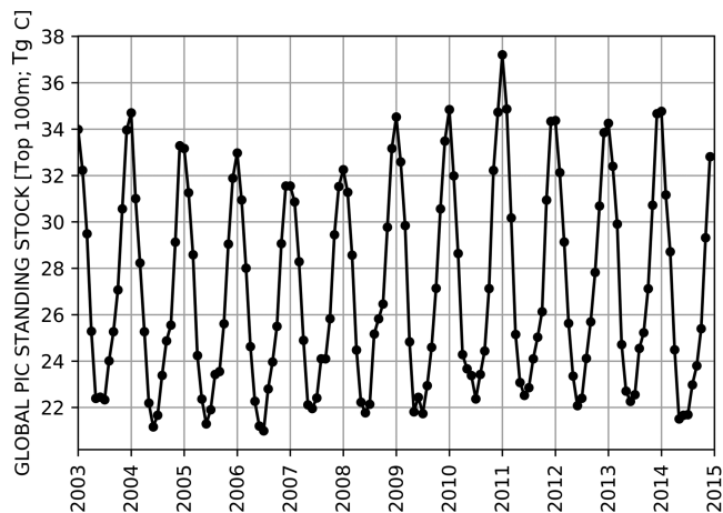
Figure 2. Globally integrated, monthly PIC standing stock time series (in teragrams of PIC). PIC = particulate inorganic carbon.
