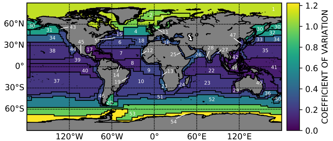
Figure 4. Temporal variability in Longhurst (1998) province particulate inorganic carbon standing stock as measured by the coefficient of variability (standard deviation/mean). Yellow indicates high variability within the seasonal time series, while blue indicates low variability. Numbers refer to the Longhurst (1998) provinces. See Figure 3 for key to province numbers.
