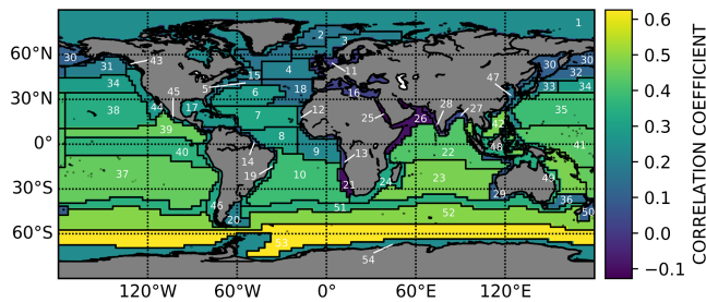
Figure 6. Correlation of province PIC 100-m-integrated standing stock anomalies with global PIC standing stock anomalies (Figure 5). Yellow represents relatively high correlation coefficient and blue a relatively low correlation coefficient. Provinces with no color are where correlation is not significant at the 5% level. See Figure 3 for key to province numbers. PIC = particulate inorganic carbon.
