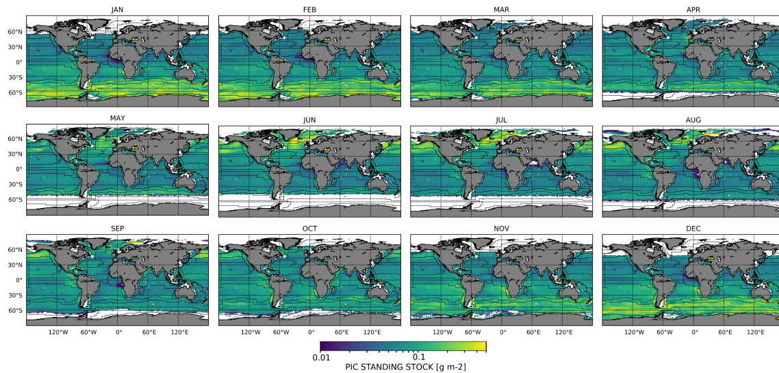
Figure 1. Average, monthly global PIC standing stocks derived from AQUA Moderate Resolution Imaging Spectroradiometer PIC concentration data (2003–2014) integrated to 100 m ( \text{g}/\text{m}^2 ). Black lines indicate Longhurst provinces (Longhurst, 1998). White areas represent regions of no data due to low winter Sun angle, water depth <200 m, persistent cloud or ice cover. PIC = particulate inorganic carbon.
