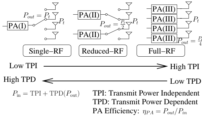
FIGURE 17: The tradeoff between single-RF, reduced-RF and full-RF schemes from the PA's perspective.
