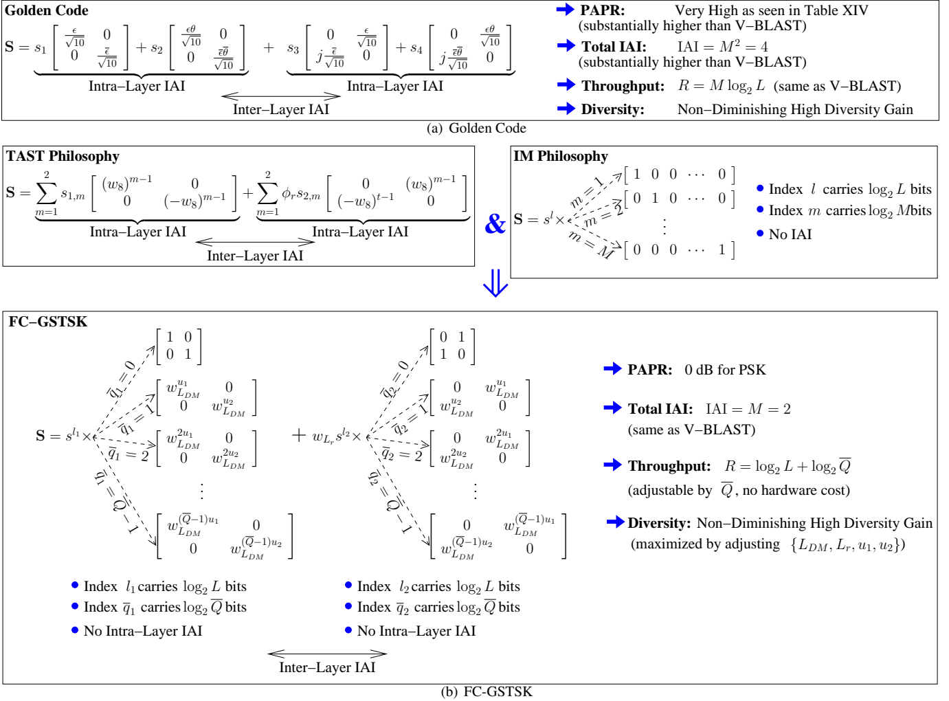
FIGURE 31: Schematic descriptions of Golden code [239] and the recently developed FC-GSTSK [137], where M = 2 TAs are used. The parameters for Golden code are the fixed \theta = \frac{1+\sqrt{5}}{2} , \epsilon = 1 + j - j\theta , \bar{\theta} = \frac{1-\sqrt{5}}{2} and \bar{\epsilon} = 1 + j - j\bar{\theta} . The parameters for FC-GSTSK are the adjustable \{L_{DM}, L_r, u_1, u_2\} , while the indices \{l_1, l_2, \bar{q}_1, \bar{q}_2\} carries source information. The notations are w_{L_{DM}} = \exp(j\frac{2\pi}{L_{DM}}) and \phi_r = w_{L_r} = \exp(j\frac{2\pi}{L_r}) .
