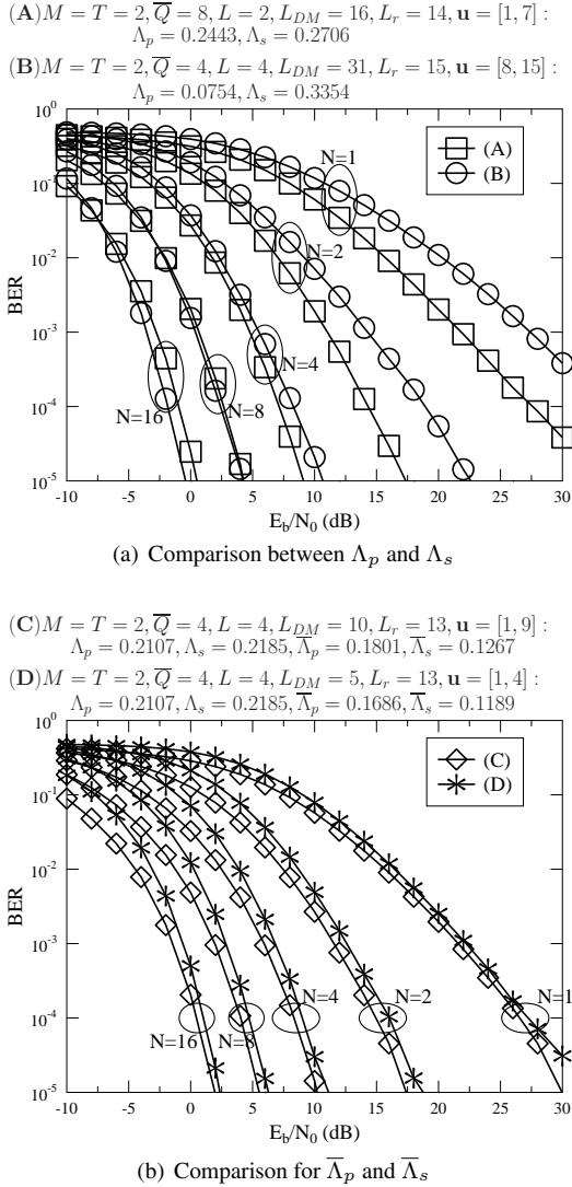
FIGURE 40: Performance comparison between four FC-GSTSK( M = T = 2, R = 4 ) associated with different parameters (adapted from [137]).
