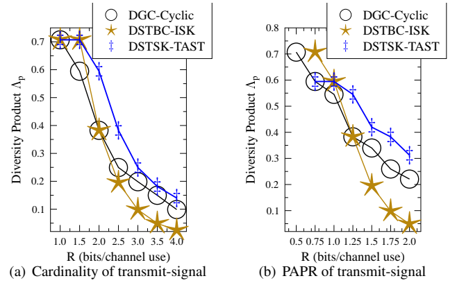
FIGURE 21: Comparison of diversity products of finite-cardinality DSTM schemes.
