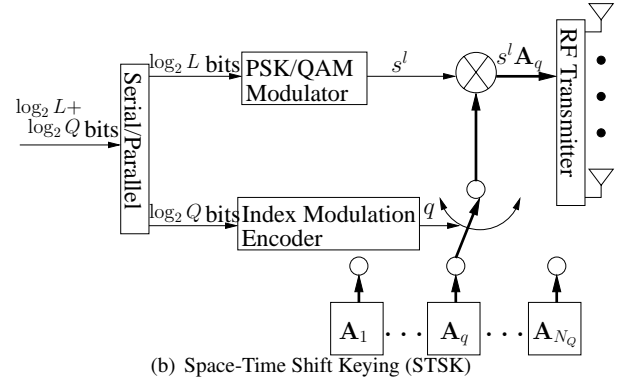
FIGURE 16: Schematics of Spatial Modulation (SM) and Space-Time Shift Keying (STSK).
