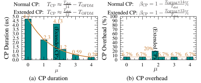
FIGURE 6: The scalable numerology on Cycle Prefix (CP) with respect to (a) CP duration; (b) CP overhead.
