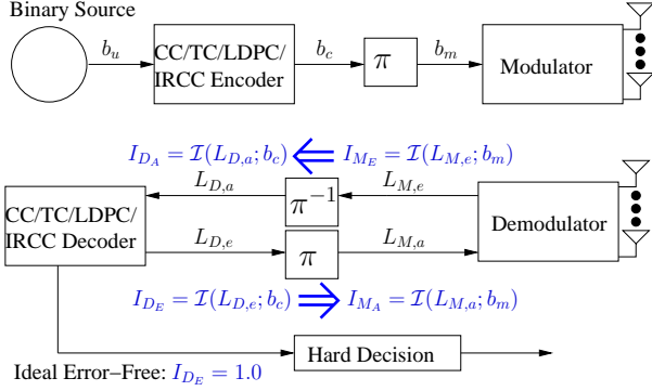
FIGURE 33: Schematic of channel coding aided modulation scheme and its two-stage turbo decoder. The channel coding arrangements include Convolutional Code (CC) of IEEE 802.11 family, Turbo Code (TC) of 4G LTE, Low-Density Parity-Check (LDPC) code of 5G NR and IrRegular Convolutional Code (IRCC) for the next-generation network.
