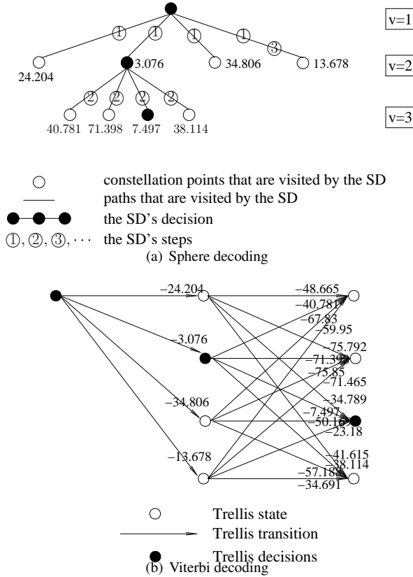
FIGURE 12: Example of Multiple-Symbol Differential Sphere Detection (MSDSD) conceived for DQPSK recorded at SNR=10 dB, where we have N_w = 3 , and its corresponding trellis decoding aided MSDD using the Viterbi algorithm.
