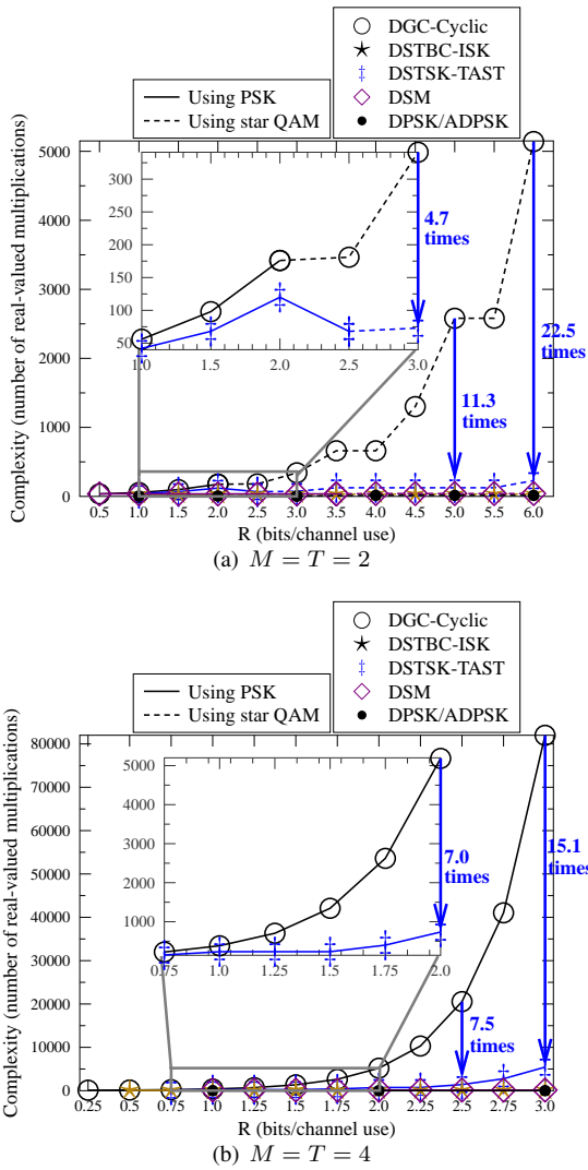
FIGURE 22: Complexity comparison for finite-cardinality DSTM schemes associated with M = T = \{2, 4\} and N = 1 , where the DSTSK-TAST's complexity reduction compared to DGC-cyclic are marked by blue arrows.
