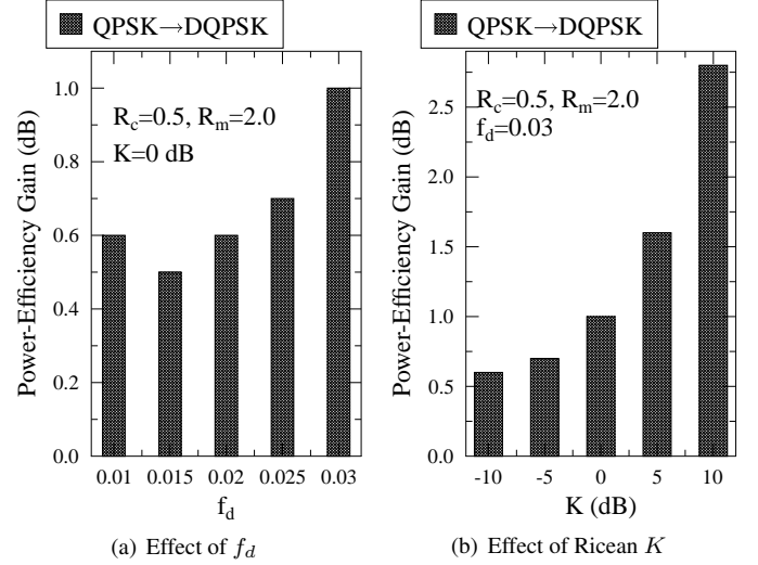
FIGURE 27: Power-Efficiency comparison of QPSK relying on pilot-based CSI estimation and DQPSK employing MSDD over Ricean fading channels, where we have R_m = 2.0 and R_c = 0.5 .
