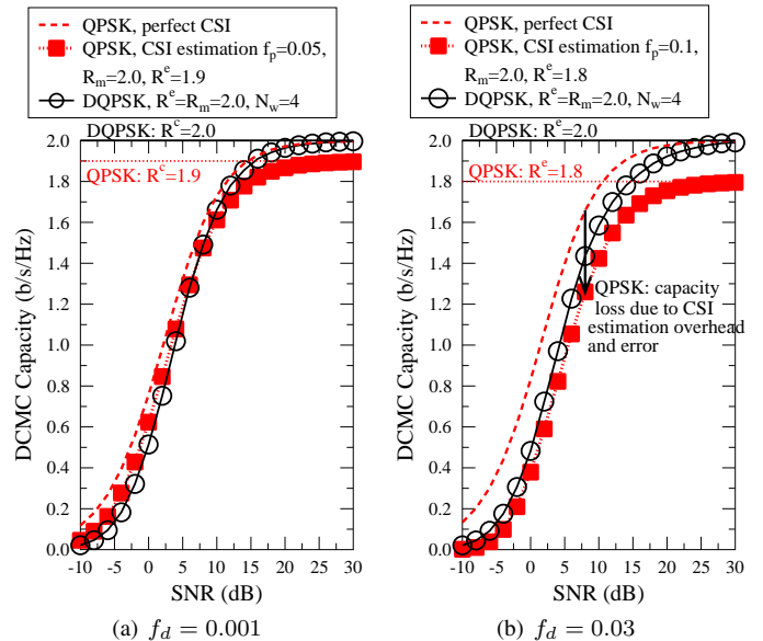
FIGURE 25: DCMC capacity comparison of QPSK relying on pilot-based CSI estimation and DQPSK employing MSD over Ricean fading channels ( K = 0 dB, f_d = \{0.001, 0.03\} ).
