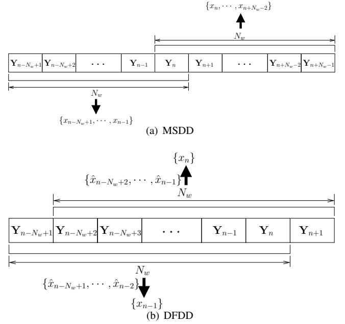
FIGURE 11: Schematics of MSDD and DFDD for non-coherent detection.
