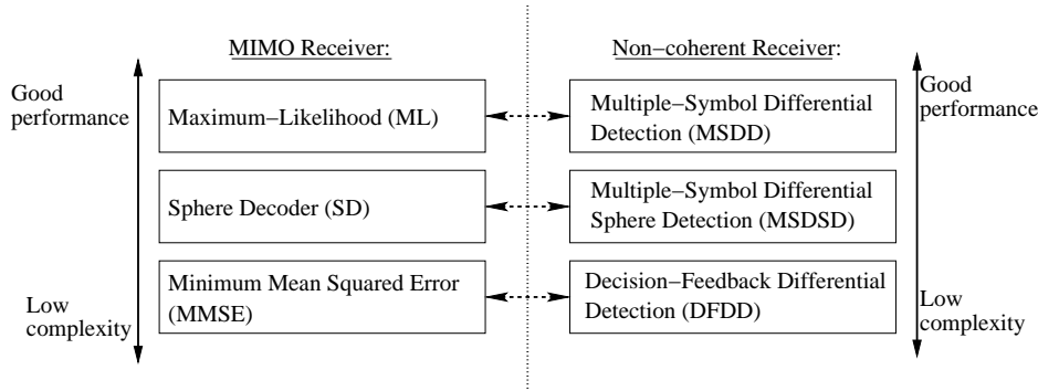
FIGURE 13: Links between generic MIMO detection schemes and generic non-coherent detection schemes.
