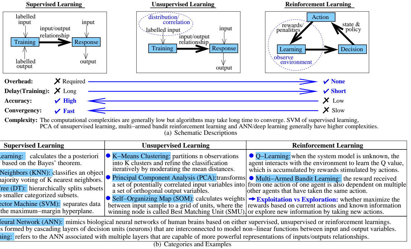
FIGURE 37: Categories, schematics, characteristics and examples of machine learning algorithms.
