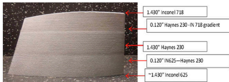
Figure 6. DED-built aerofoil comprised of various superalloys used for testing and evaluation purposes. Reproduced from [56], with the permission of Springer, 2017.
